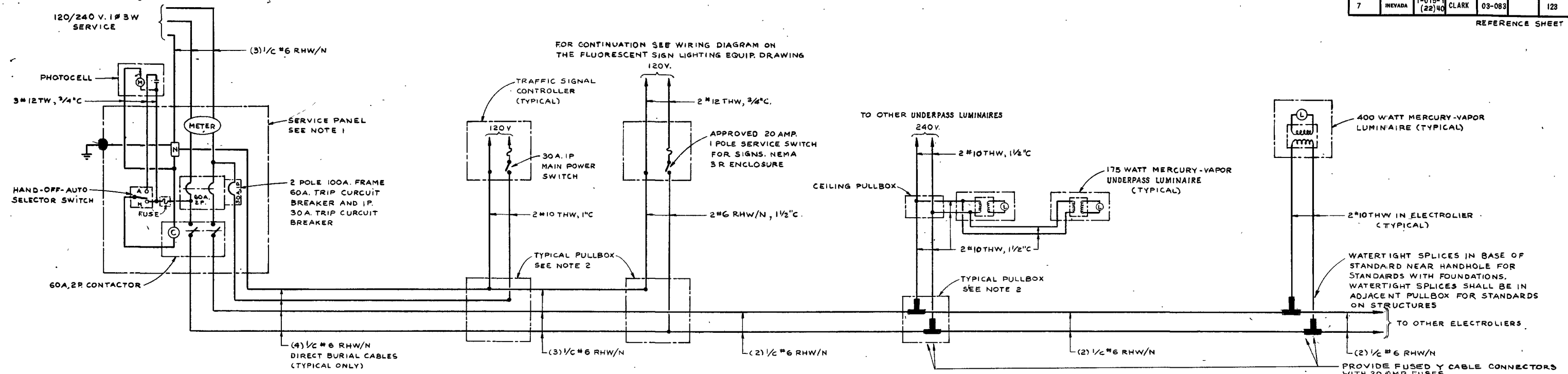
TYPICAL ELECTRICAL SERVICE AND SYSTEM WIRING DIAGRAM FOR LIGHTING AND TRAFFIC SIGNALS NO SCALE
