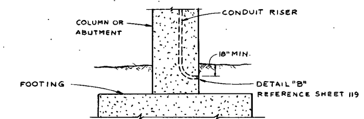
CONDUIT RISER AT COLUMN OR ABUTMENT NO SCALE
