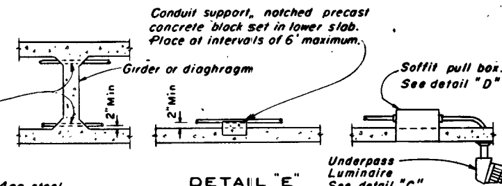
DETAIL "E" Luminaire See detail "C" CONDUIT INSTALLATION IN BOX GIRDER SECTIONS
