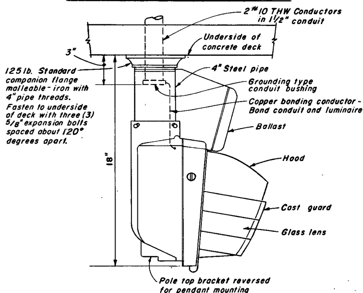
DETAIL "C" UNDERPASS LUMINAIRE
