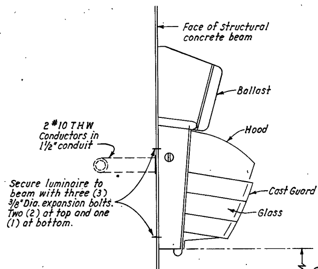
DETAIL "F" UNDERPASS LUMINAIRE
