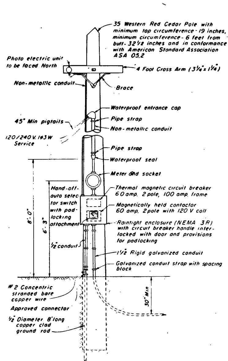
DETAIL "A" SERVICE POLE
