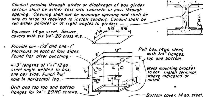
DETAIL "D" SOFFIT PULL BOX
