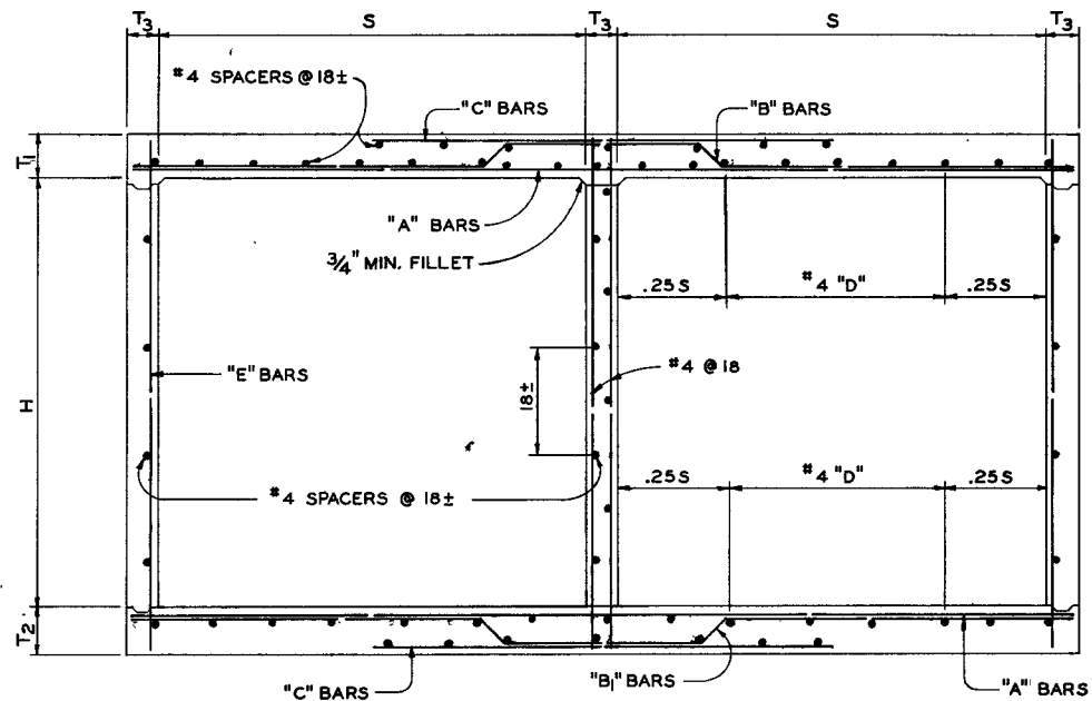
TYPICAL SECTION
