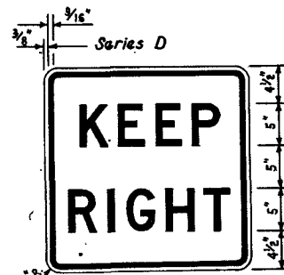
R4-7S 2'-0" x 2'-0"
