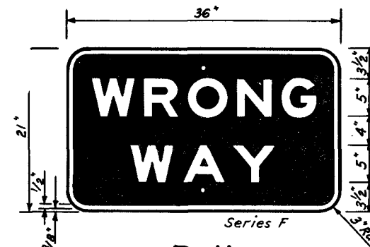
R-11 3'-0" x 1'-9"
