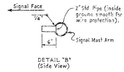
MAST ARM SIGNAL MOUNTINGS (Use Std. Plumbizer)
