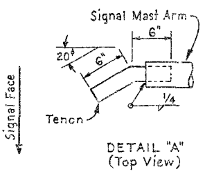
MAST ARM SIGNAL MOUNTINGS (Use Std. Plumbizer)
