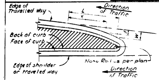
ISLAND & MISCELLANEOUS AREAS PAVING
