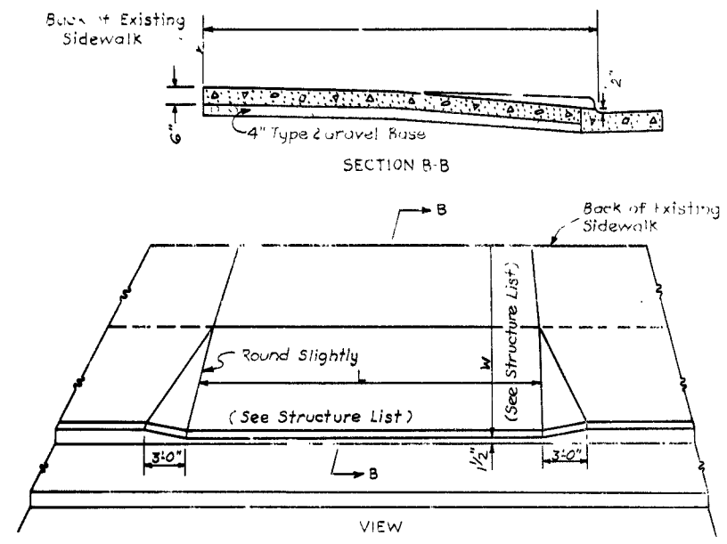
DRIVEWAY DETAIL
