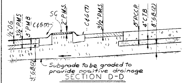
DETAIL AT FREEWAY NOSE
