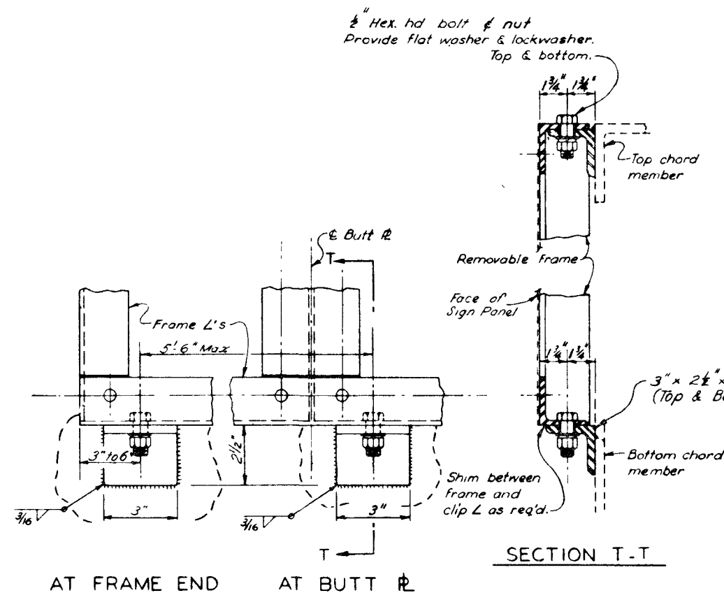
FRAME MOUNTING DETAILS
