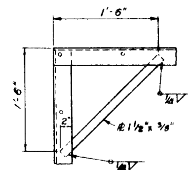
DETAIL ⑨
