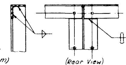
DETAIL (10)
