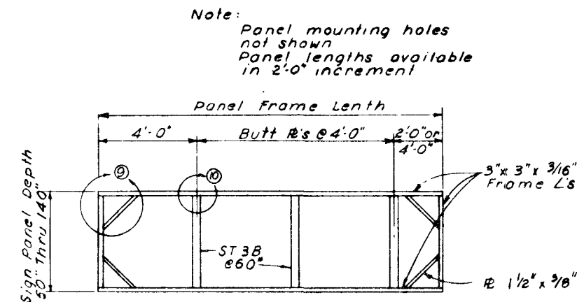
TYPICAL REMOVABLE FRAME (4'-0" thru 20'-0")
