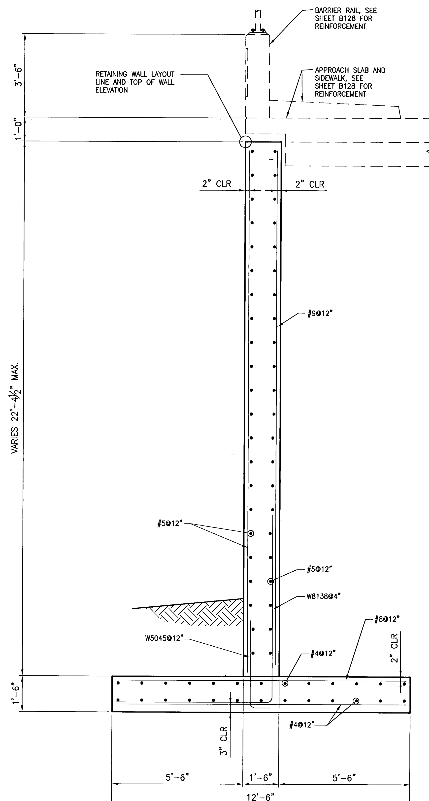
SECTION B-B
