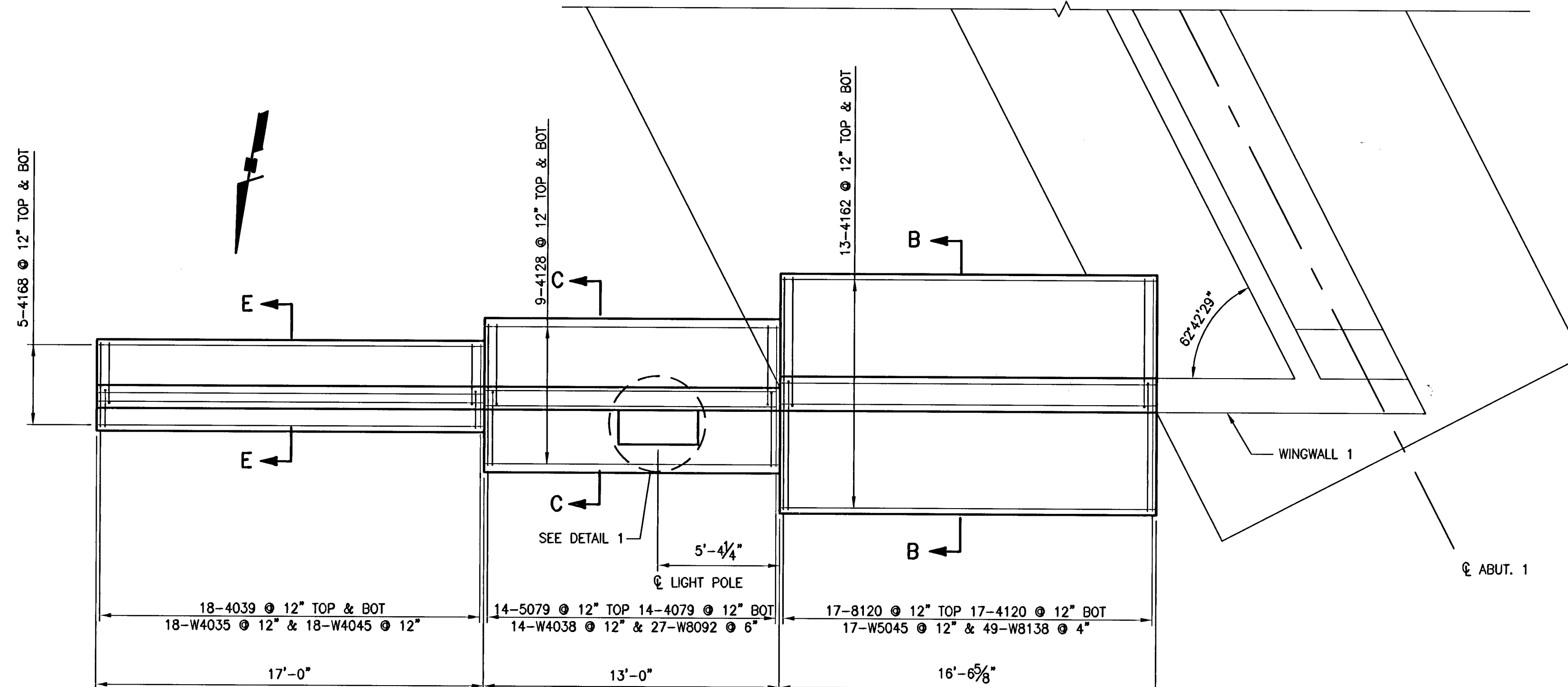
PLAN RETAINING WALL 8
