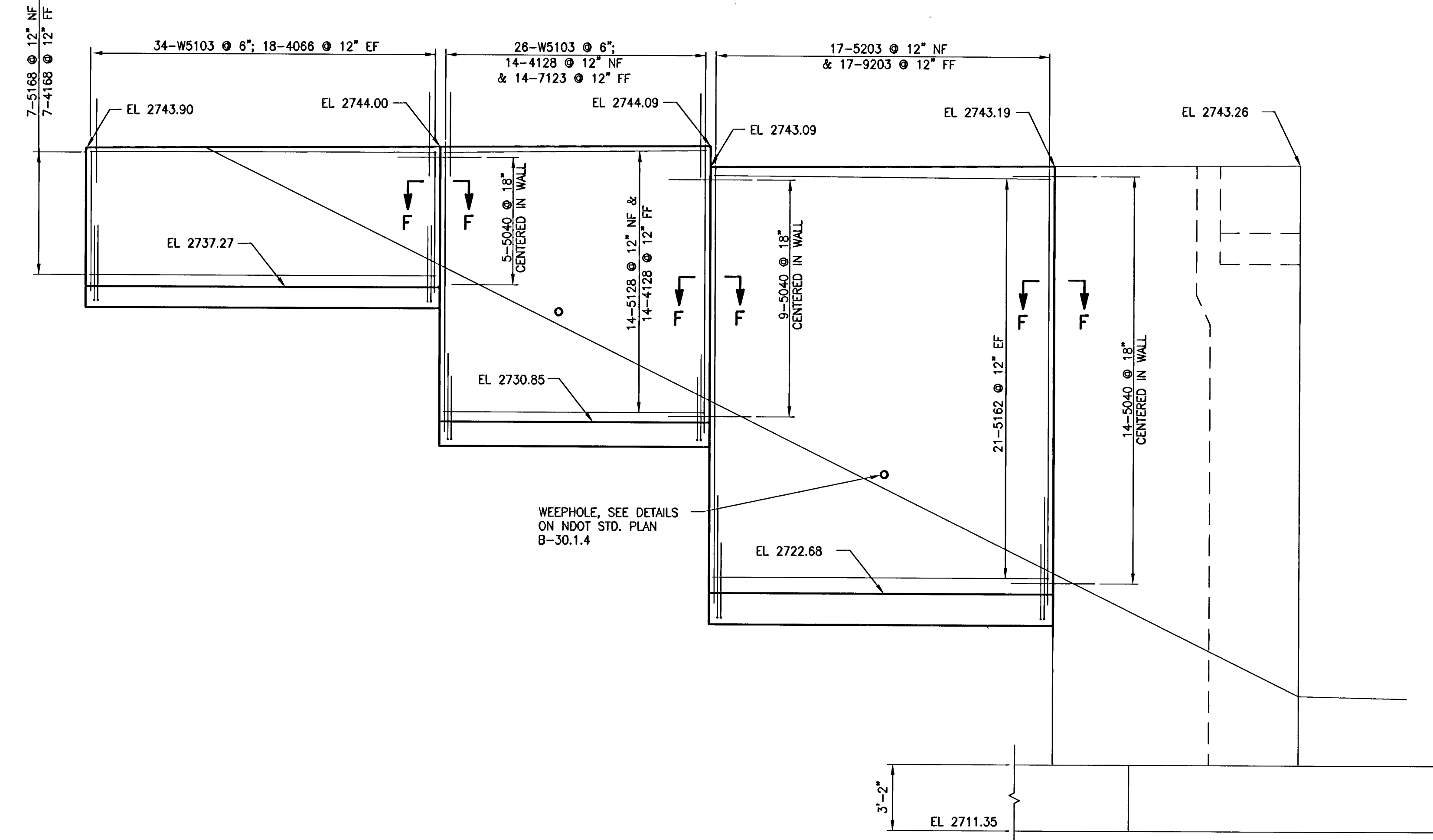
ELEVATION RETAINING WALL 8
