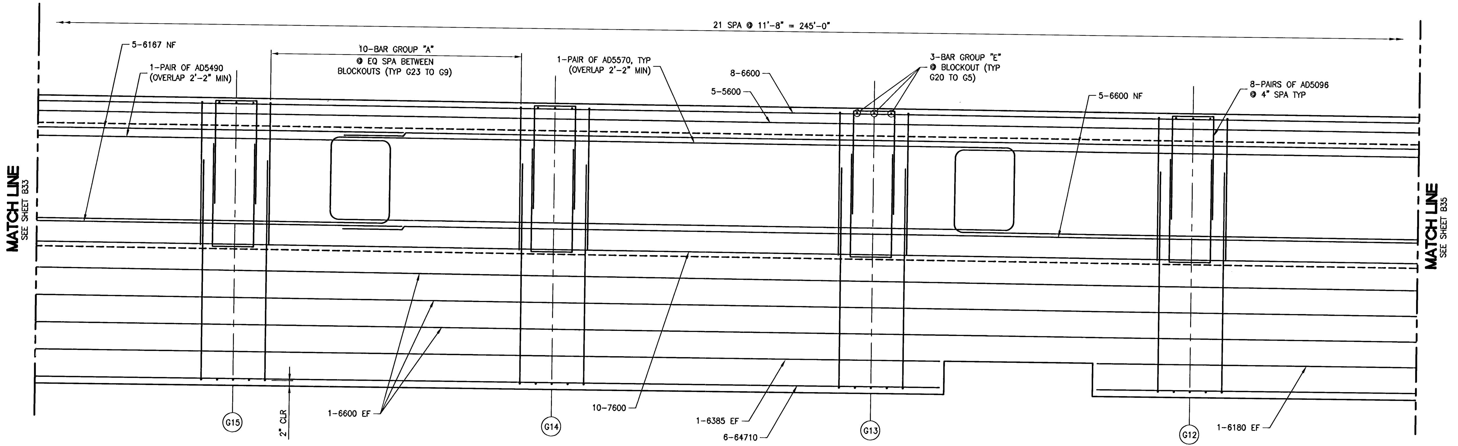
PARTIAL ELEVATION (LOOKING BACK STATION)
