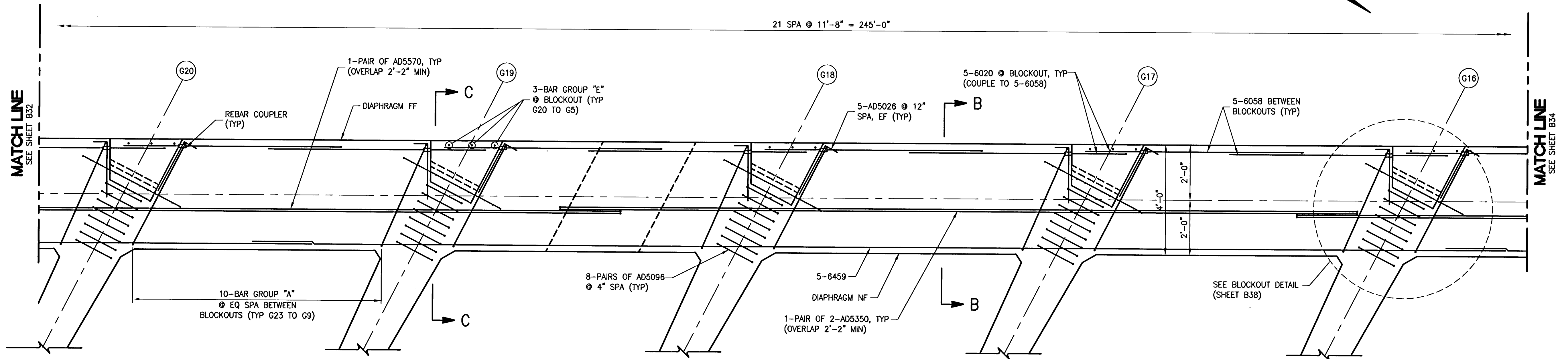
PARTIAL PLAN
