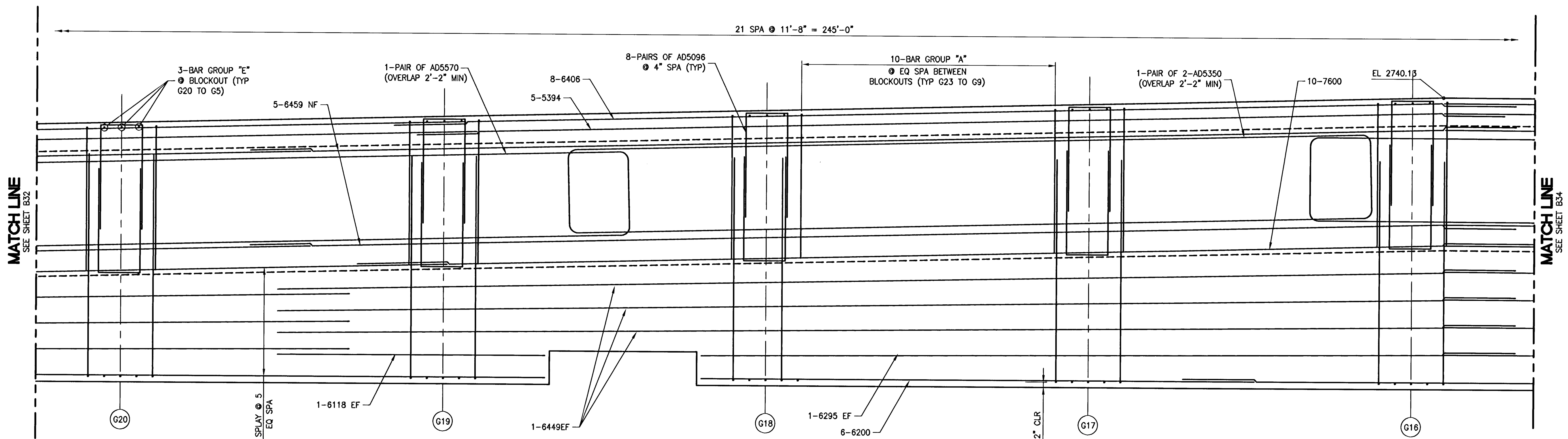
PARTIAL ELEVATION (LOOKING BACK STATION)
