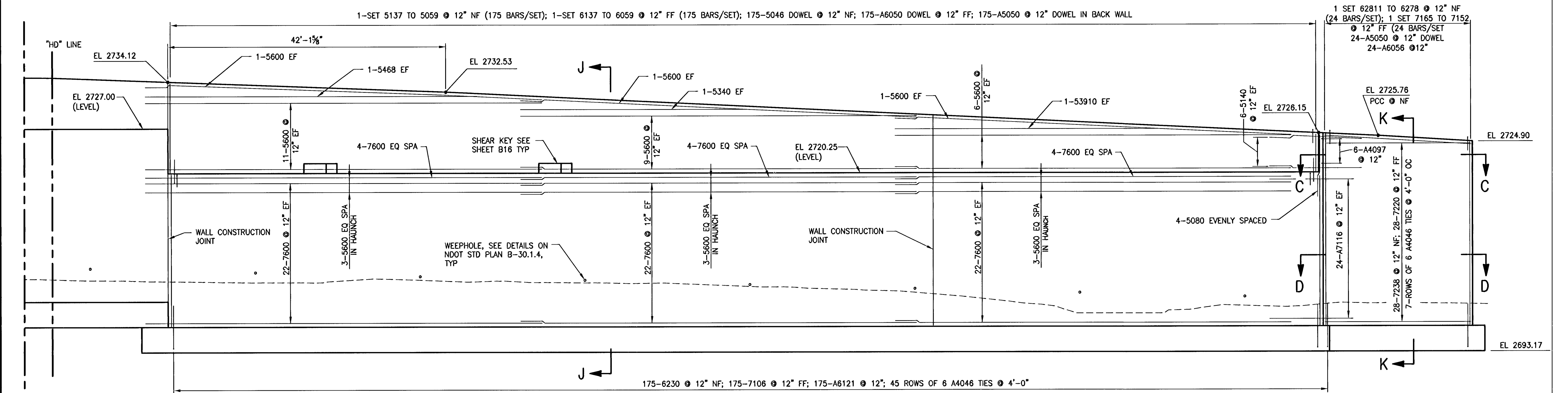
PARTIAL ELEVATION 2
