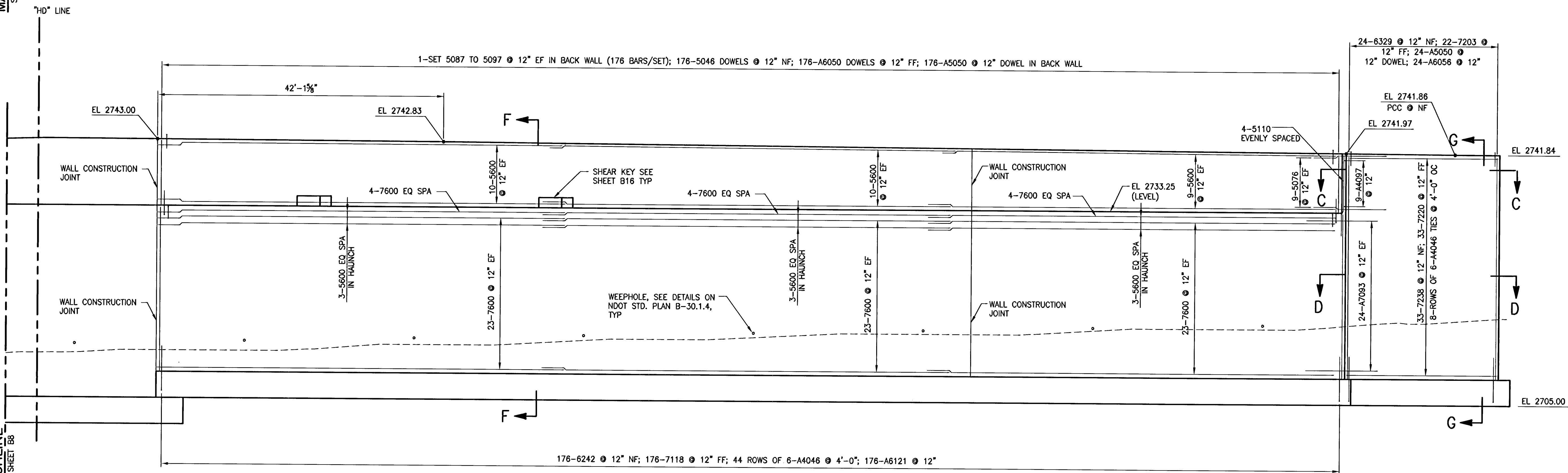
PARTIAL ELEVATION 2
