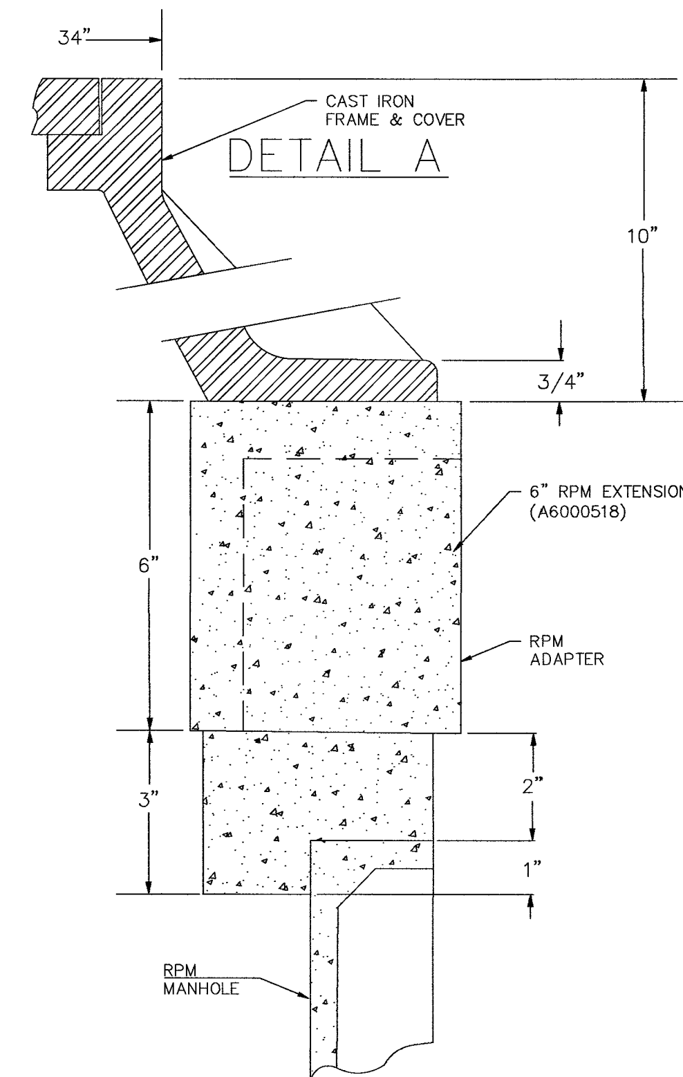
DETAIL B
