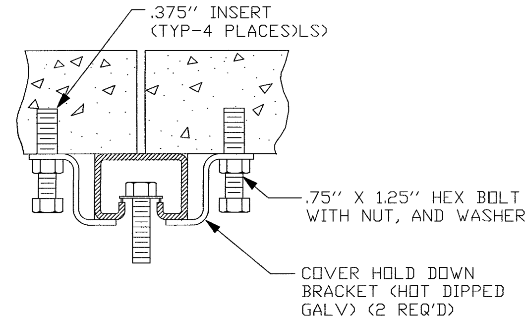
DETAIL "A-4"
