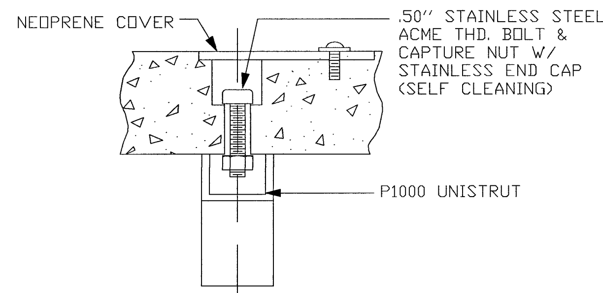
DETAIL "A-3"
