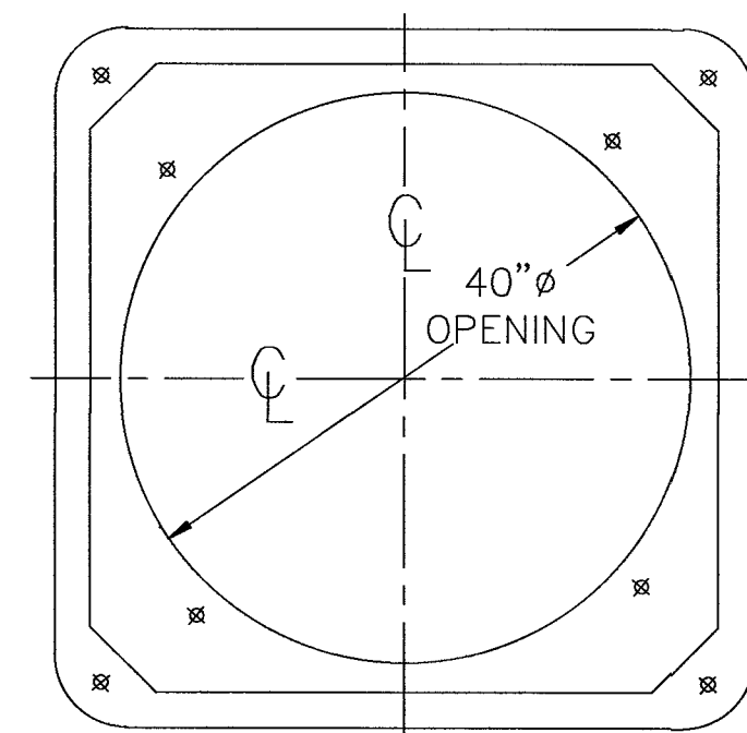
POLYMER CONCRETE ADAPTER SECTION C-C
