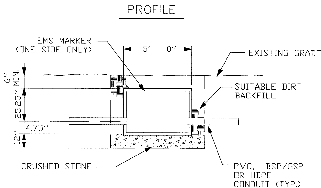
DETAIL "C" EXCAVATION PIT
