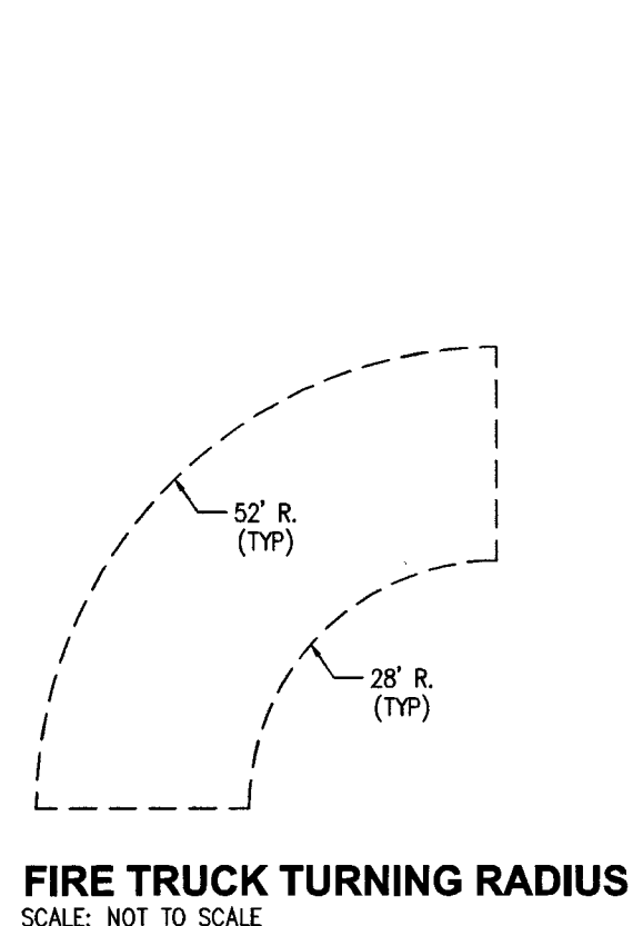
FIRE TRUCK TURNING RADIUS SCALE: NOT TO SCALE
