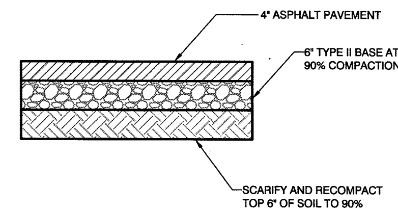
ASPHALT PAVEMENT SECTION NOT TO SCALE
