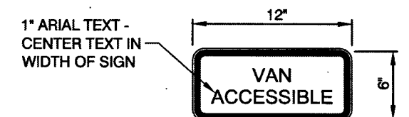
VAN ACCESSIBLE SIGN NOT TO SCALE R7-8b (12" X 18")
