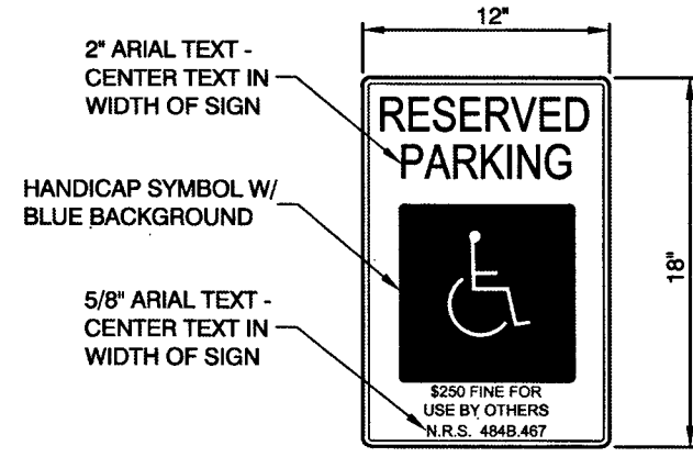
RESERVED PARKING SIGN NOT TO SCALE R7-8 (12" X 18")
