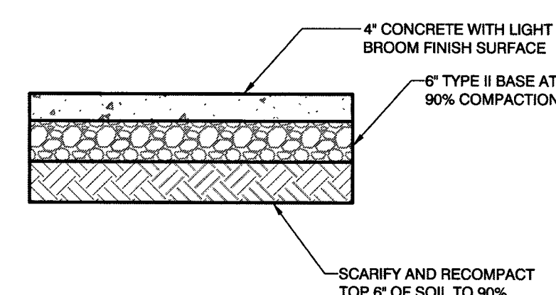
CONCRETE SURFACE SECTION NOT TO SCALE
