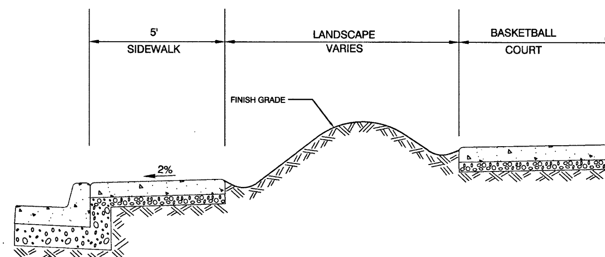
GRADING ADJACENT TO BASKETBALL COURT NOT TO SCALE (SEE STRUCT. PLANS FOR COURT DESIGN)
