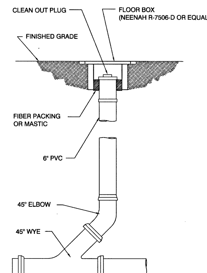
SANITARY SEWER CLEANOUT NOT TO SCALE (SIMILAR TO COWRD DCSWCS SD-26)
