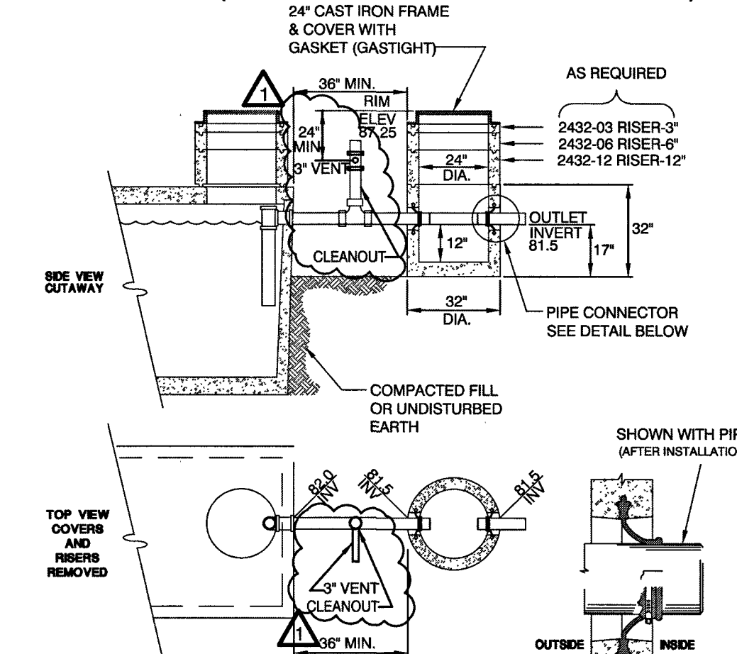
SAMPLE BOX NOT TO SCALE 'TR' STA 15+36.1, 107.6' RT
