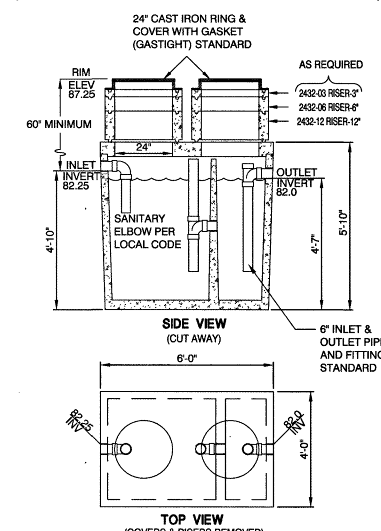
500 GAL SAND-OIL INTERCEPTOR NOT TO SCALE 'TR' STA 15+36.1, 114.8' RT
