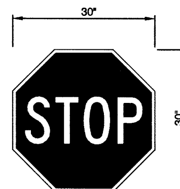
STOP SIGN NOT TO SCALE R1-1 (30" X 30")
