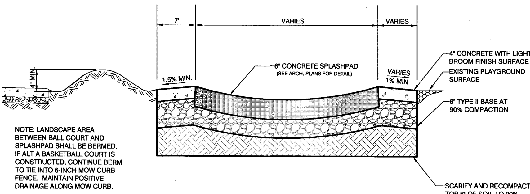
SPASHPAD GRADING SECTION (WITH ALT A SHOWN) NOT TO SCALE (SEE ARCH. PLANS FOR SPASHPAD DESIGN AND DETAILS)
