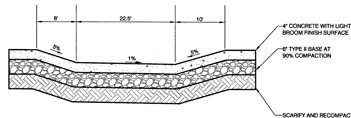
PARKING LOT ACCESSIBLE RAMP SECTION NOT TO SCALE
