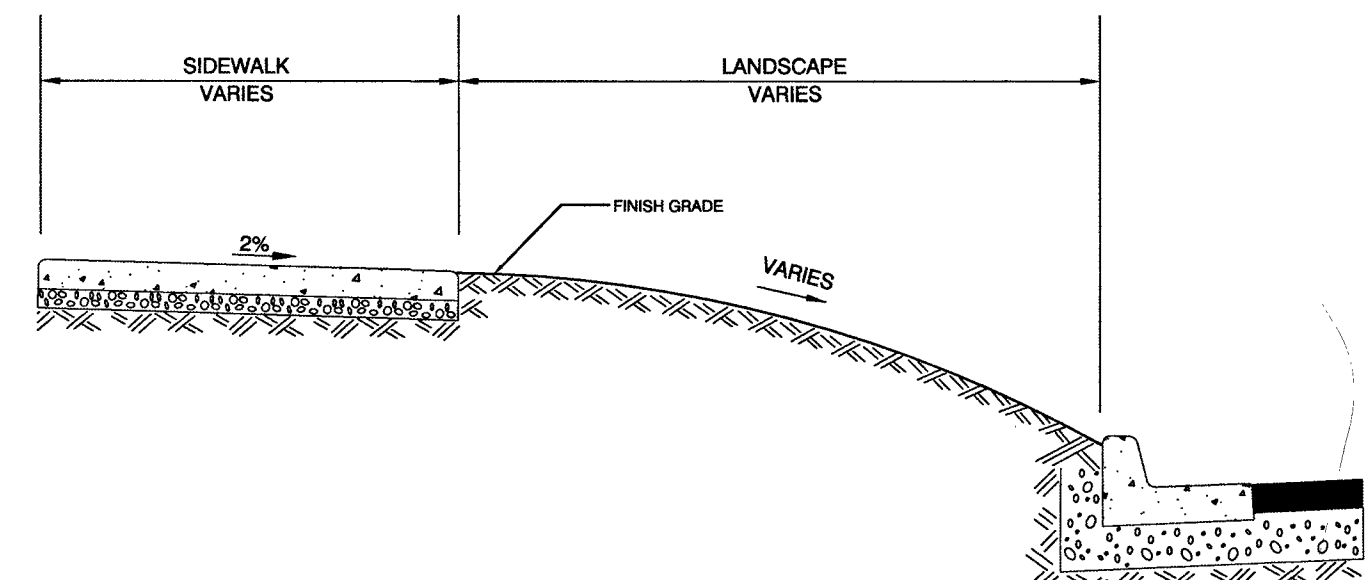
OFFSET SIDEWALK GRADING SECTION NOT TO SCALE
