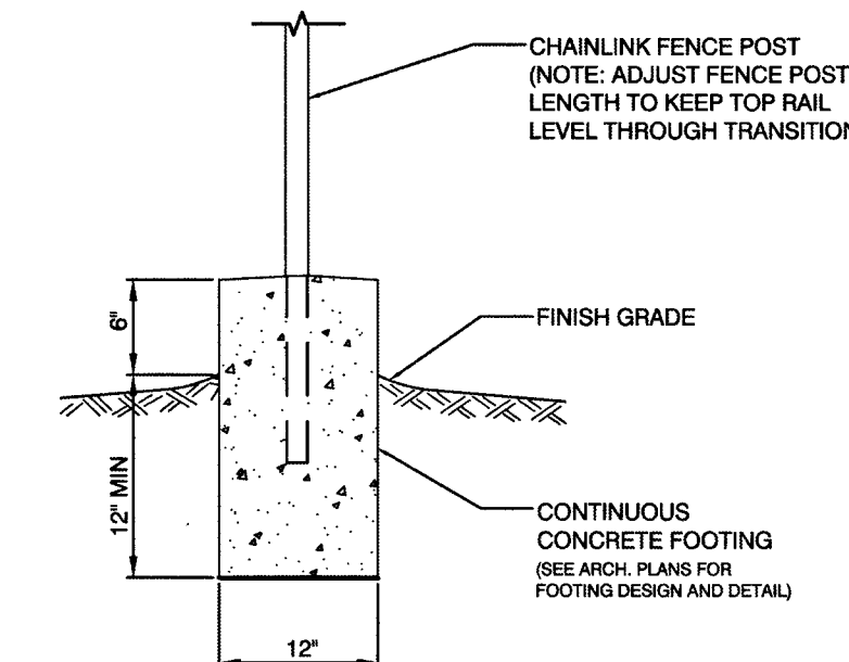
ELEVATED MOW CURB FENCE NEAR SPASHPAD NOT TO SCALE (SEE ARCH. PLANS FOR FENCE DETAILS)
