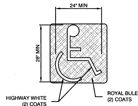
HANDICAP PARKING SYMBOL NOT TO SCALE
