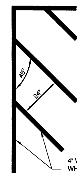
CHEVRON STRIPING DETAIL NOT TO SCALE
