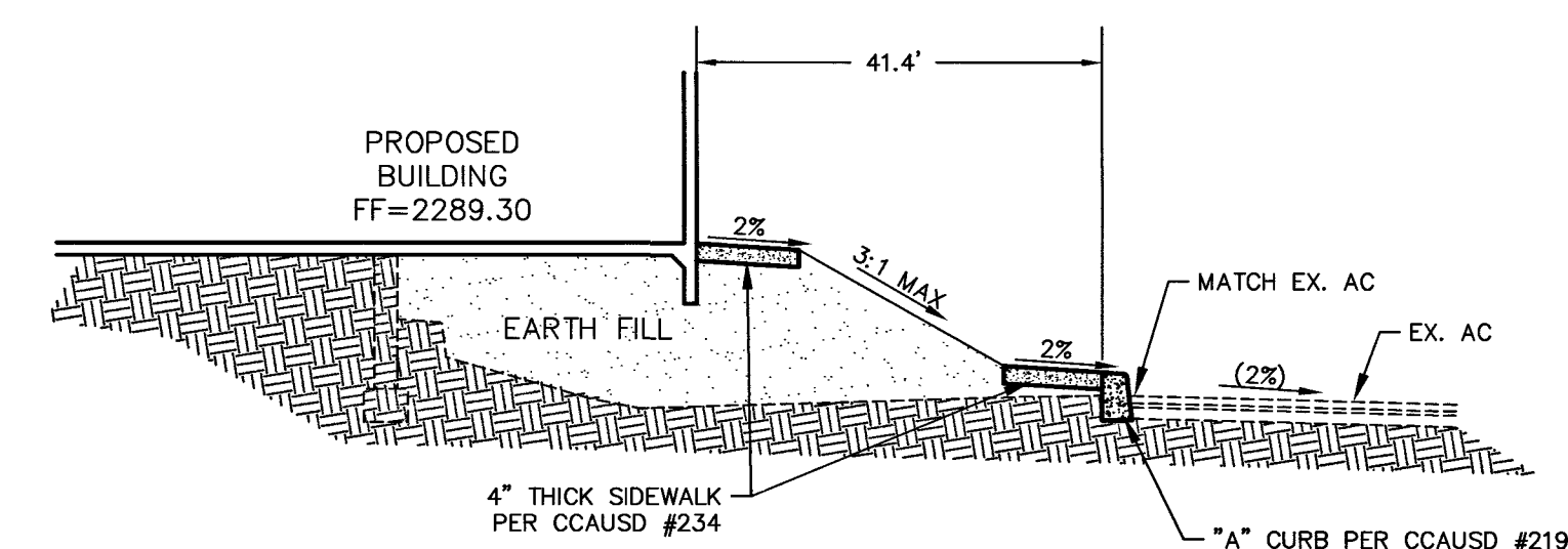
SECTION
