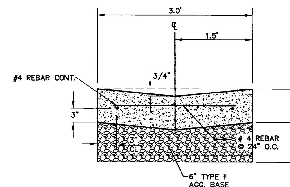
3' VALLEY GUTTER
