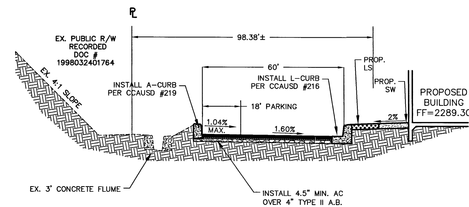
SECTION
