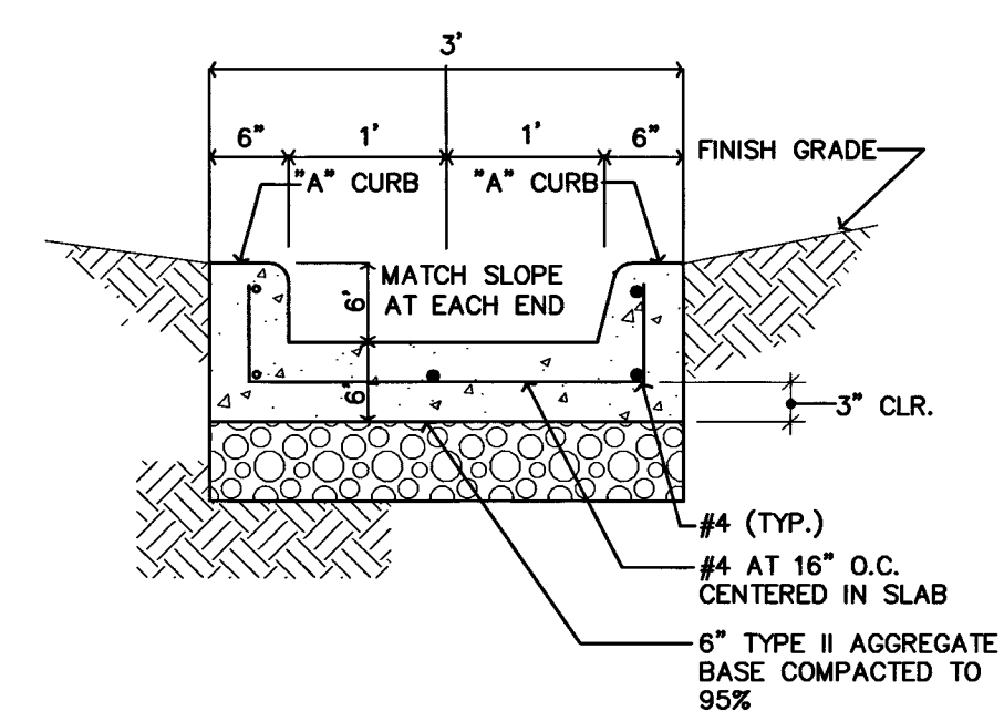
3' CONCRETE FLUME
