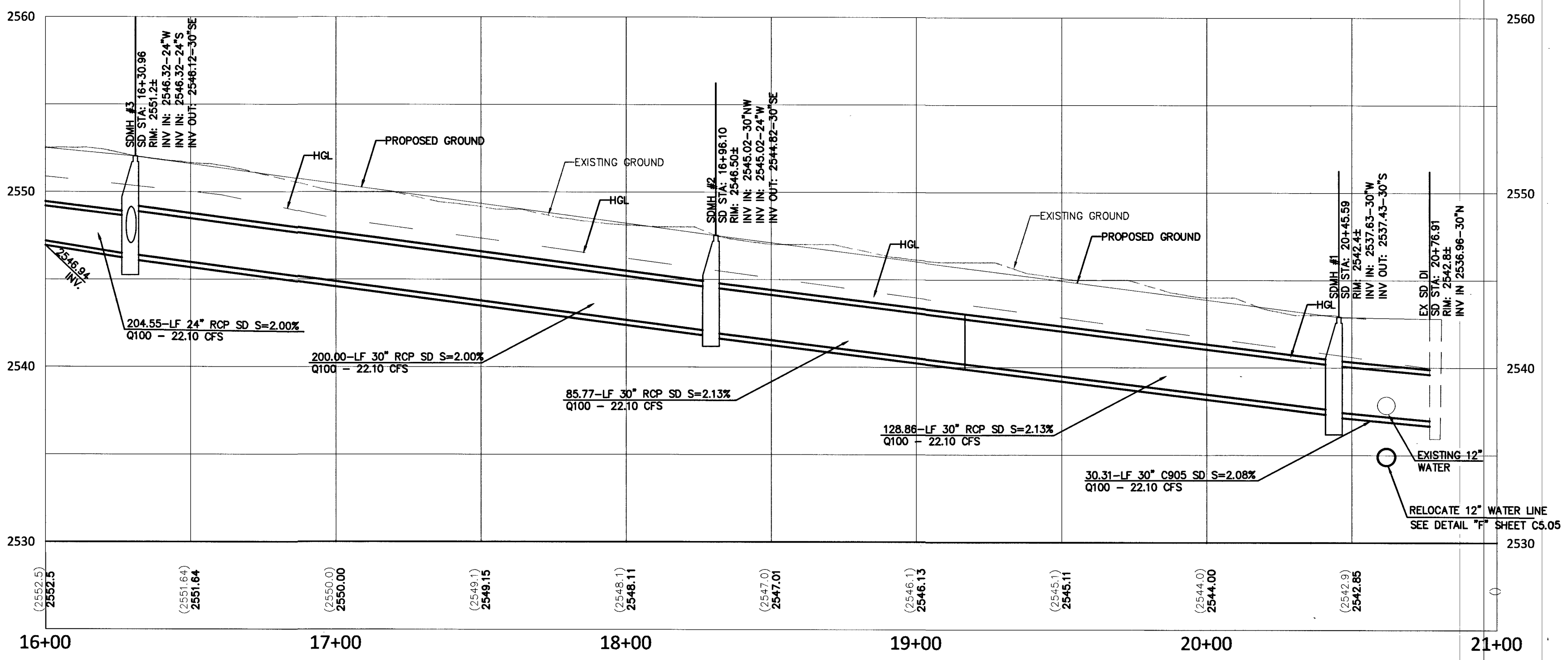
PROFILE VIEW H: 1"=30' V: 1"=4'
