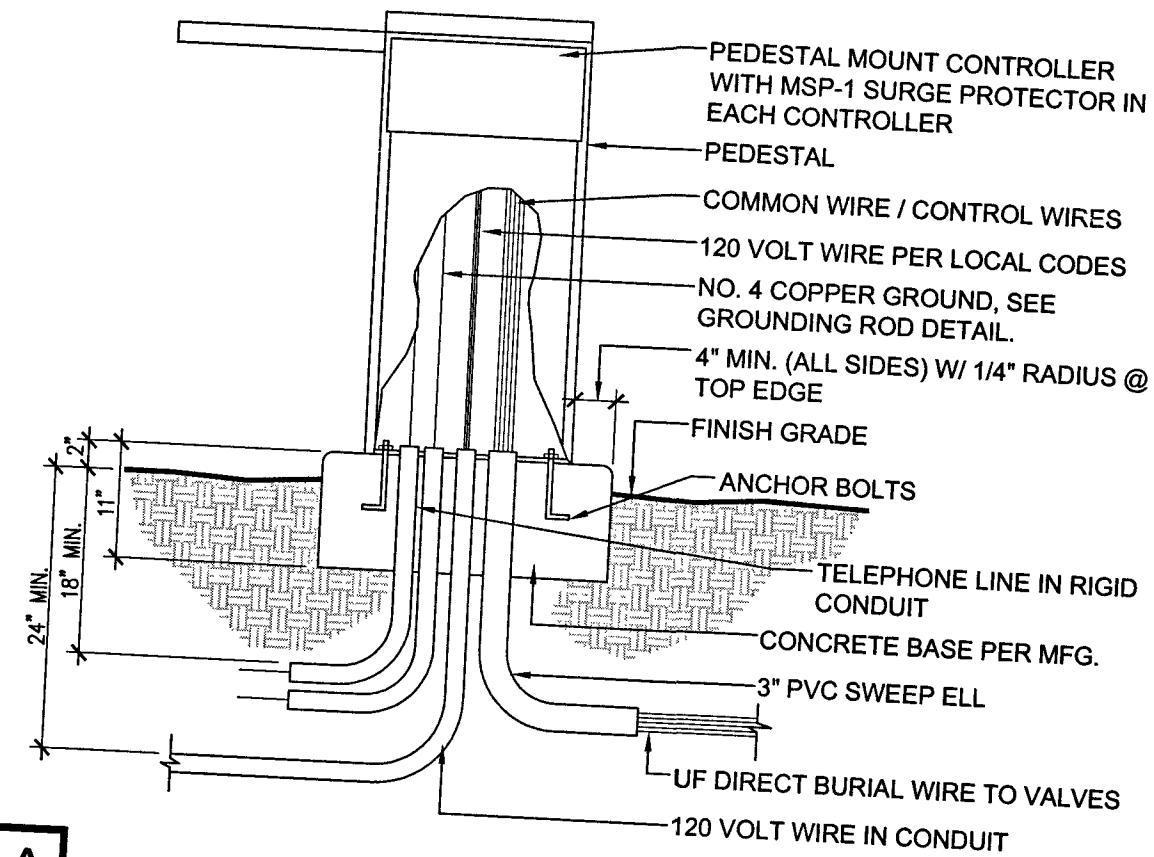
A IRRIGATION CONTROLLER
