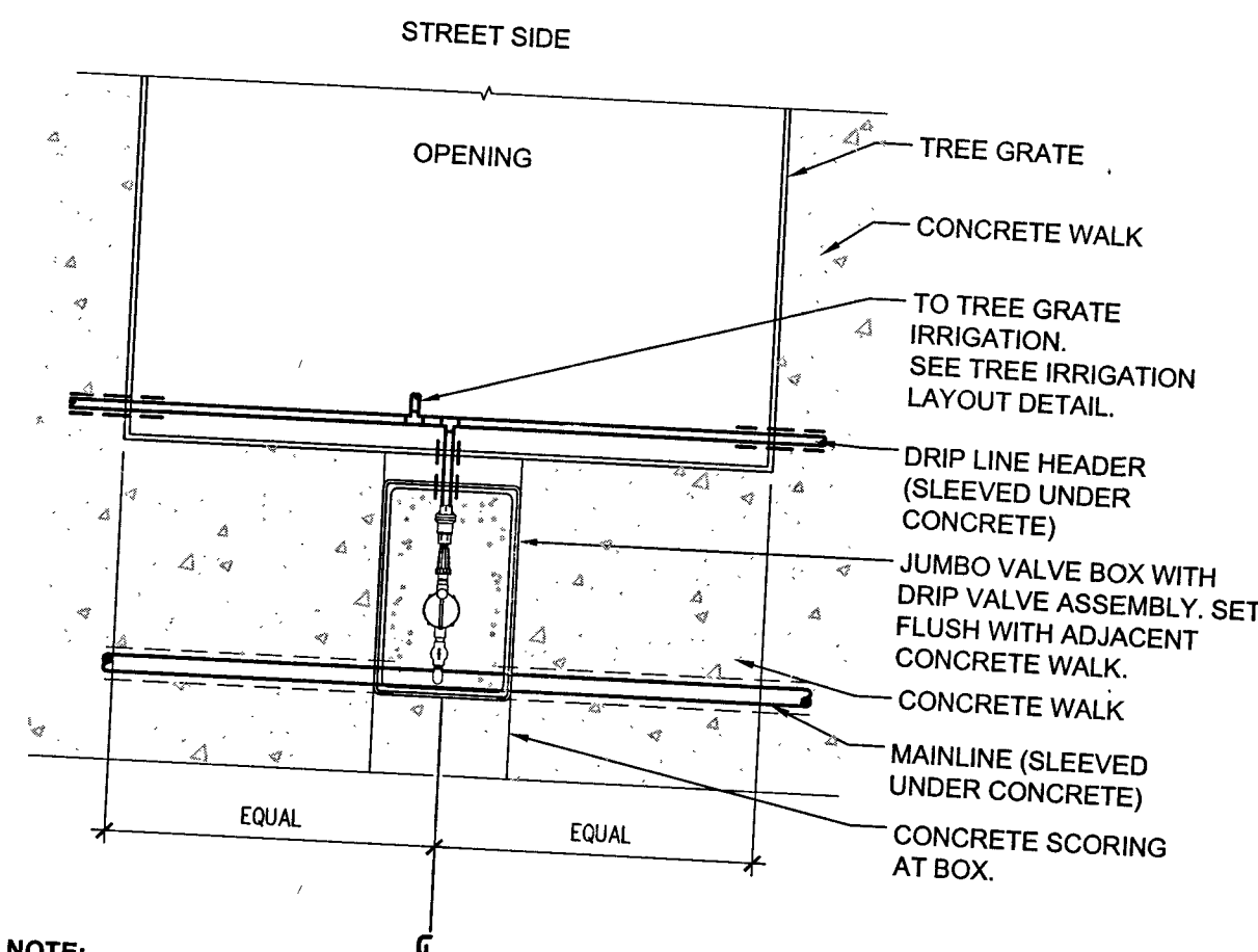
G DRIP VALVE ASSEMBLY AT TREE WELL
