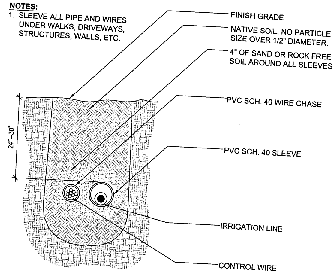
B SLEEVE SECTION
