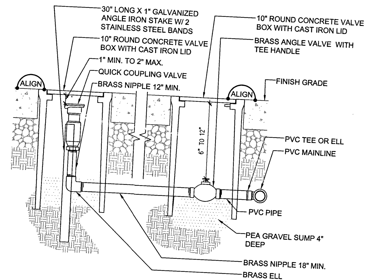
D QUICK COUPLER
