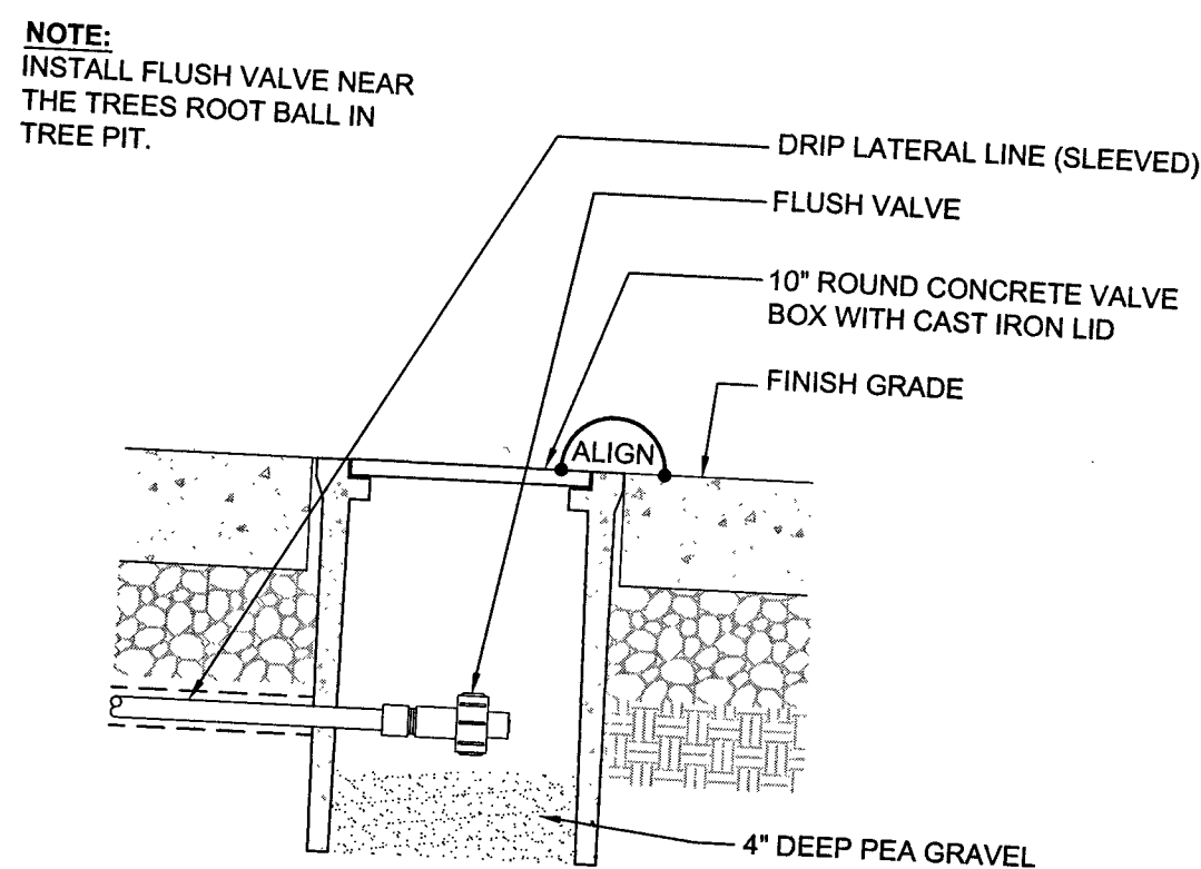
I DRIP FLUSH VALVE
