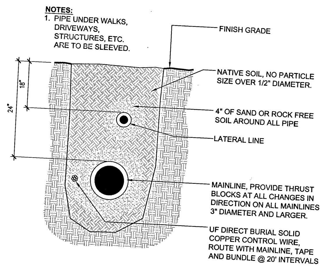
C TRENCH SECTION
