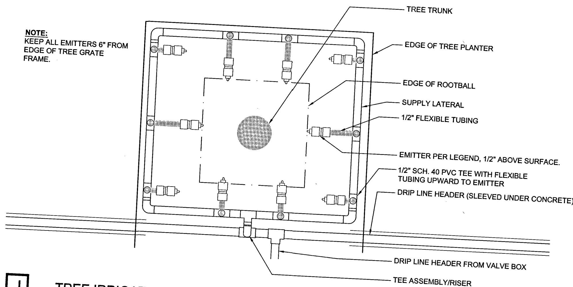
J TREE IRRIGATION LAYOUT
