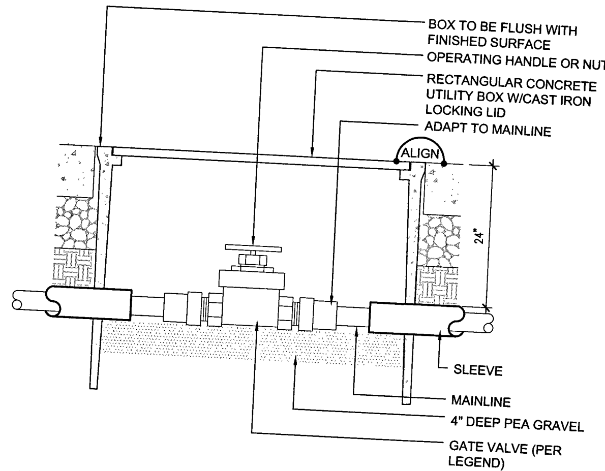
E GATE VALVE IN LARGE VALVE BOX
