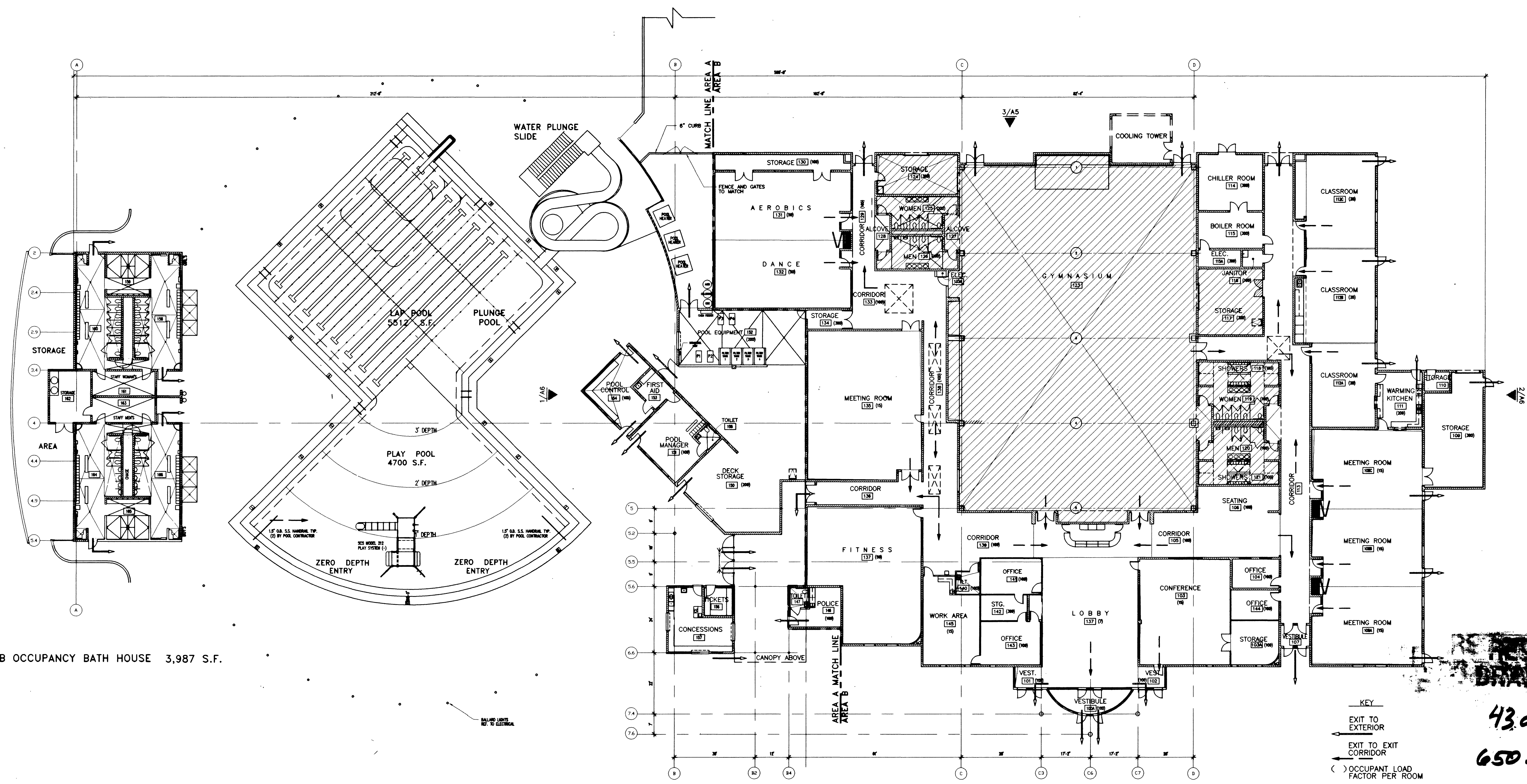
1 KEY PLAN / EXITING PLAN A1 SCALE: 1/16" = 1'-0"
