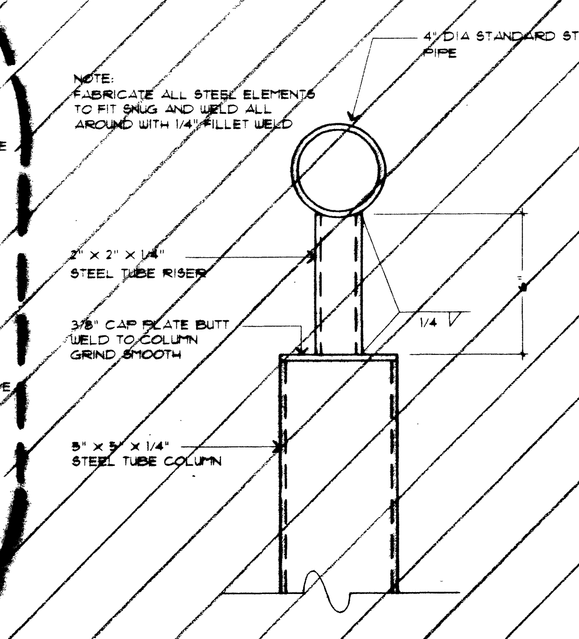
POST TO ROOF CONNECTION SCALE: 3/8"=1'-0"
