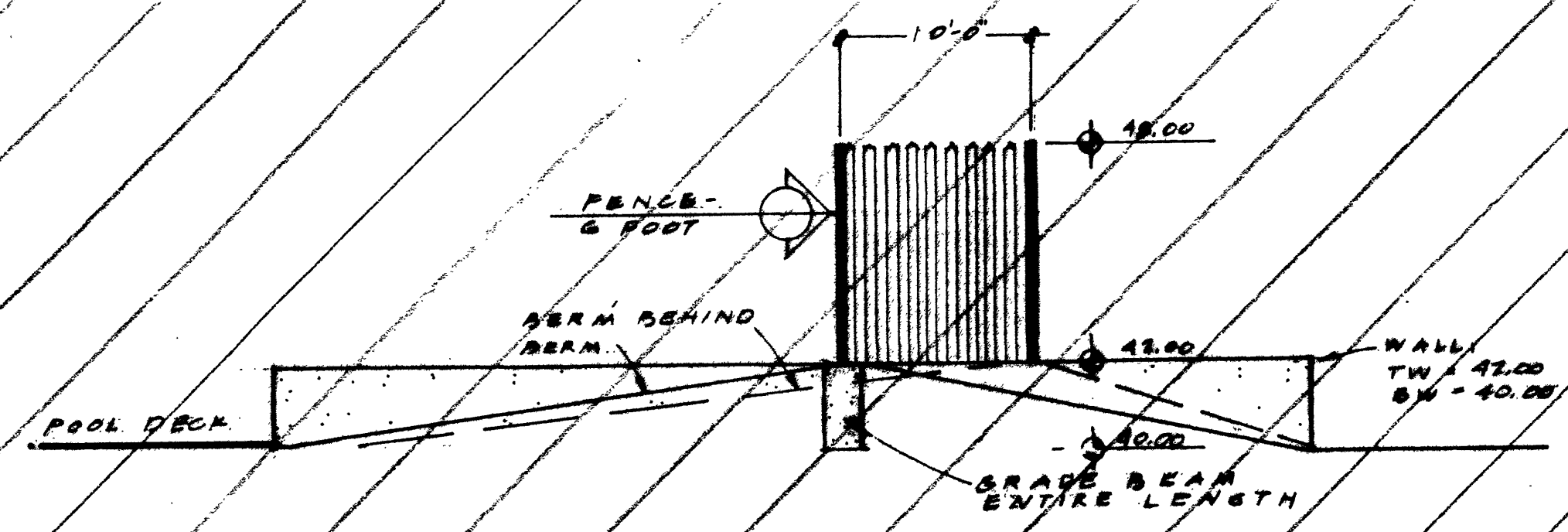
POOL AREA AT SOUTHEAST-SECTION C-C VERT.: 1/4"=1'-0" HORIZ.: 1/8"=1'-0"
