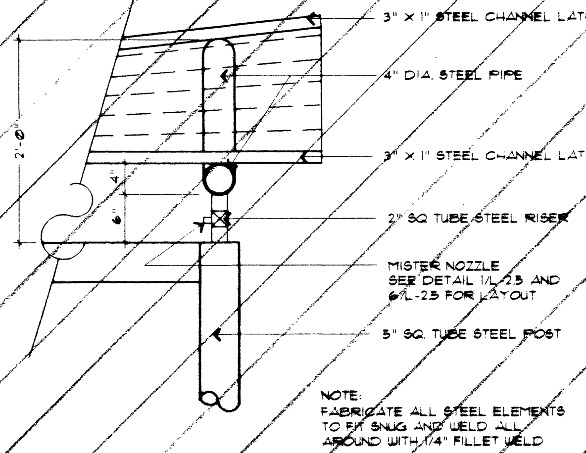
POST TO ROOF-FRONT NTS
