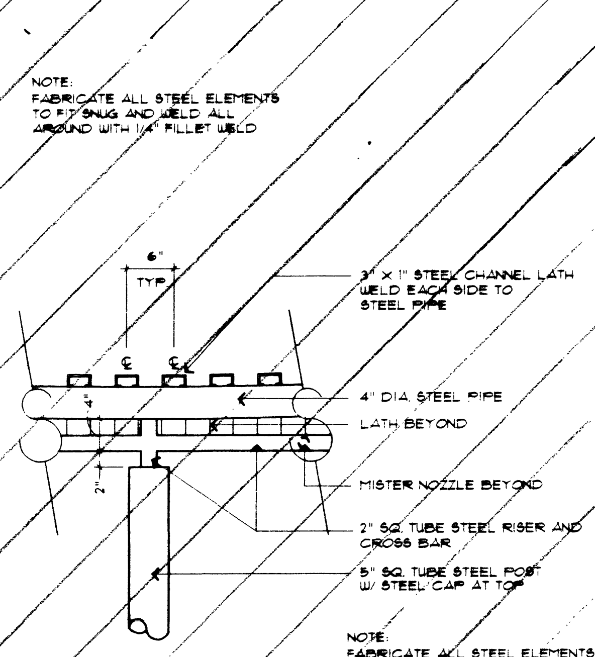
POST TO ROOF-LOW POINT SCALE: 1"=1'-0"
