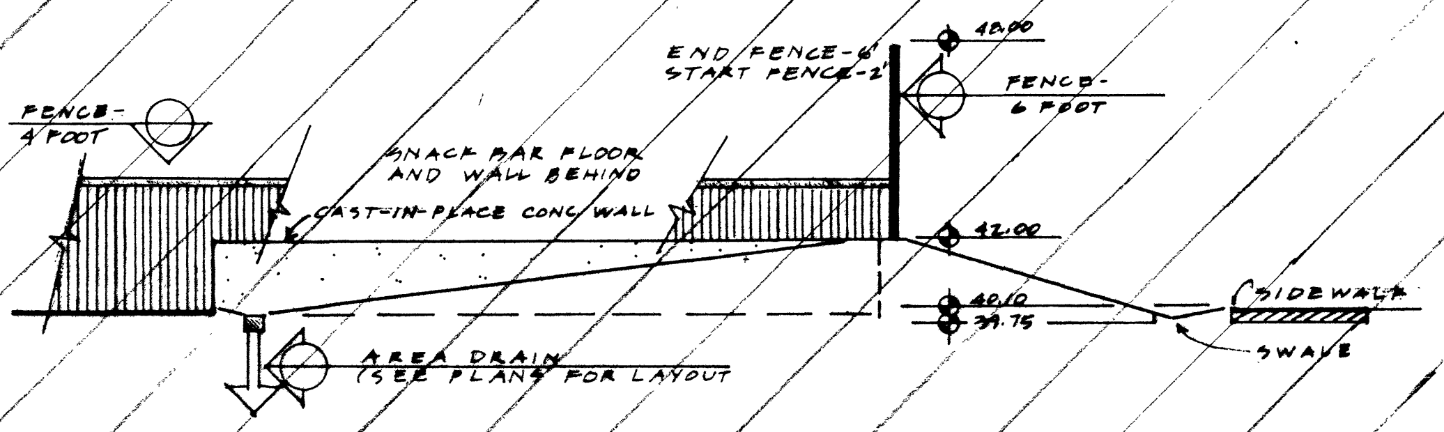
SECTION AT SOUTH END OF SNACK BAR-SECTION B-B VERT.: 1/4"=1'-0" HORIZ.: 1/8"=1'-0"
