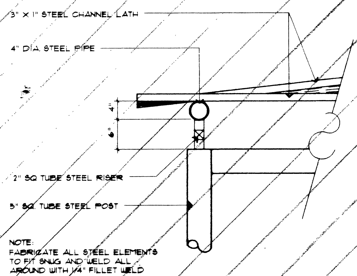
POST TO ROOF-BACK SCALE: 1"=1'-0"
