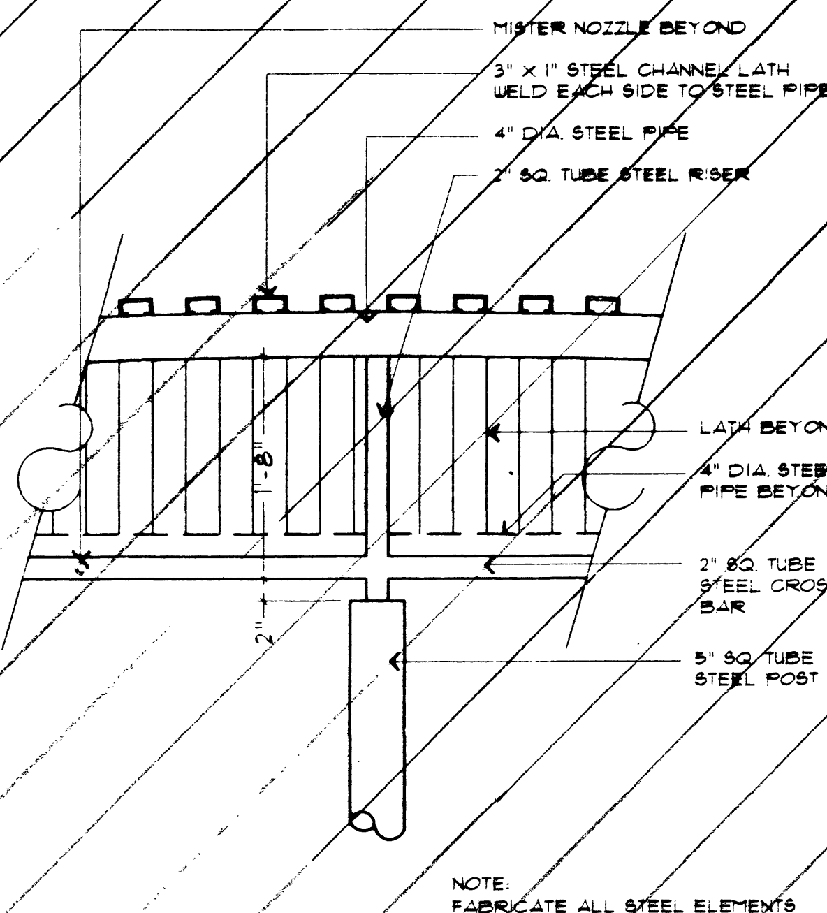
POST TO ROOF-HIGH POINT SCALE: 1"=1'-0"
