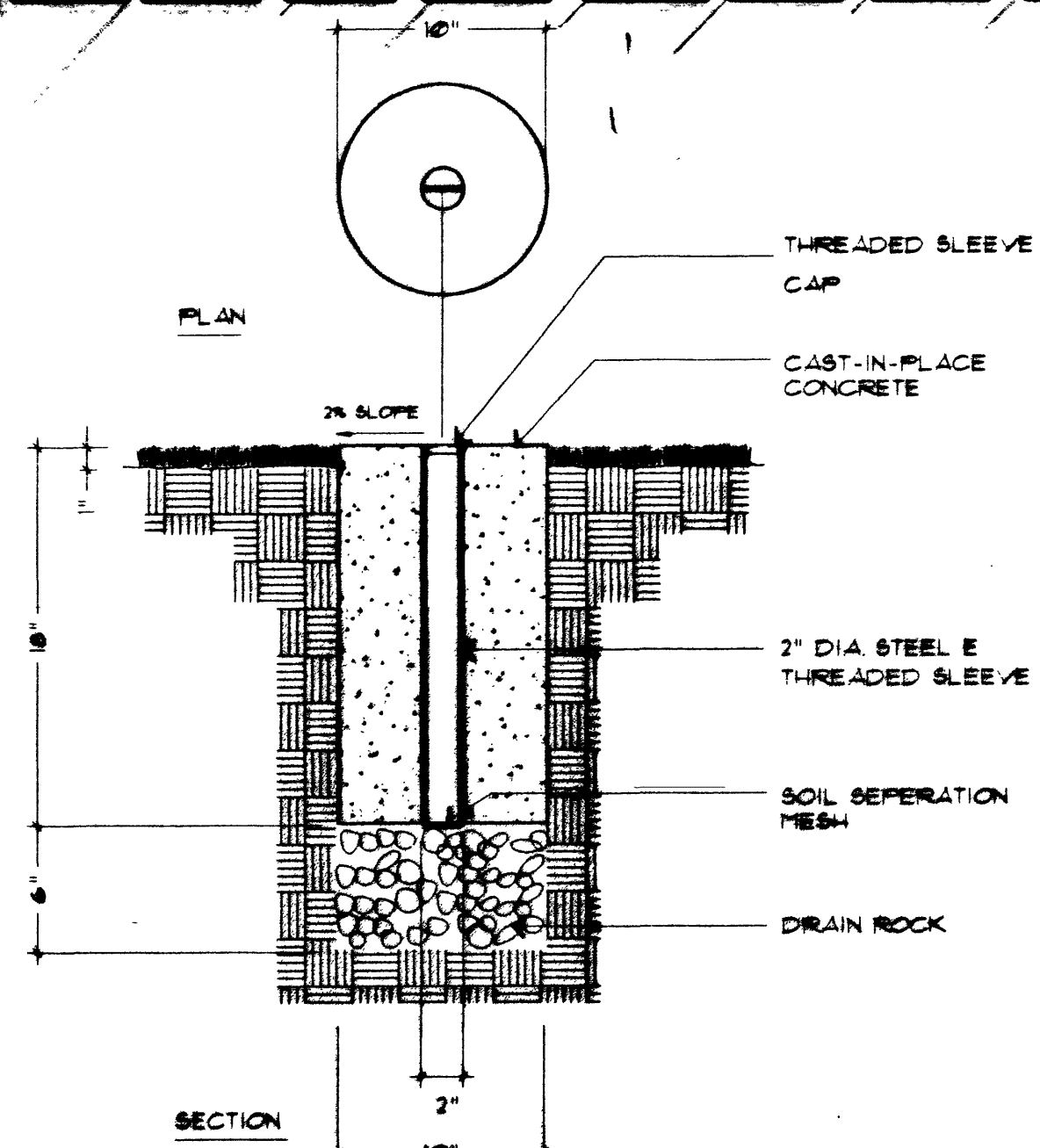
UMBRELLA SLEEVE IN LAWN SCALE: 3/4"=1'-0"
