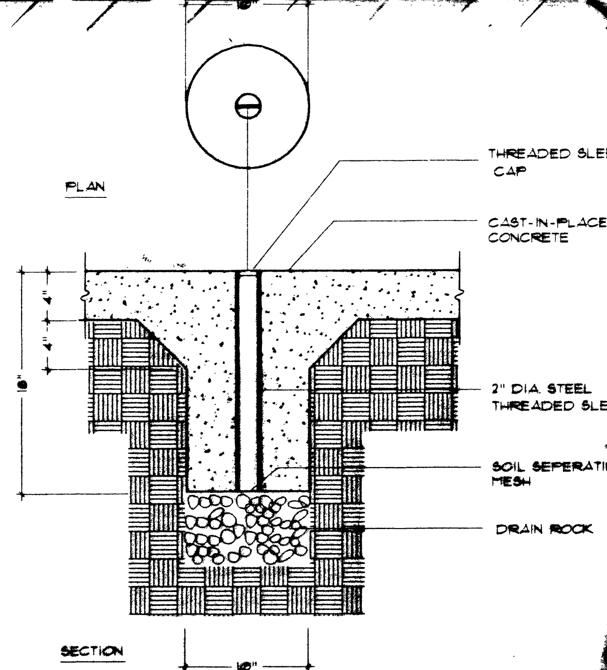
UMBRELLA SLEEVE IN CONC. SCALE: 3/4"=1'-0"
