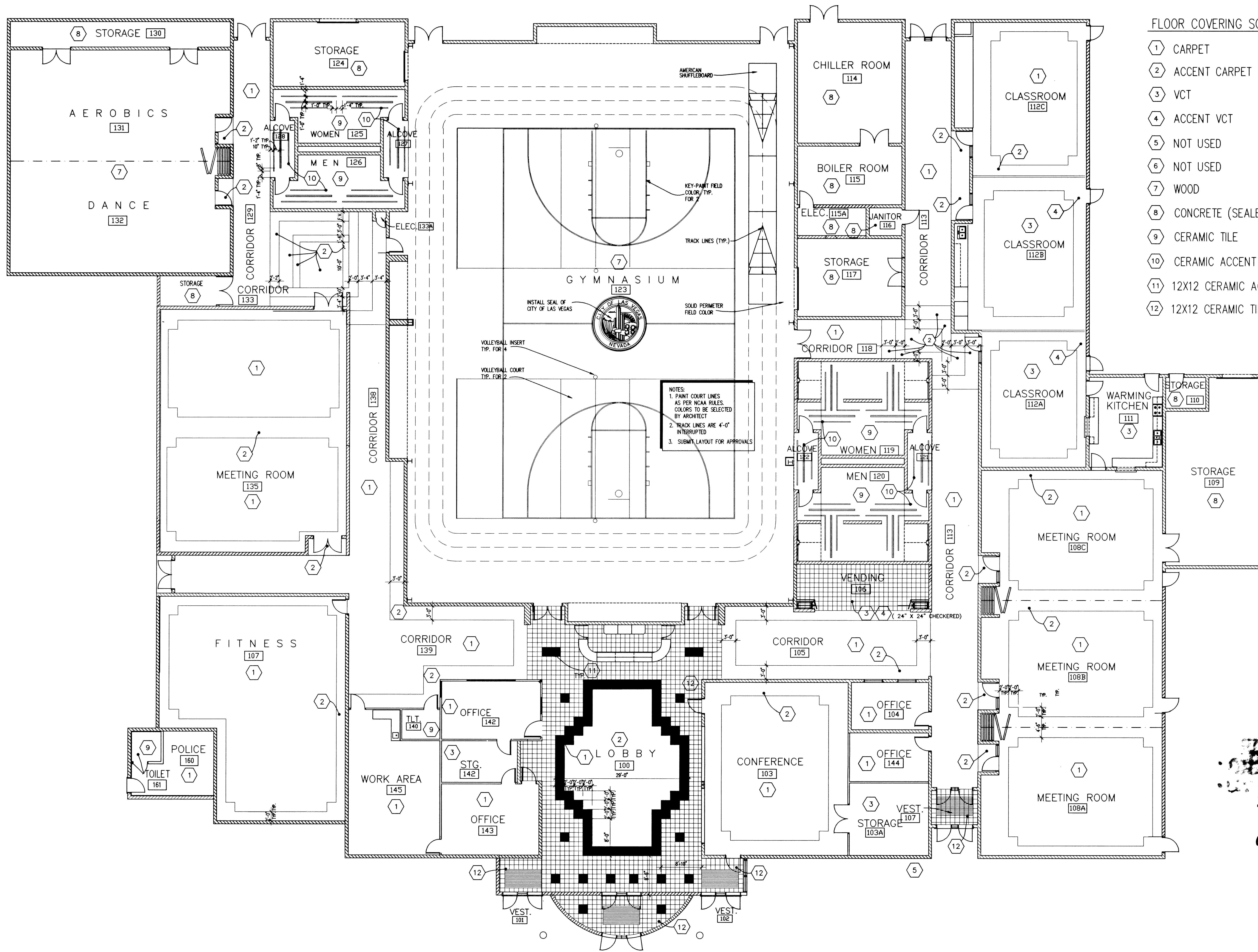
1 FLOOR FINISH PLAN AREA B A29 SCALE: 1/8" = 1'-0"
