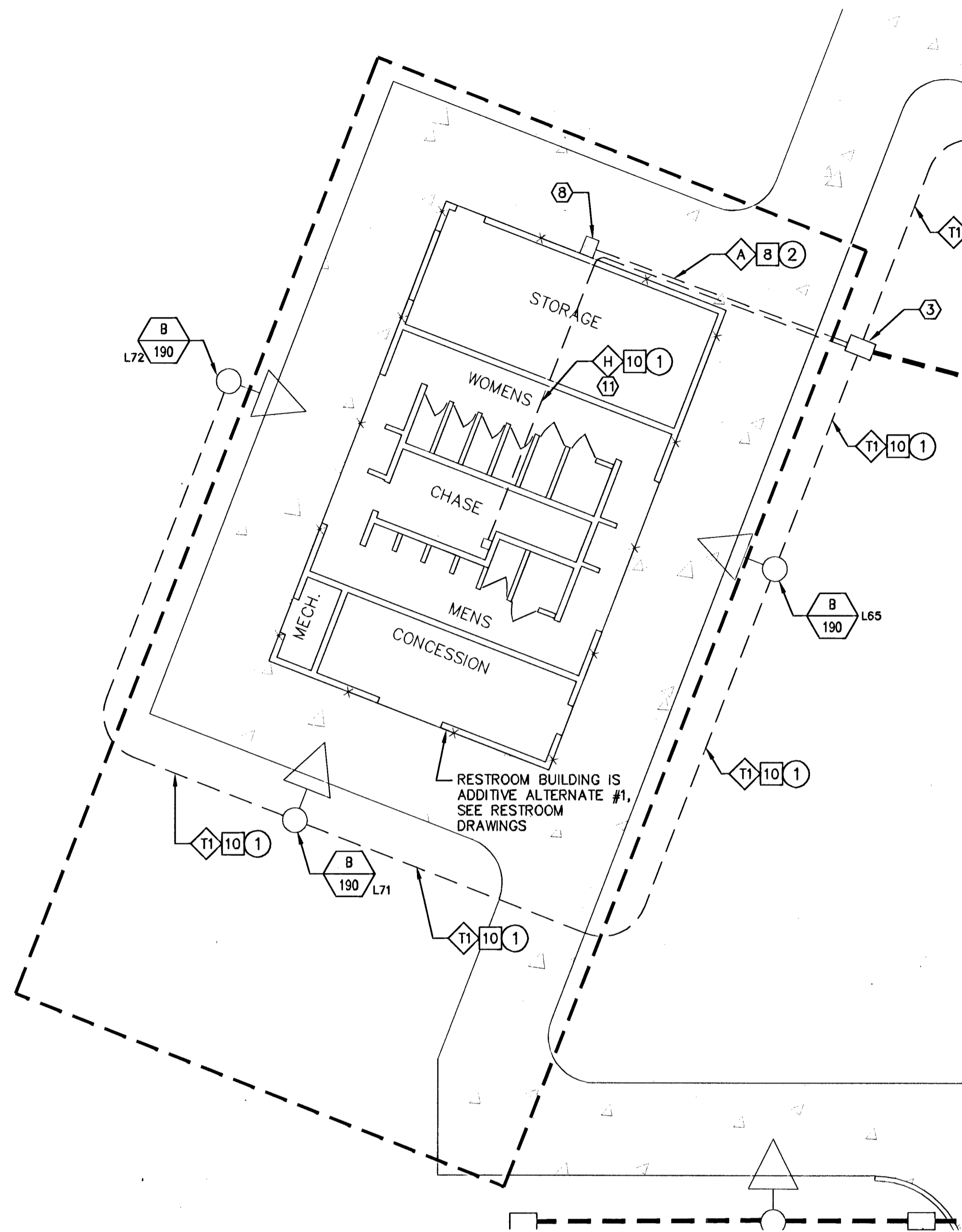
A E-4 ENLARGED RESTROOM ELECTRICAL PLAN SCALE: 1"=10'
