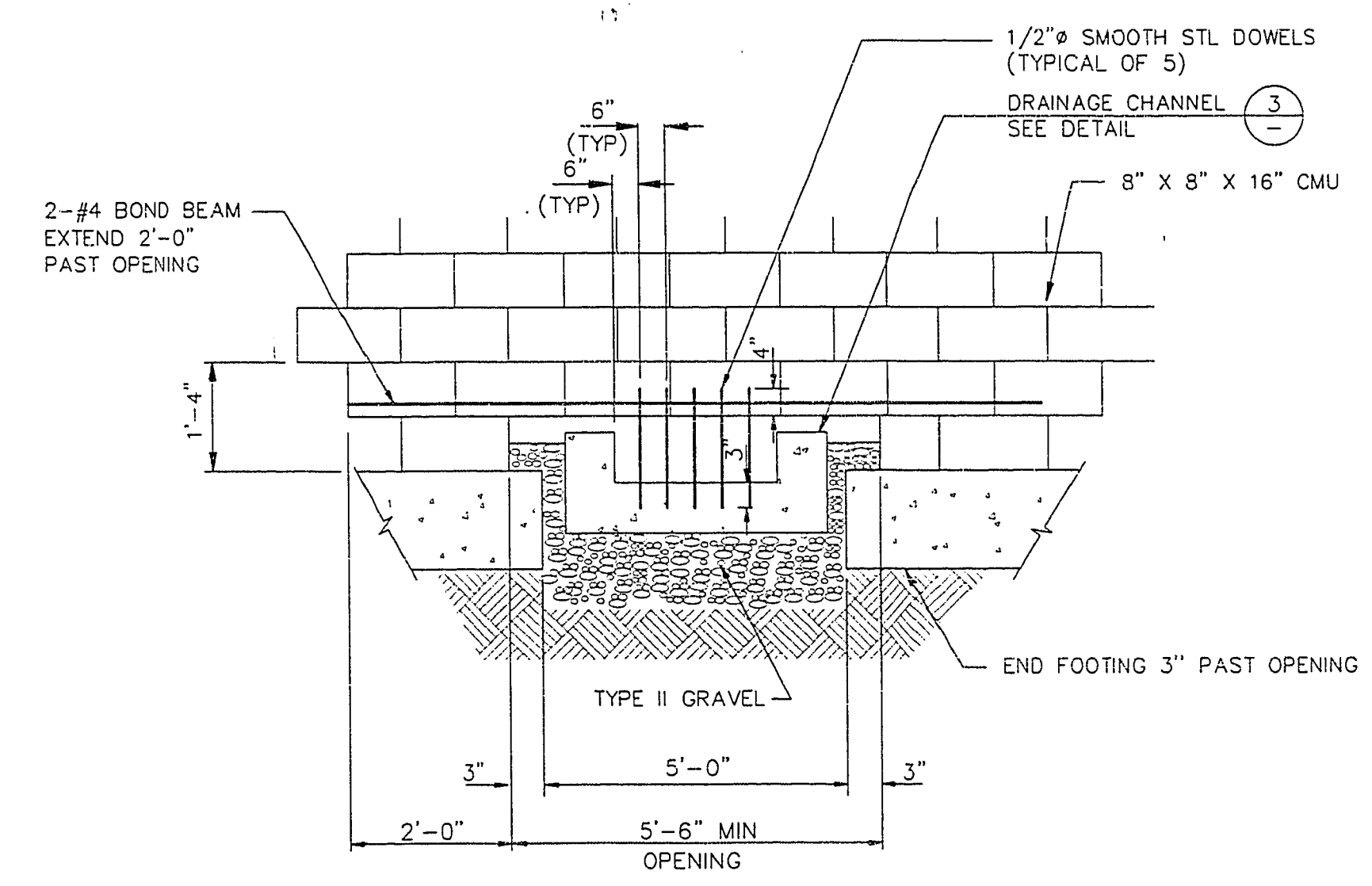
WALL OPENING DETAIL 2 NOT TO SCALE
