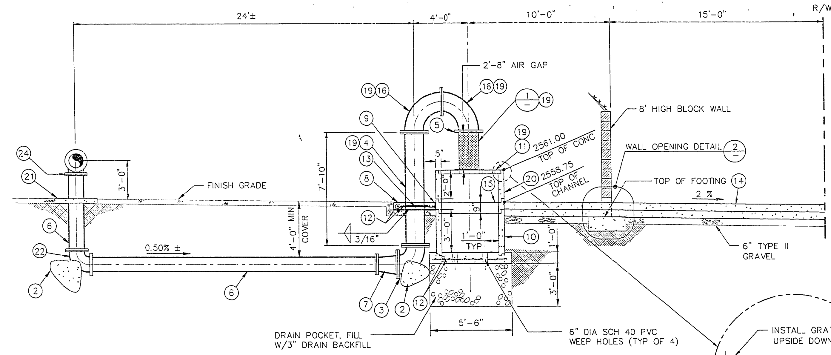
DRAINAGE DISCHARGE PROFILE A SCALE: 1/4"=1'-0"
