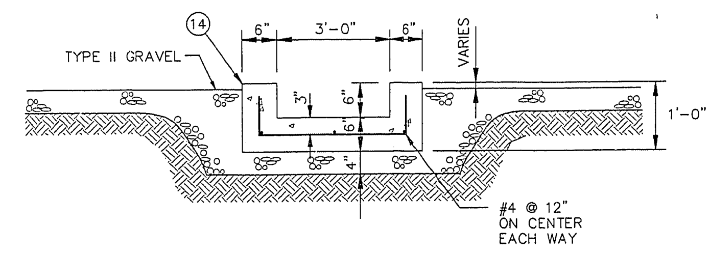
DRAINAGE CHANNEL 3 NOT TO SCALE
