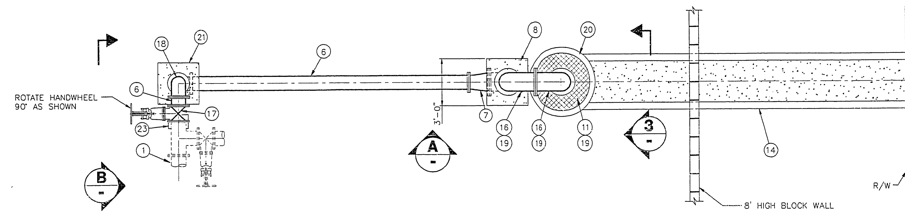
DRAINAGE DISCHARGE PLAN SCALE: 1/4"=1'-0"
