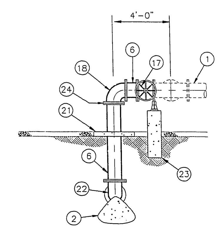
DRAINAGE DISCHARGE PROFILE B SCALE: 1/4"=1'-0"
