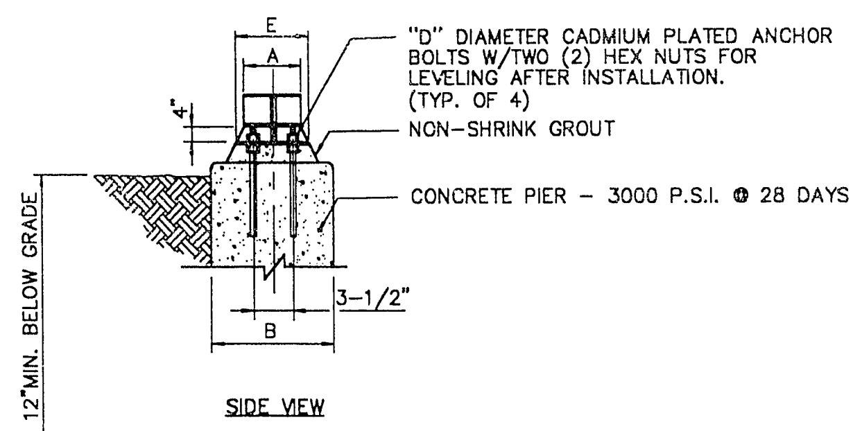
SIDE VIEW
