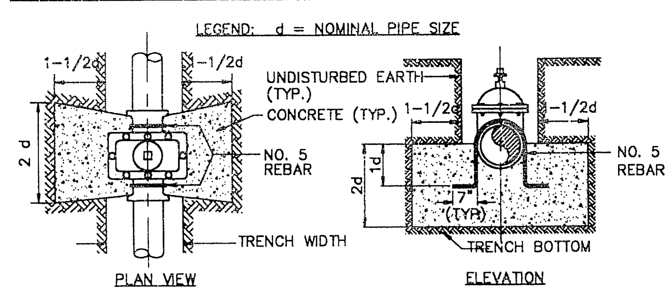
GATE VALVES
