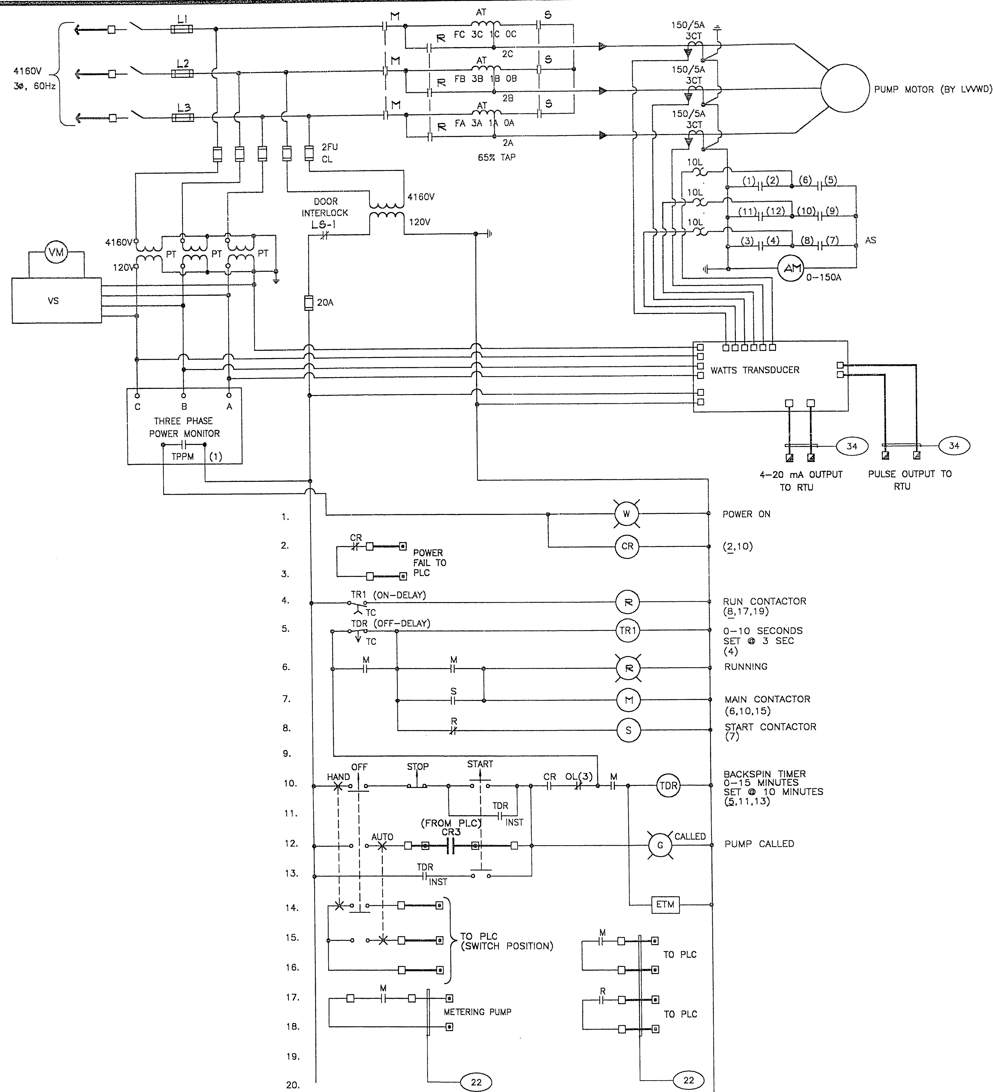
MCC SCHEMATIC DIAGRAM
