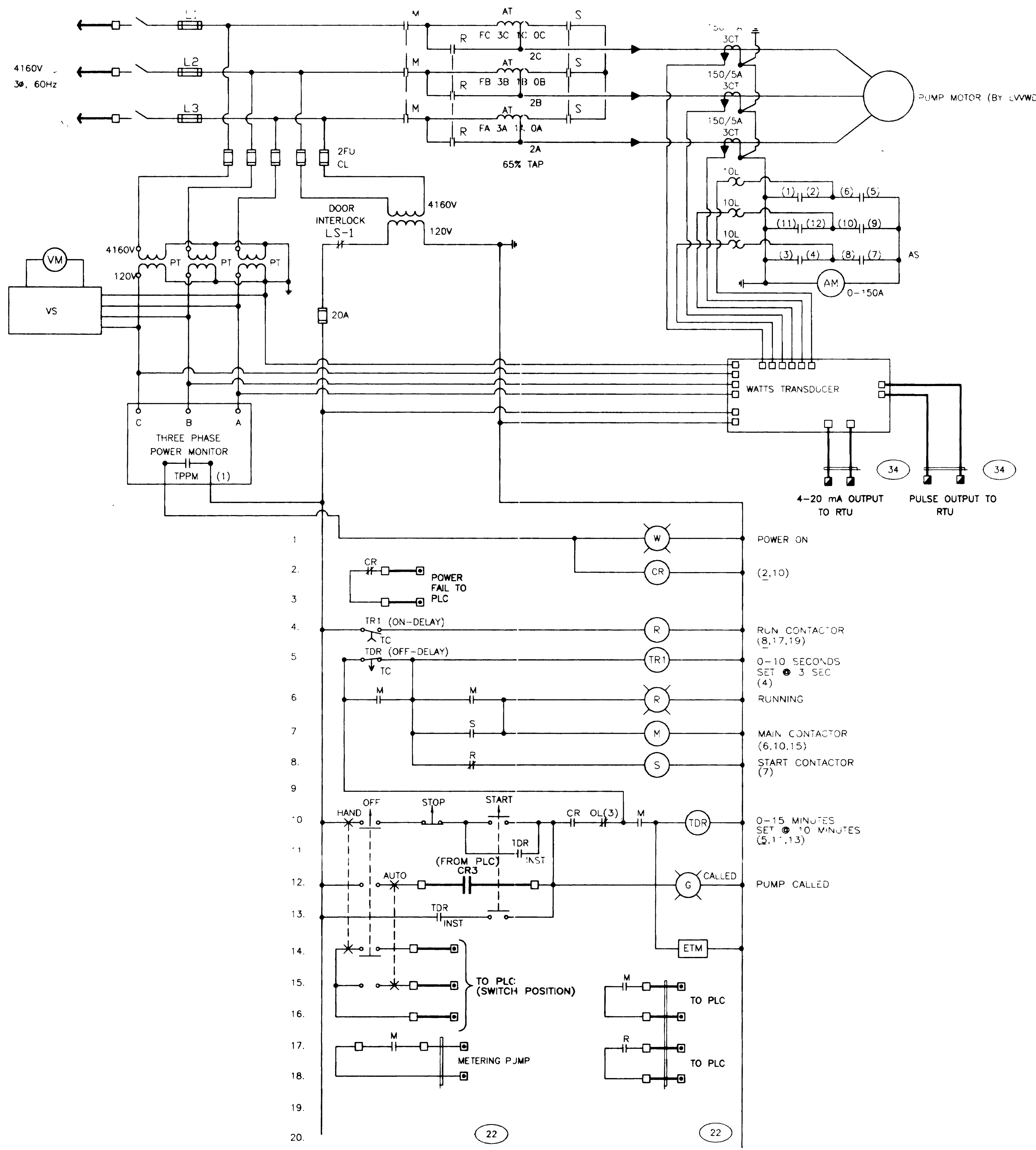
MCC SCHEMATIC DIAGRAM SCALE - NONE
