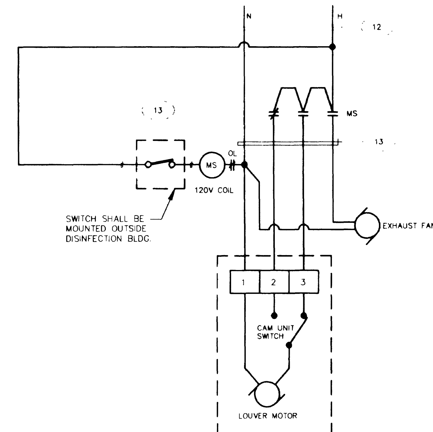
EXHAUST FAN/LOUVERS DIAGRAM
