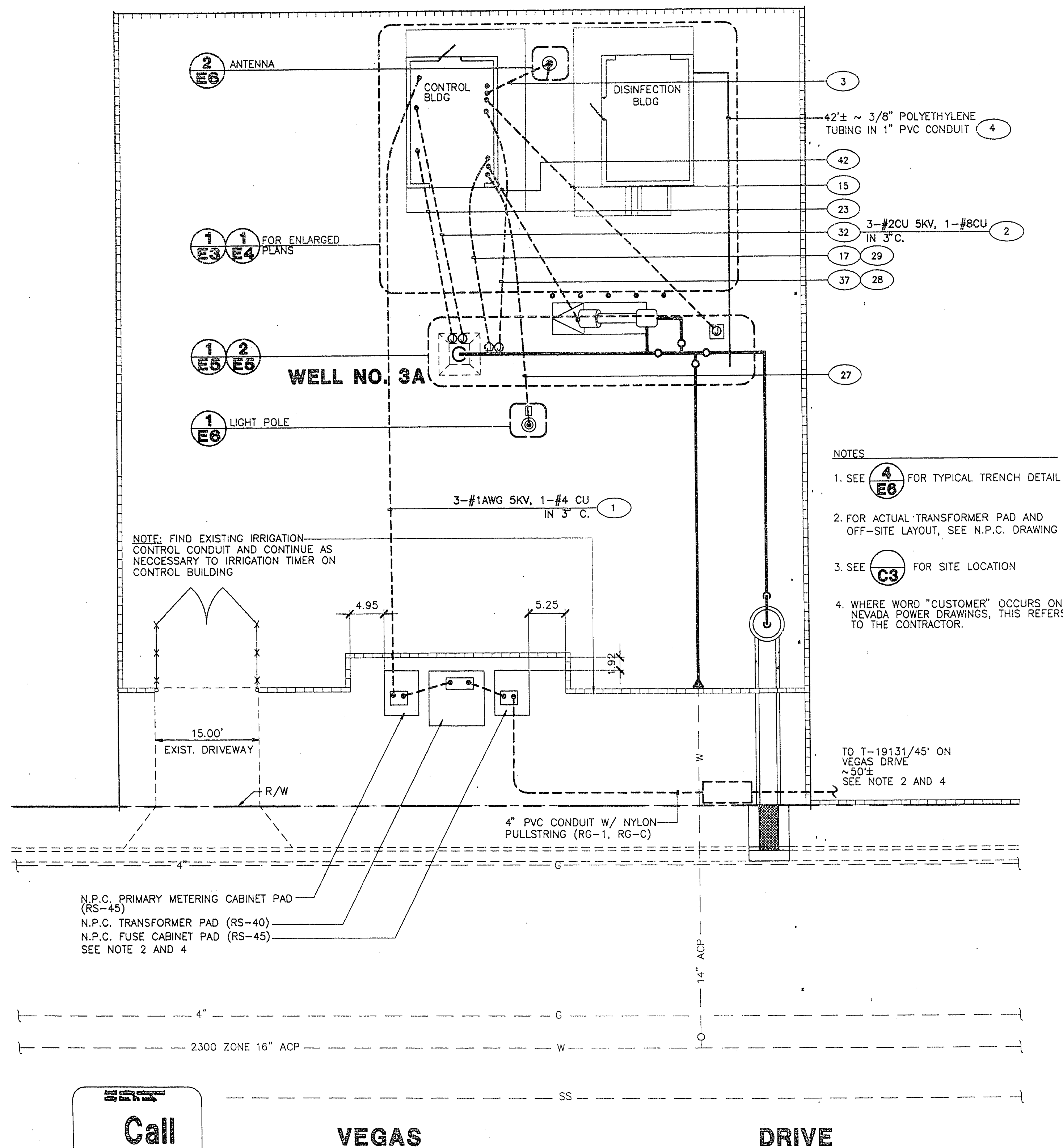
ELECTRICAL SITE PLAN 1 SCALE - NOTED
