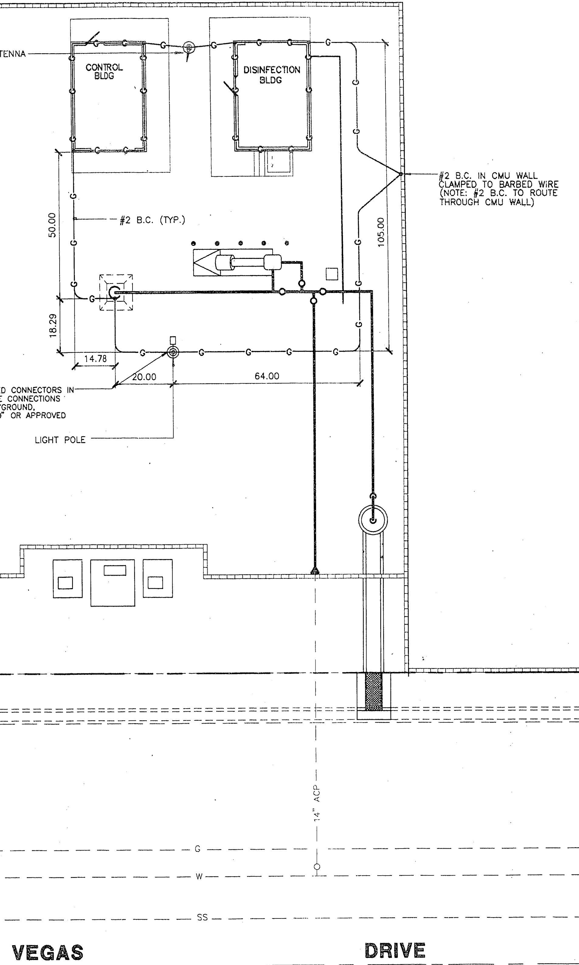
GROUNDING PLAN 2 SCALE - NOTED
