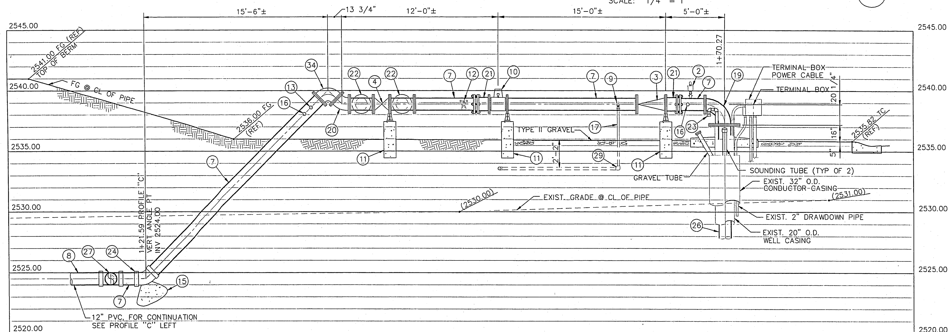
WELL NO. 95 DISCHARGE PIPING PROFILE A SCALE: 1/4" = 1'-0"
