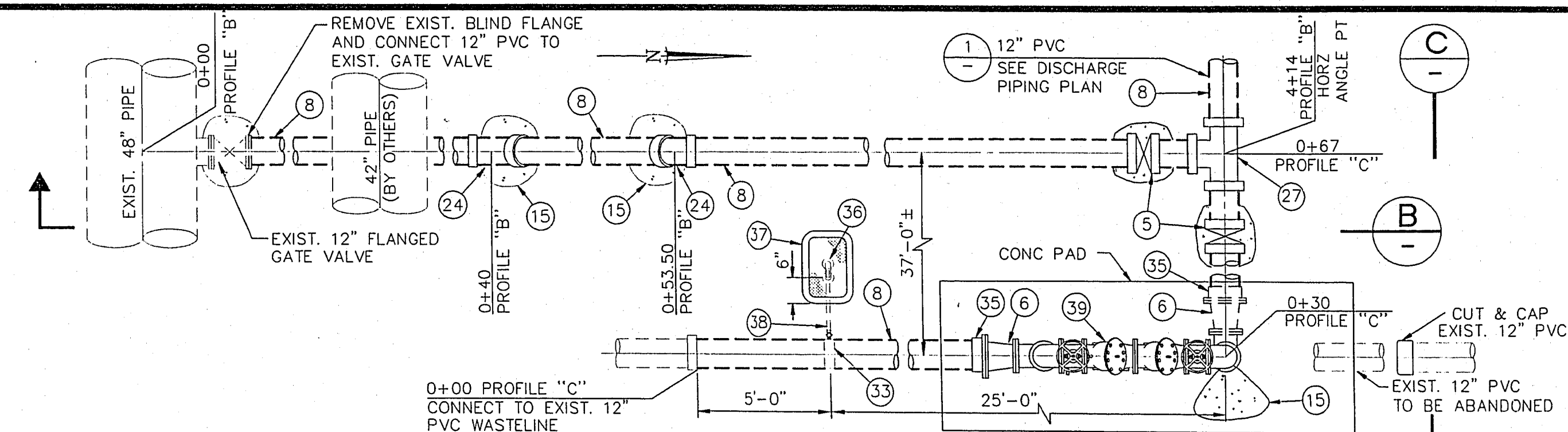
WELL NO. 95 DISCHARGE PIPING PLAN 2 SCALE: 1/4" = 1'
