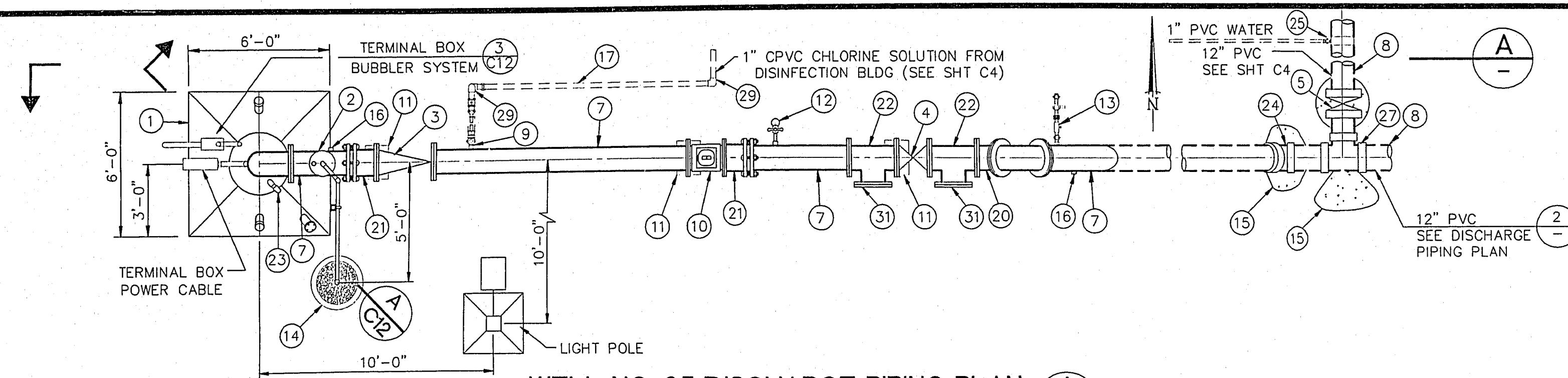
WELL NO. 95 DISCHARGE PIPING PLAN 1 SCALE: 1/4" = 1'
