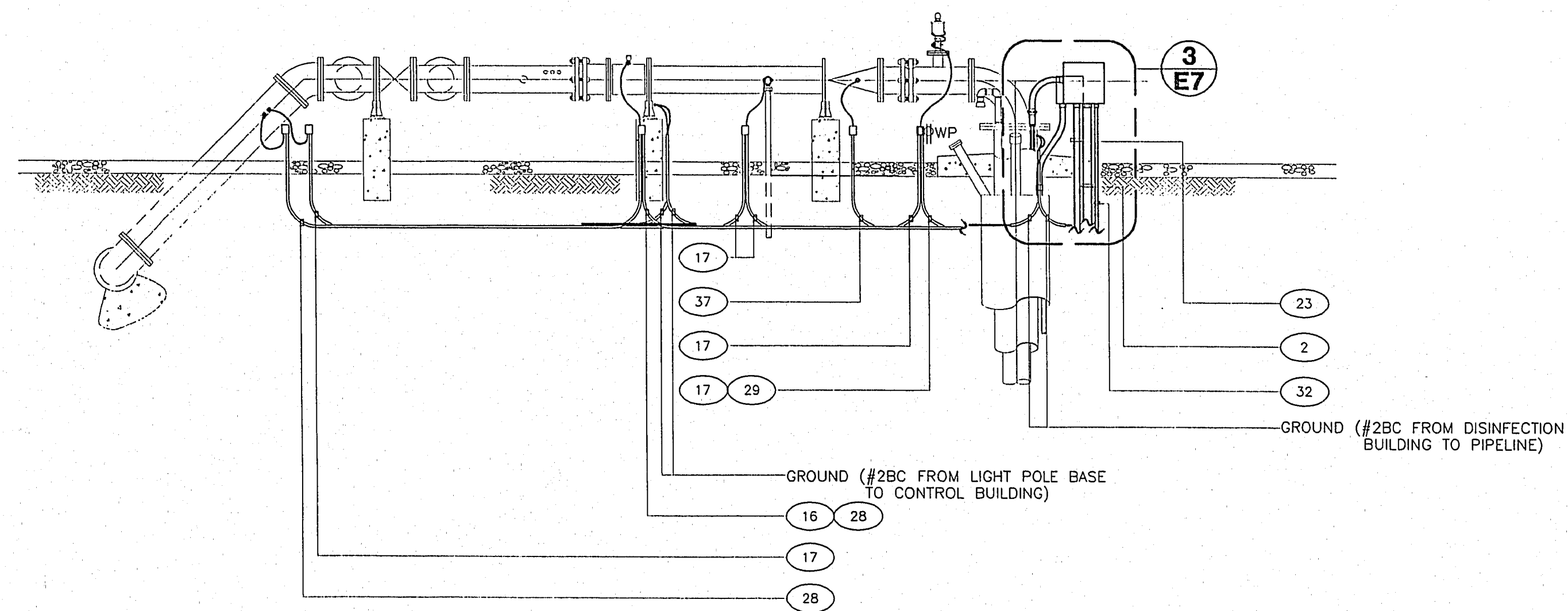
WELL No. 90 ELECTRICAL PROFILE 2 SCALE - 1/4" = 1'-0"
