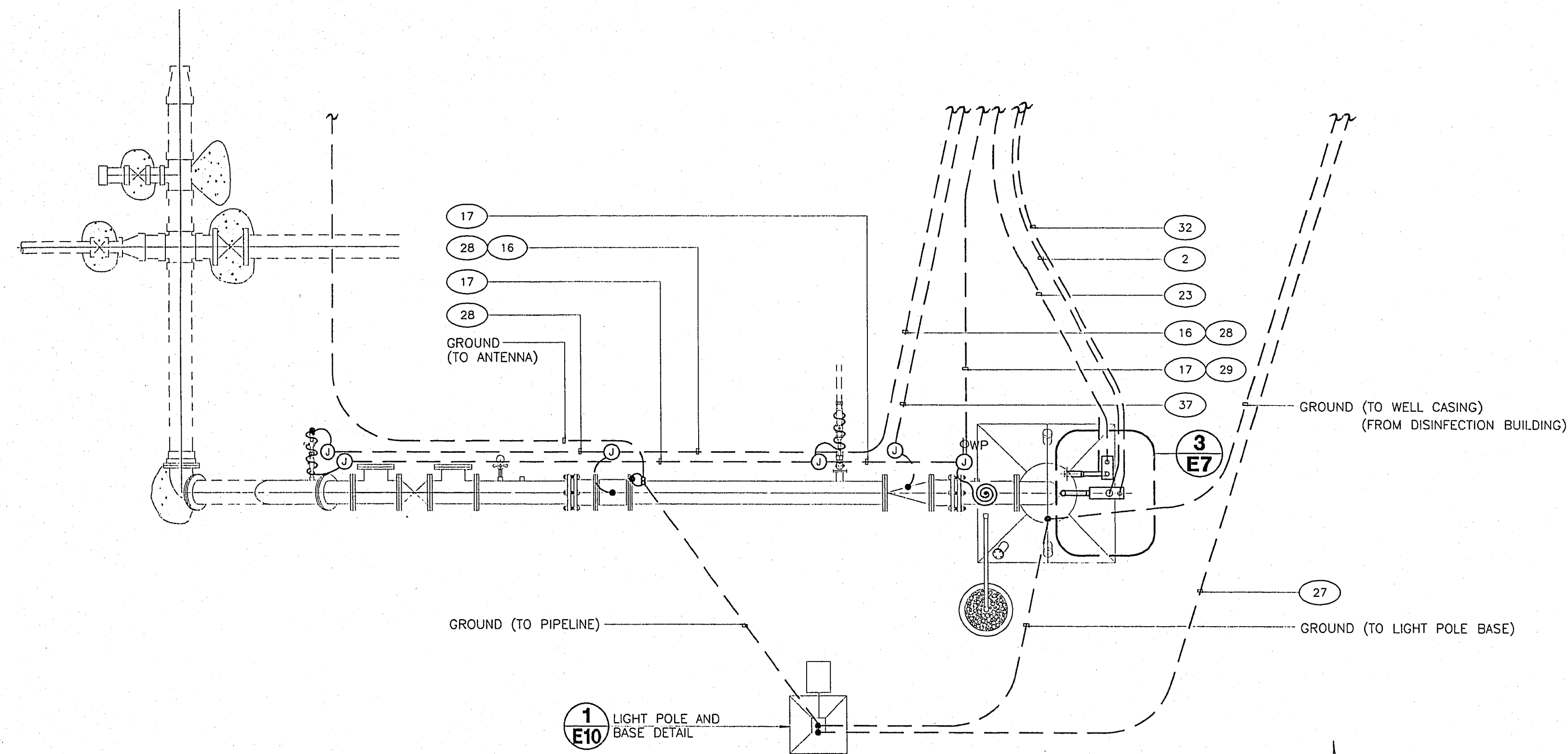
WELL No. 90 ELECTRICAL PLAN 1 SCALE - 1/4" = 1'-0"
