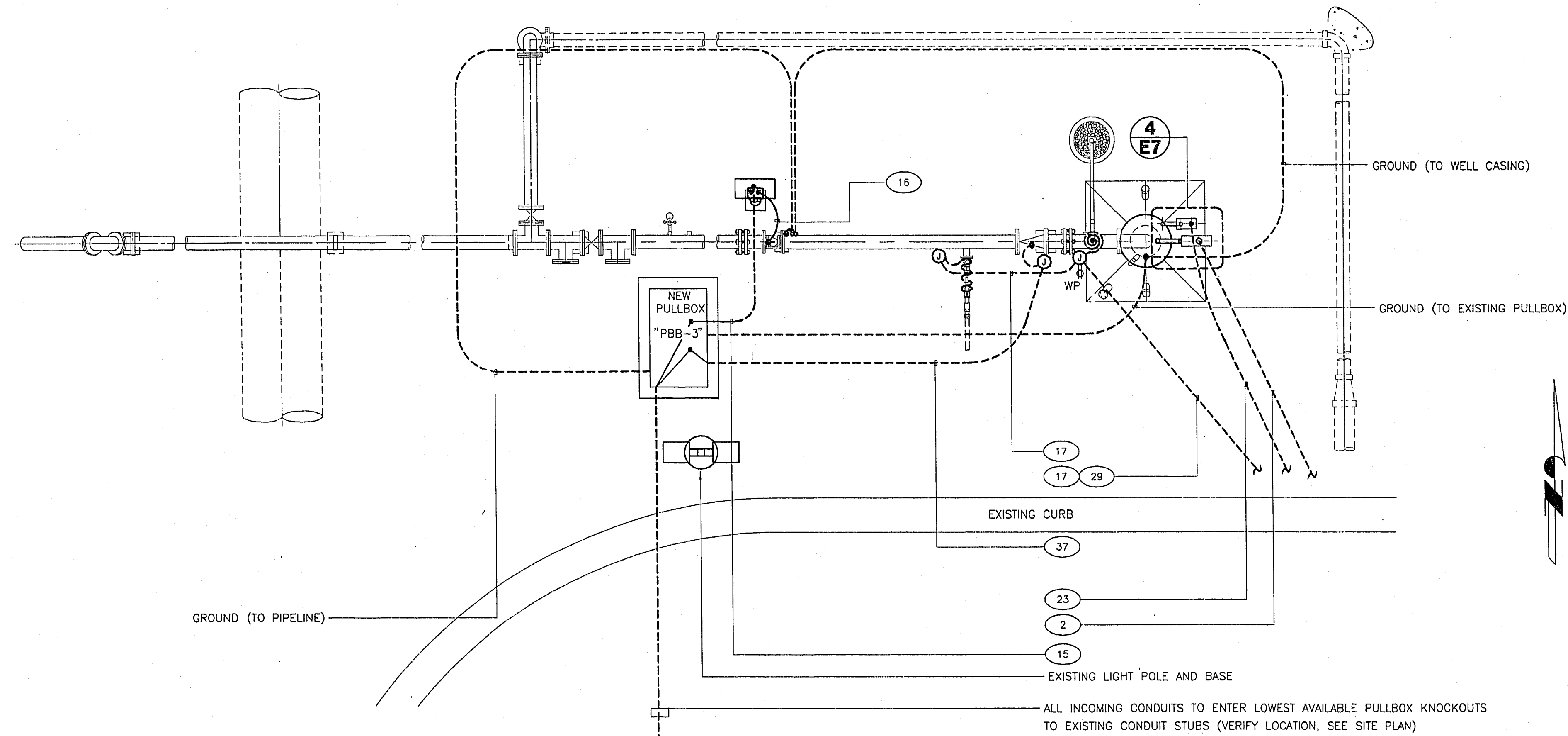
ELECTRICAL PLAN SCALE - 1/4" = 1'-0"
