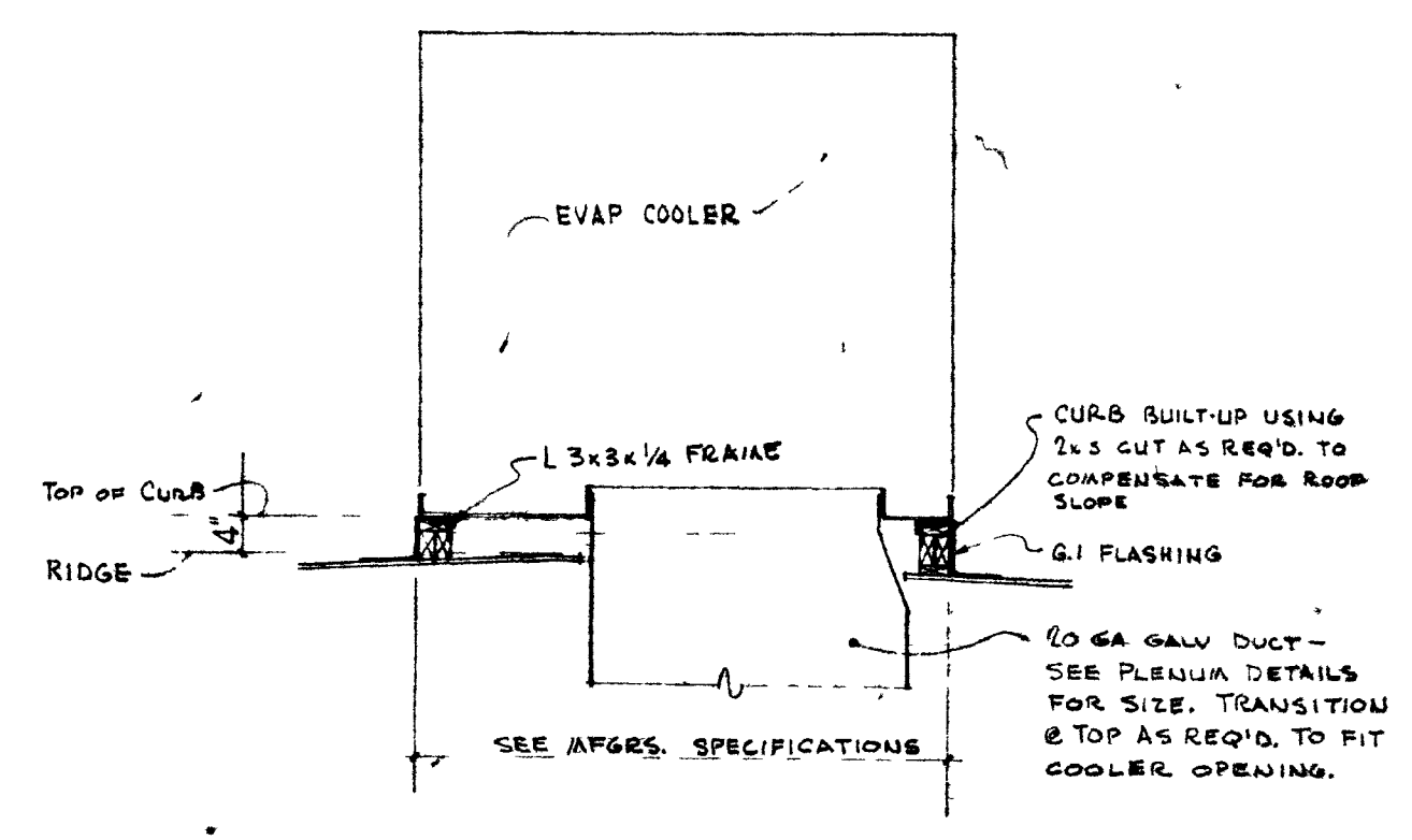
DETAIL C SCALE 1/4" = 1'-0"
