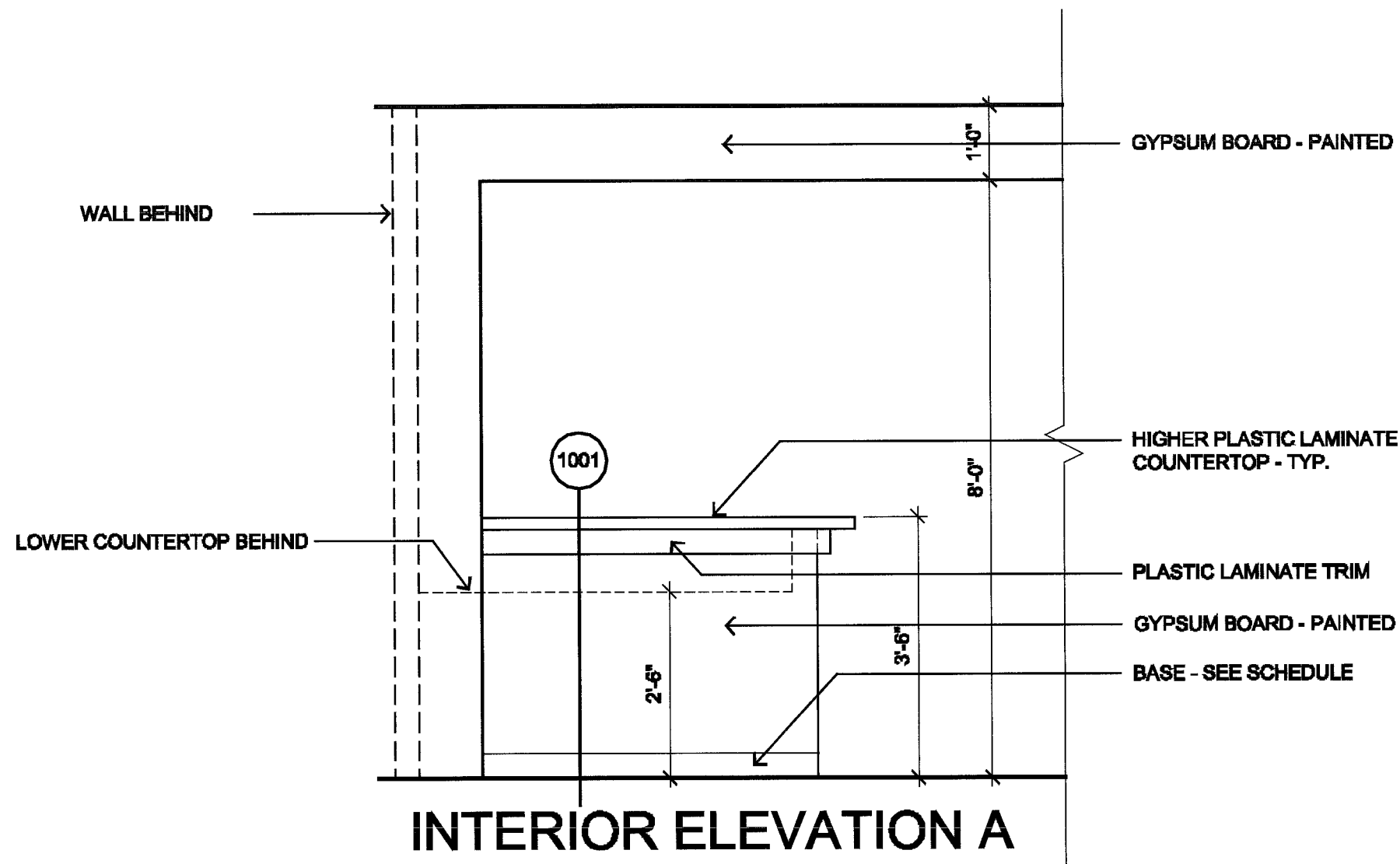
120 LAB 1/2"=1'-0"
