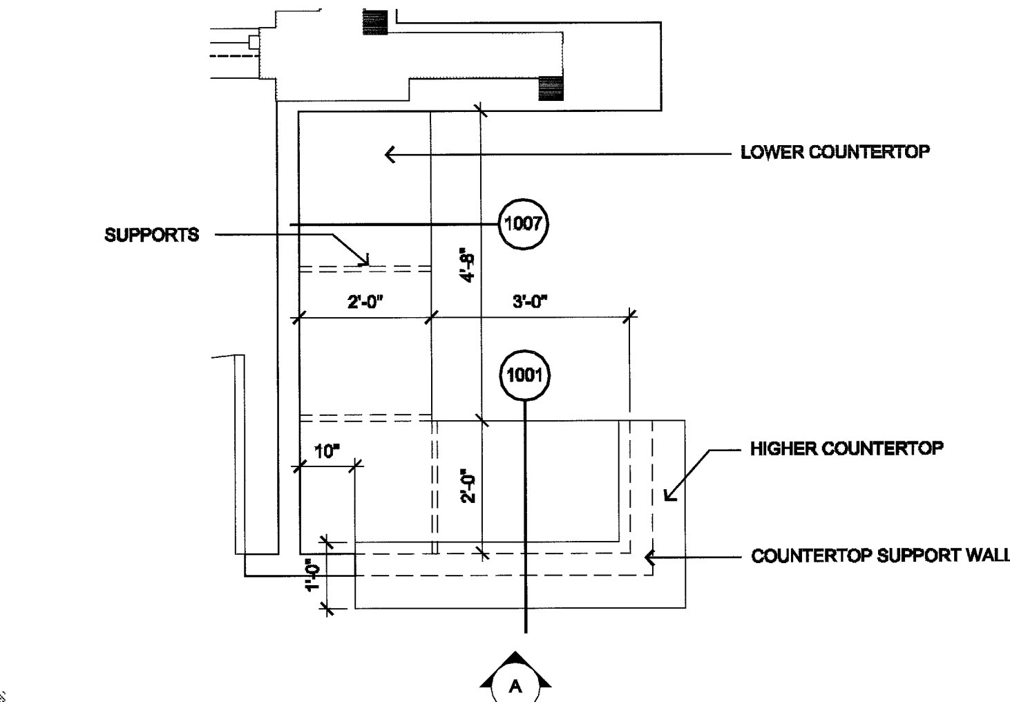
122 NURSE STATION 1/2"=1'-0"
