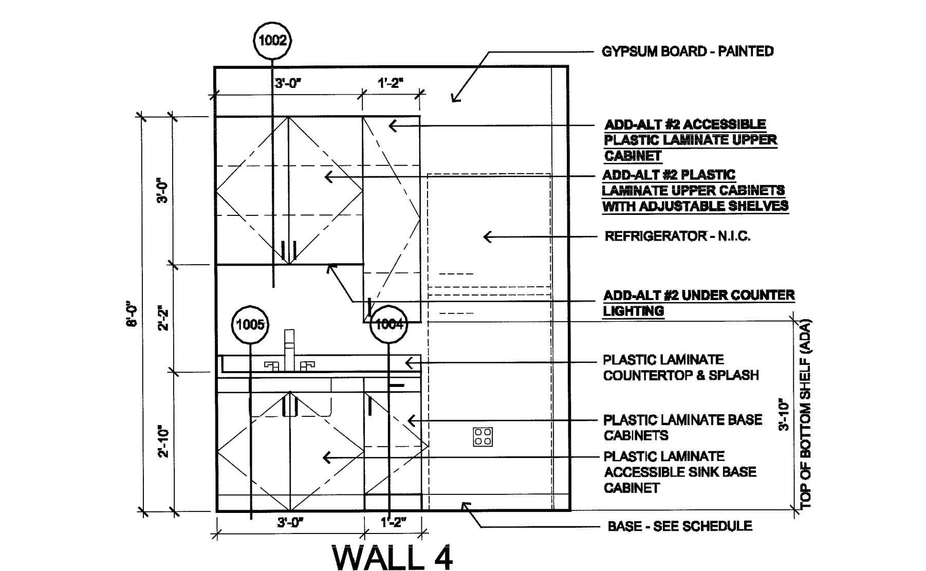
123 BREAK ROOM 1/2"=1'-0"
