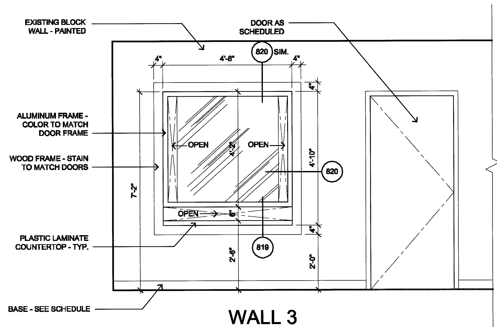
100 LOBBY 1 1/2"=1'-0"
