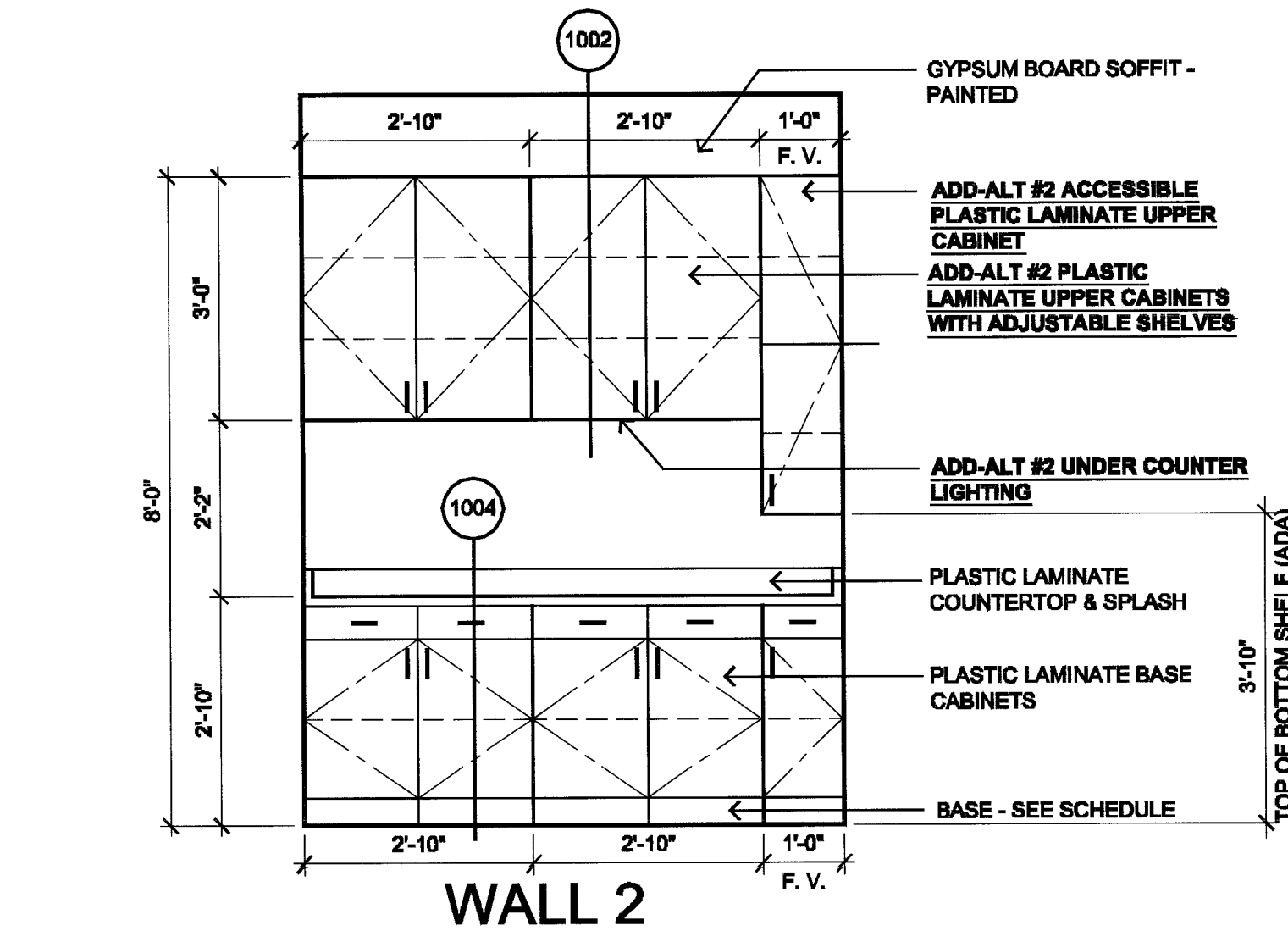
121 HALLWAY 3 1/2"=1'-0"
