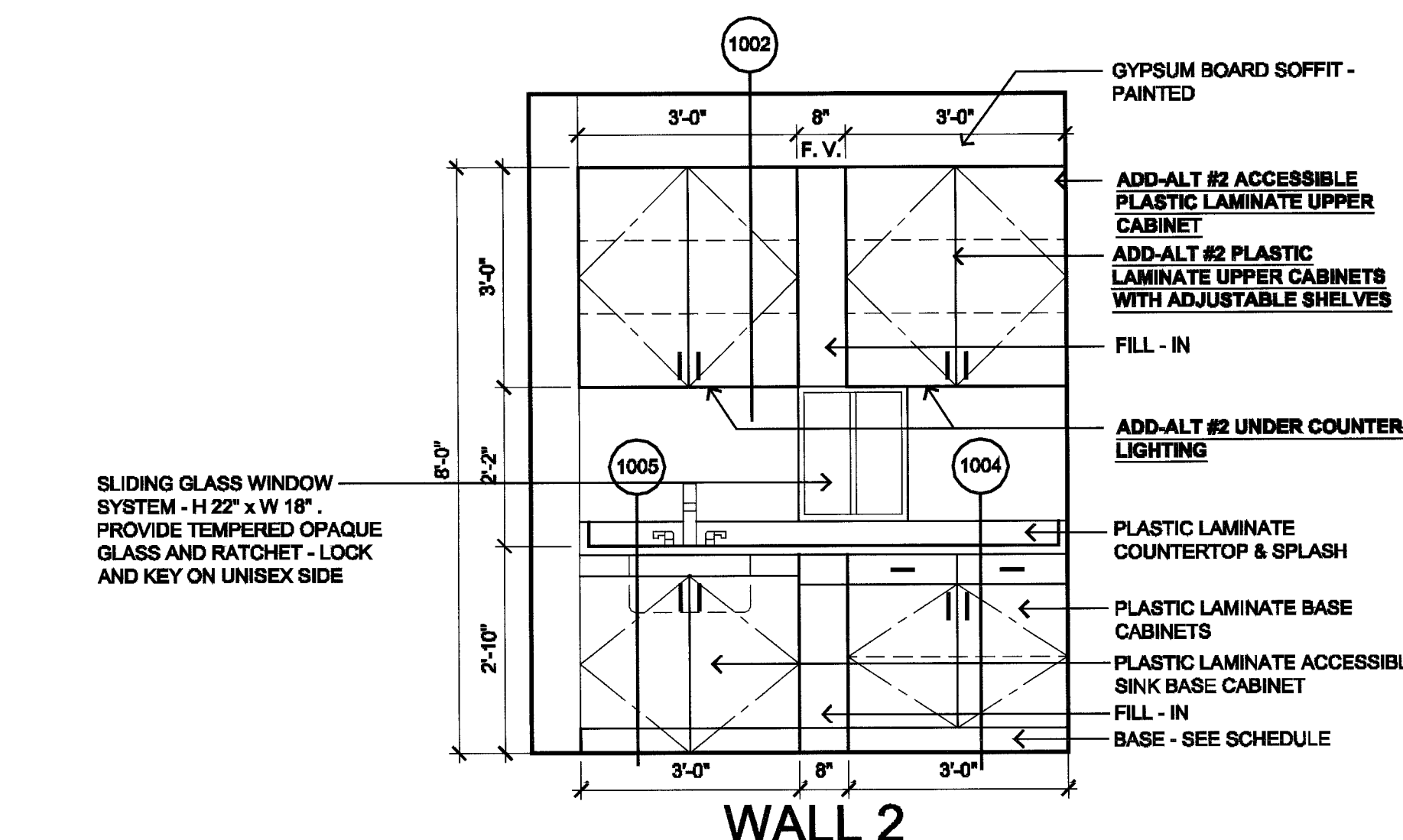
120 LAB 1/2"=1'-0"
