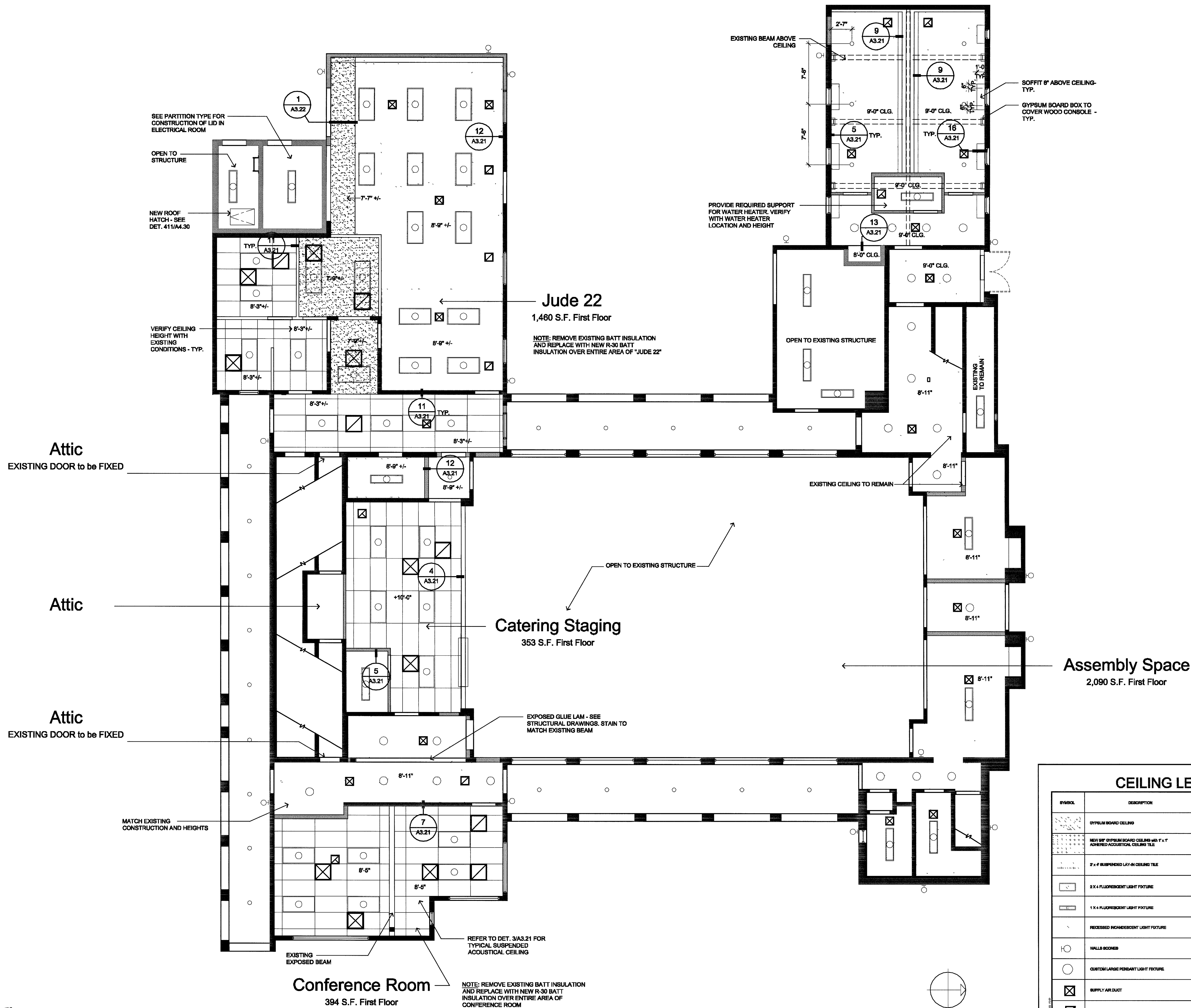
95873 BUILDING 3 - FIRST FLOOR - REFLECTED CEILING PLAN 3/16\"/>
