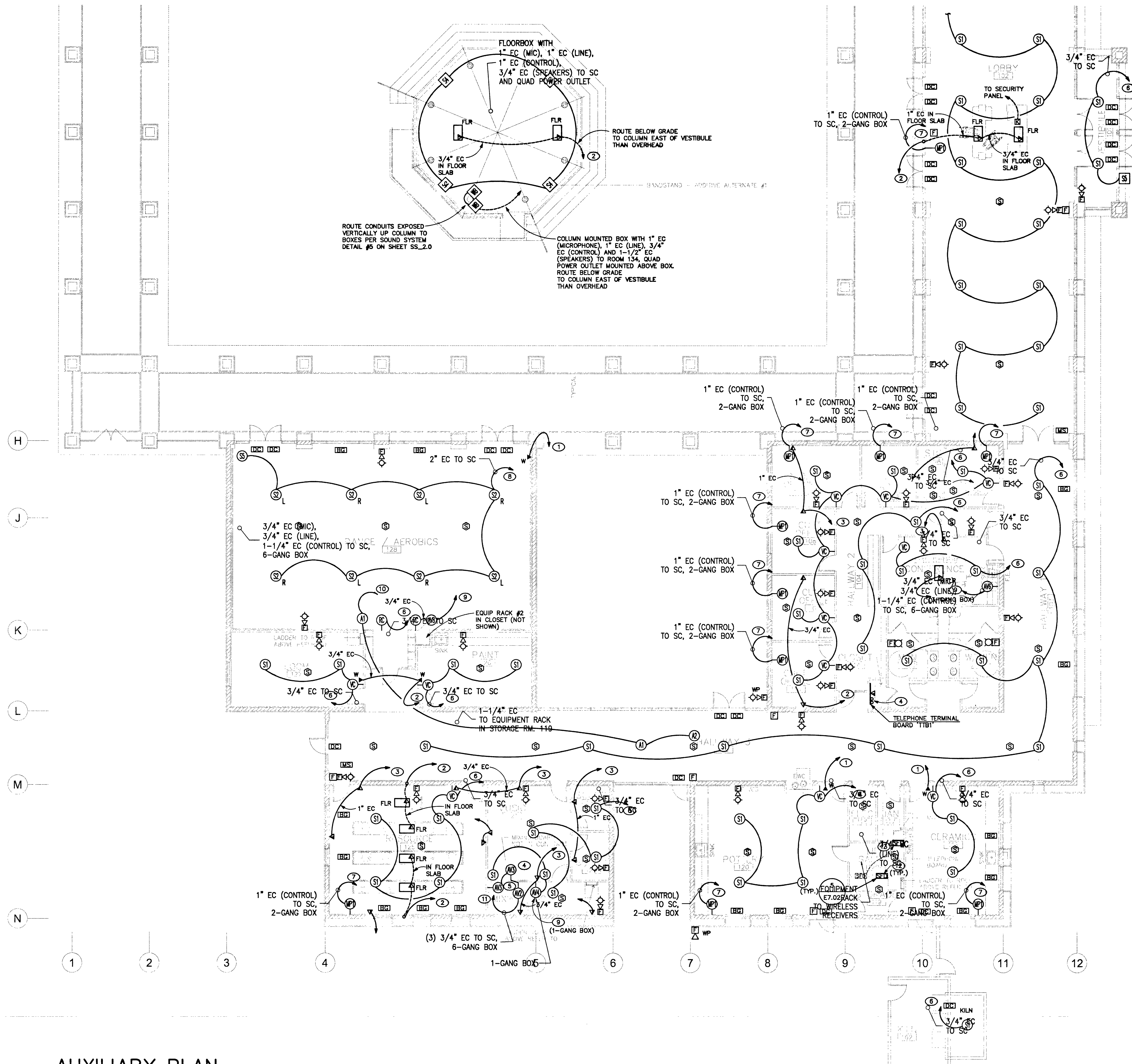
AUXILIARY PLAN SCALE: 1/8" = 1' - 0"
