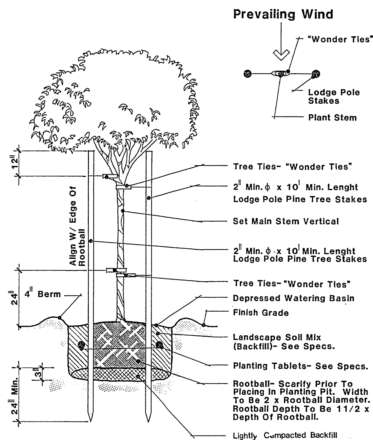
7 Tree Planting Detail
