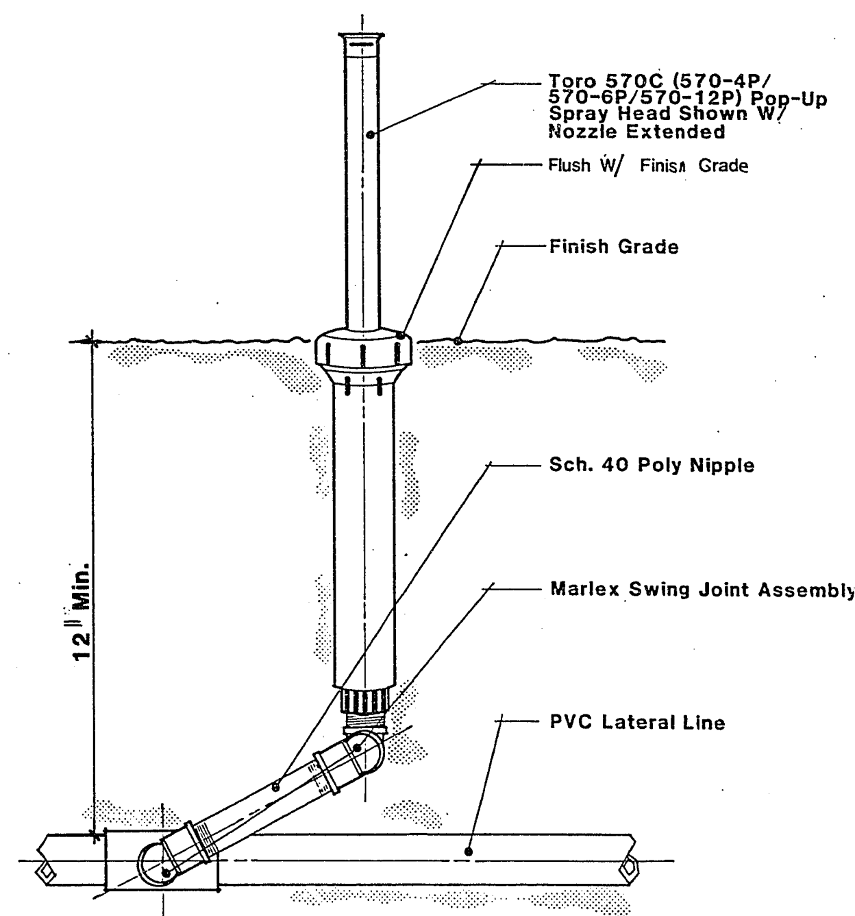
8 Toro 570C Pop-Up Spray Head
