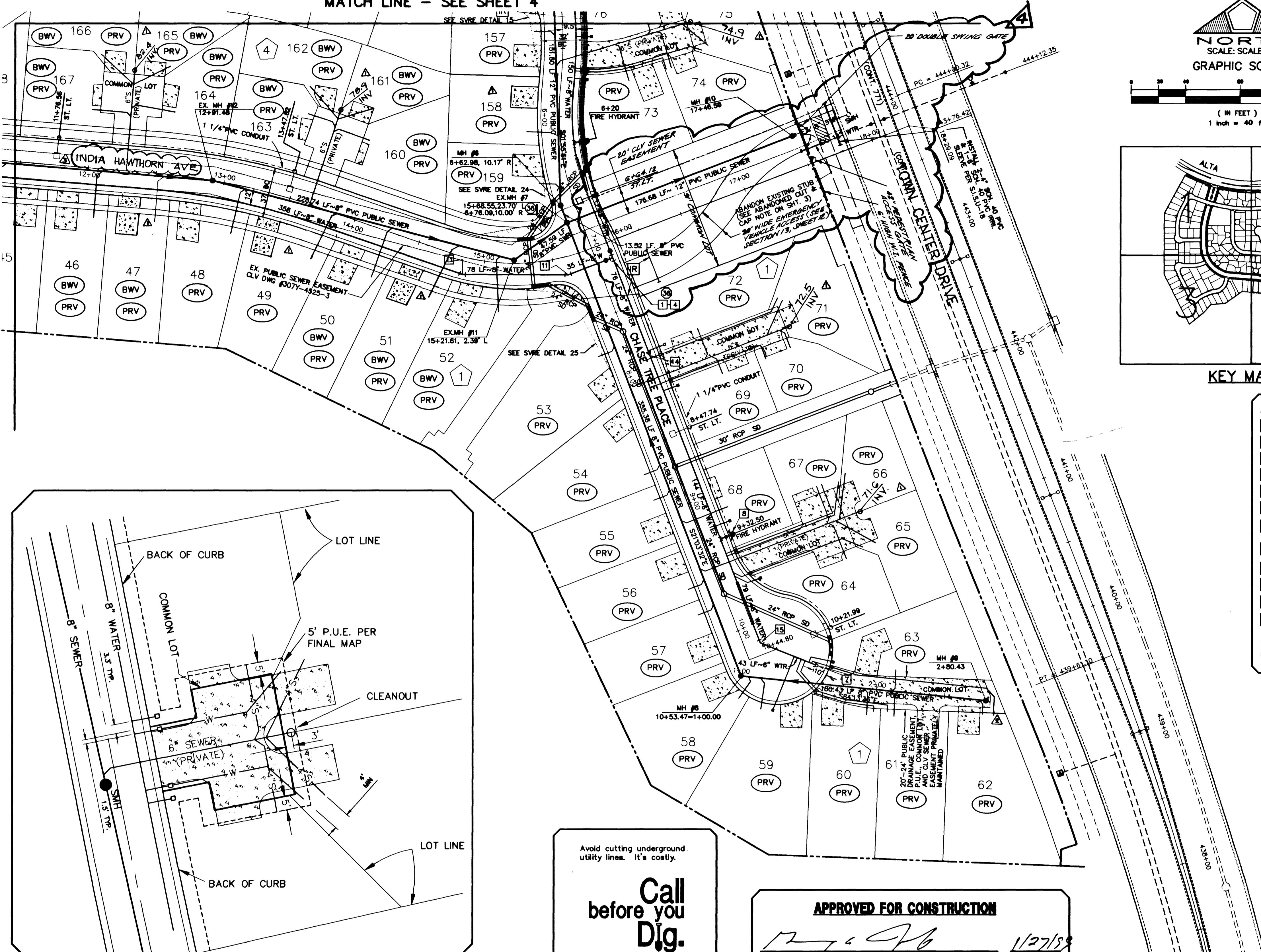
TYPICAL WATER AND SEWER LATERAL - CLUSTER HOMES SCALE: 1"=20'
