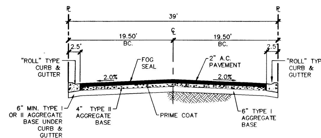
TYPICAL 39' PRIVATE STREET SECTION N.T.S. (PRIVATE STREET)
