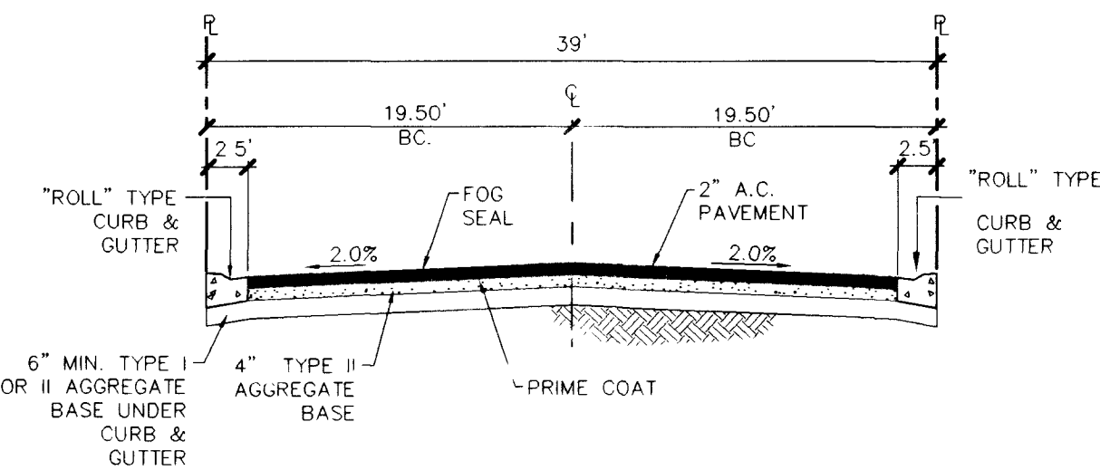
TYPICAL 39' PRIVATE STREET SECTION
