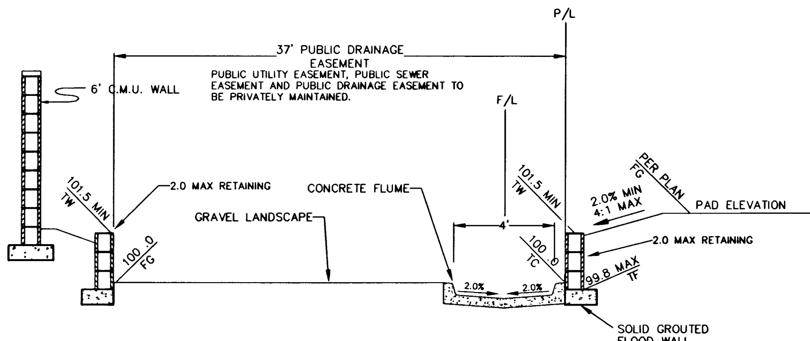
PUBLIC UTILITY EASEMENT, PUBLIC SEWER EASEMENT AND PUBLIC DRAINAGE EASEMENT TO BE PRIVATELY MAINTAINED. DETAIL B
