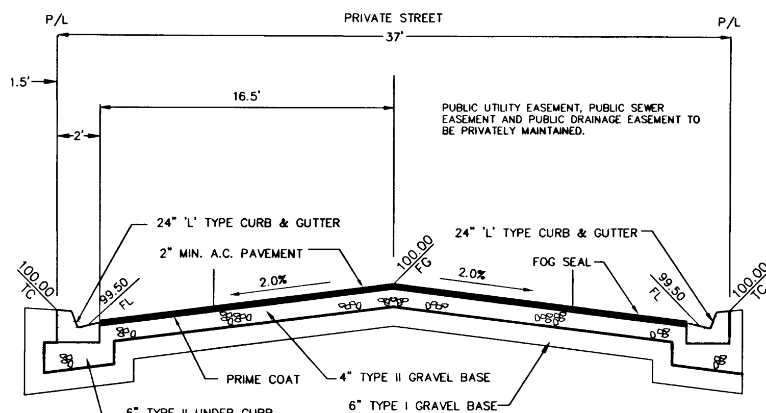
SECTION G - C/L CROWN - INTERIOR STREET (TYP.) - PRIVATE
