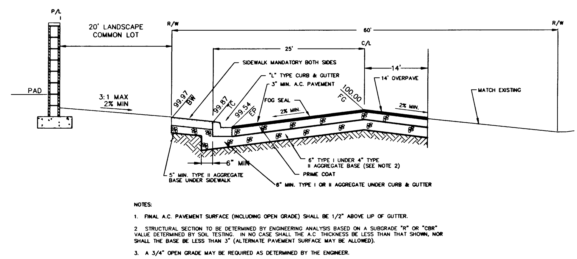
60' ROW SECTION DETAIL SECTION F - THOM BLVD.
