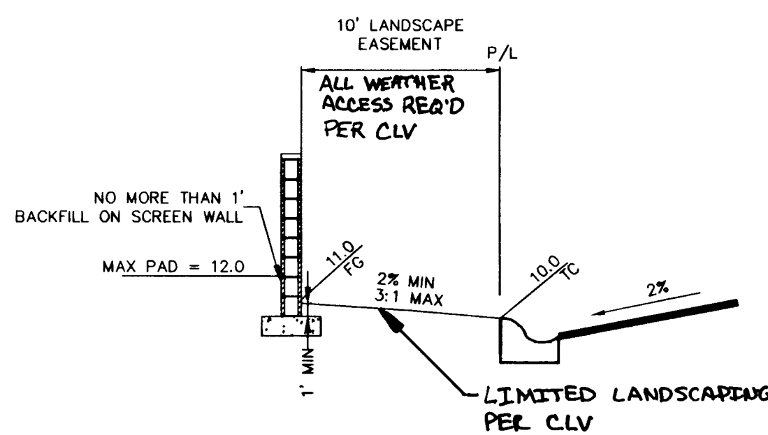
SECTION D - CORNER LANDSCAPE EASEMENT
