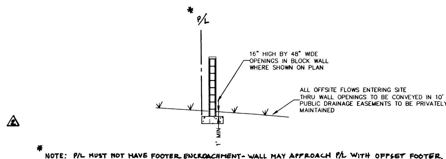
SECTION E - WEST P/L (TYP)
