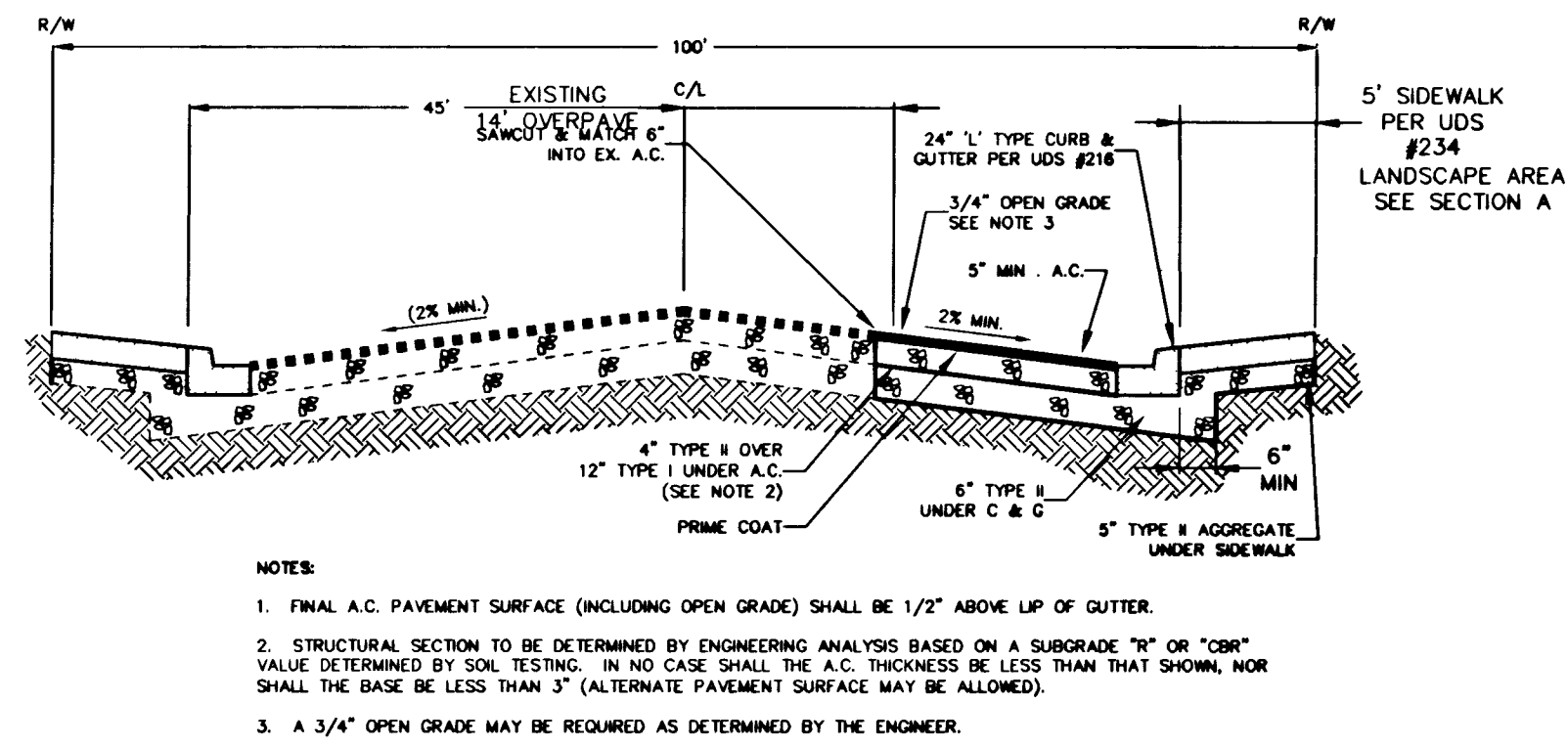
100' ROW SECTION DETAIL SECTION N - ELKHORN ROAD SECTION
