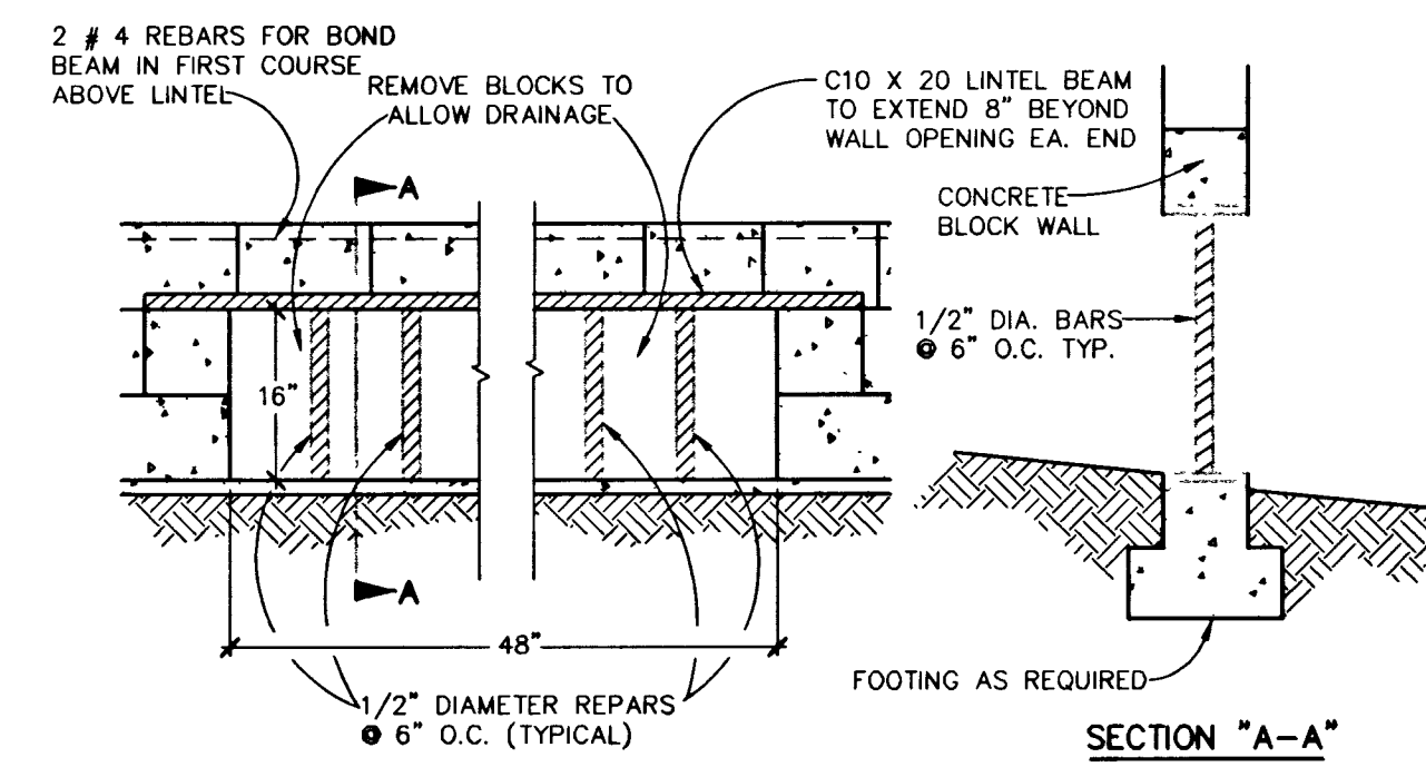
BLOCK WALL OPENING DETAIL SCALE: NONE
