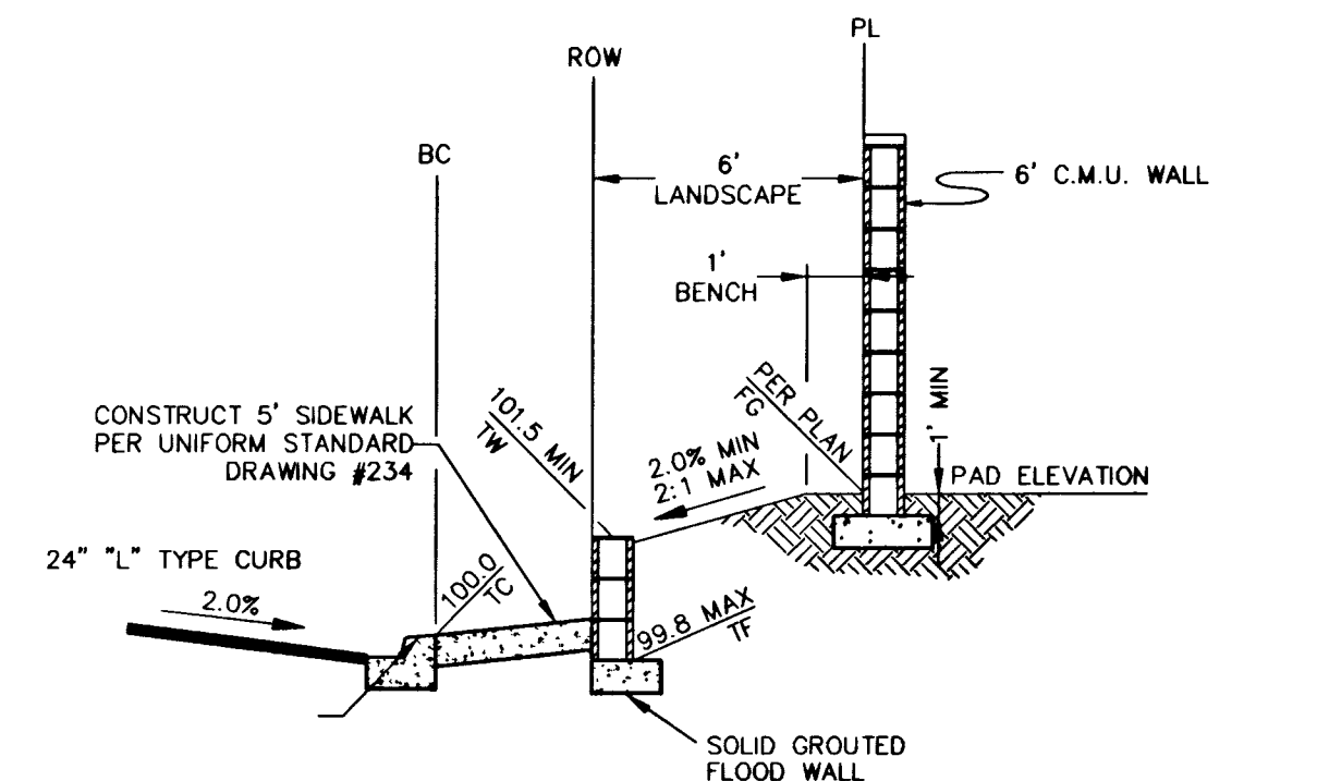
COMMON LOT SECTION A FLOOD PROTECTION WALL DETAIL
