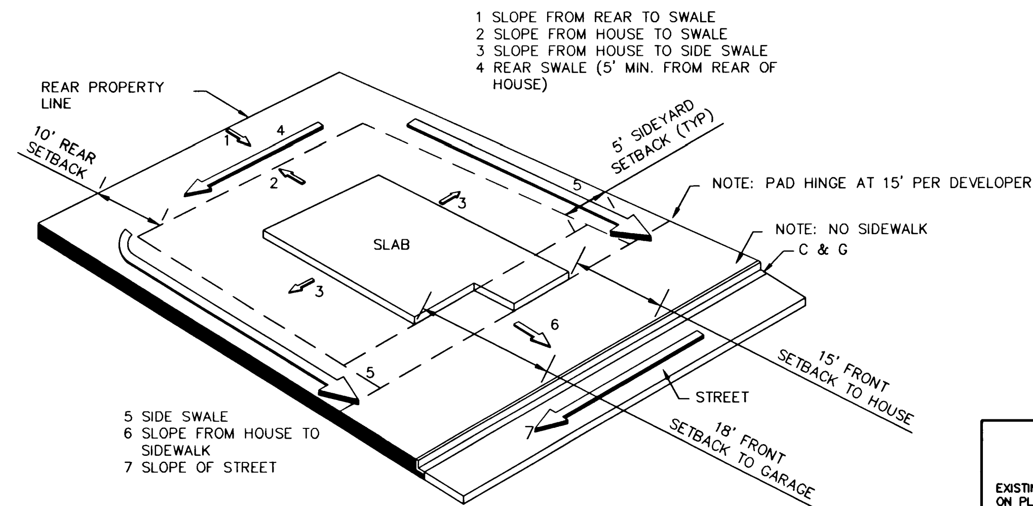
F.H.A. TYPE "A" DRAINAGE W/ SETBACKS + HINGE LINES NTS
