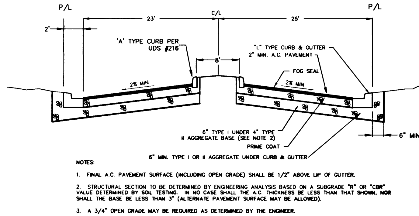
PRIVATE ENTRY STREET SECTION DETAIL SECTION H - DIAMOND STREAM LANE
