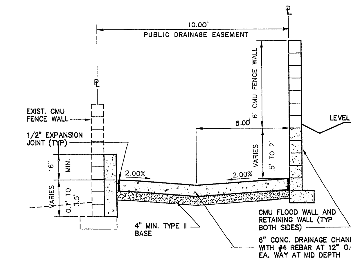
SYR 8 CONCRETE CHANNEL DETAIL SCALE: NO SCALE
