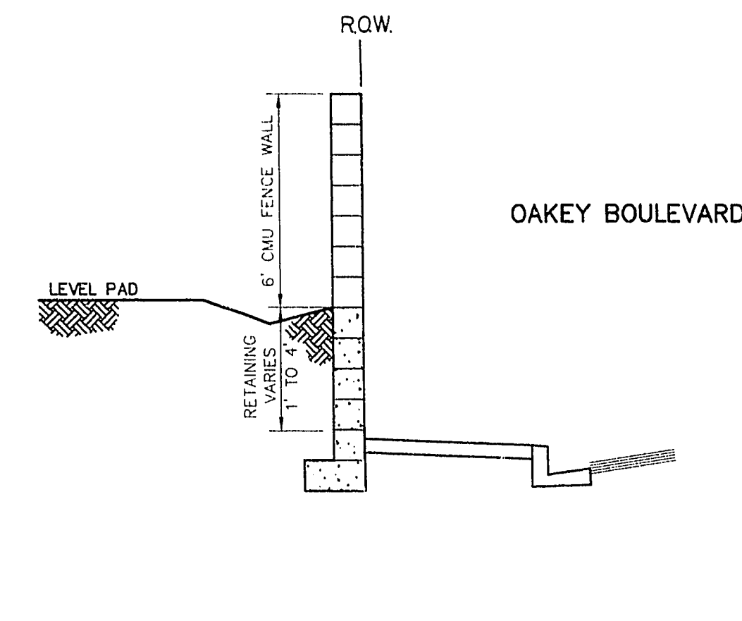
CCD4 5 CORNER SIDE YARD WITH RETAINING DETAIL SCALE: NO SCALE
