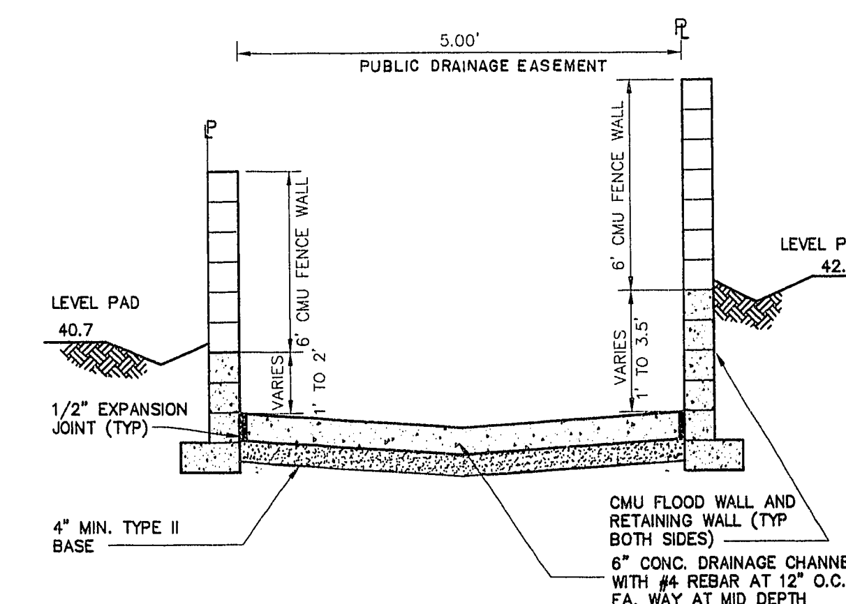
RWCS (3) CONCRETE CHANNEL DETAIL SCALE: NO SCALE
