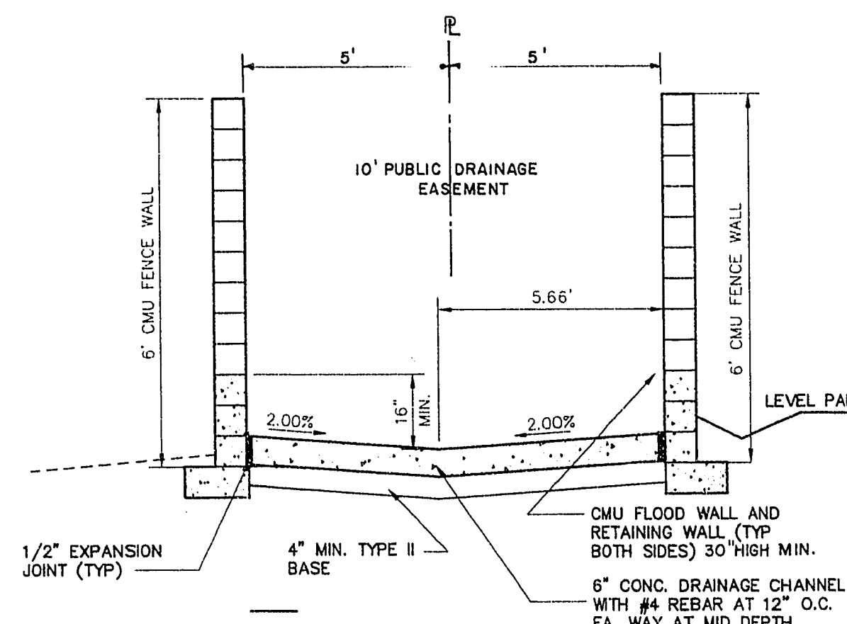
9 CONCRETE CHANNEL DETAIL SCALE: NO SCALE
