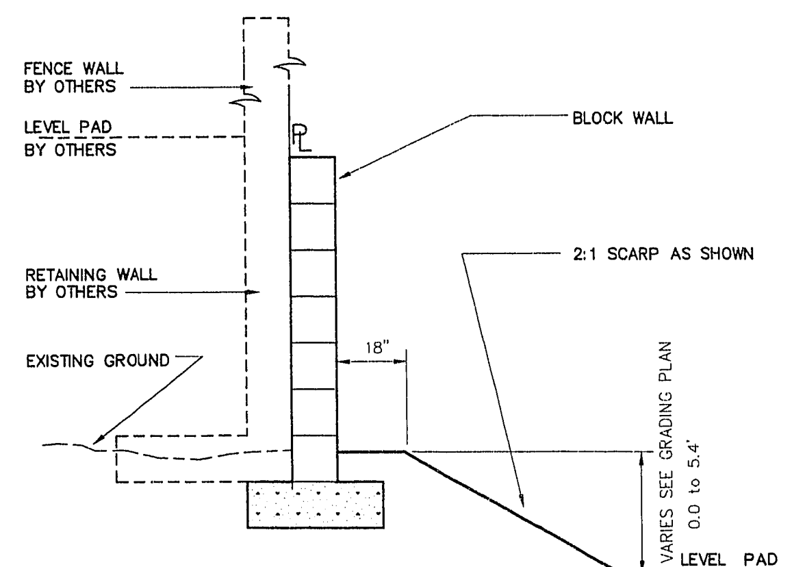
10 REAR YARD DETAIL SCALE: NO SCALE
