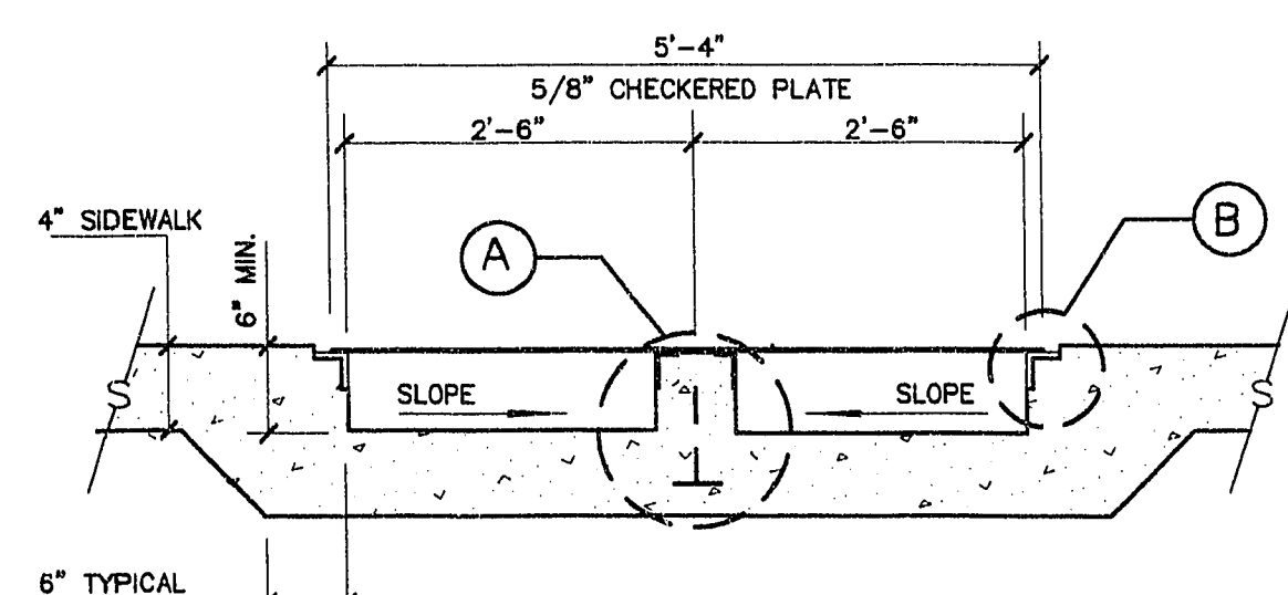
13 SIDEWALK UNDERDRAIN DETAIL SCALE: NO SCALE
