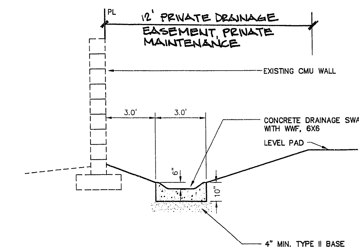
11 TYPICAL CONCRETE SWALE DETAIL SCALE: NO SCALE
