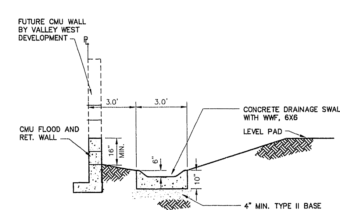
TUC 2 CONCRETE CHANNEL DETAIL SCALE: NO SCALE
