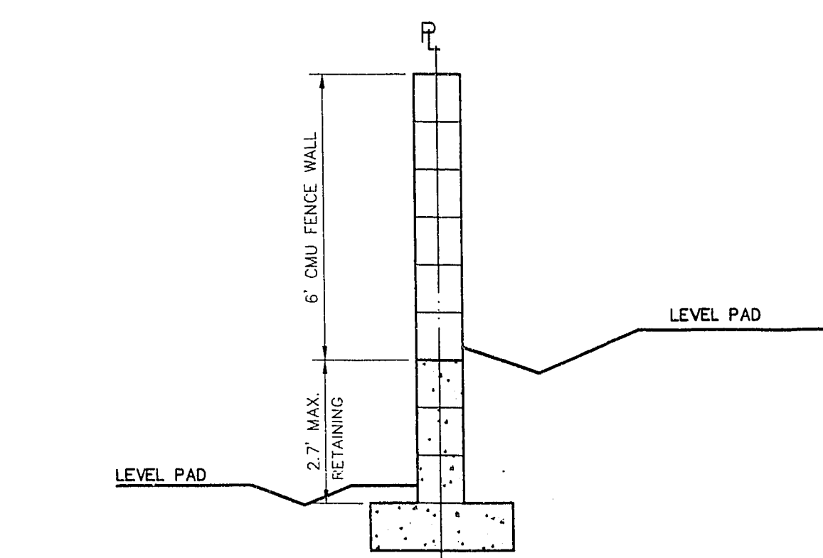
12 SIDE YARD RETAINING DETAIL SCALE: NO SCALE
