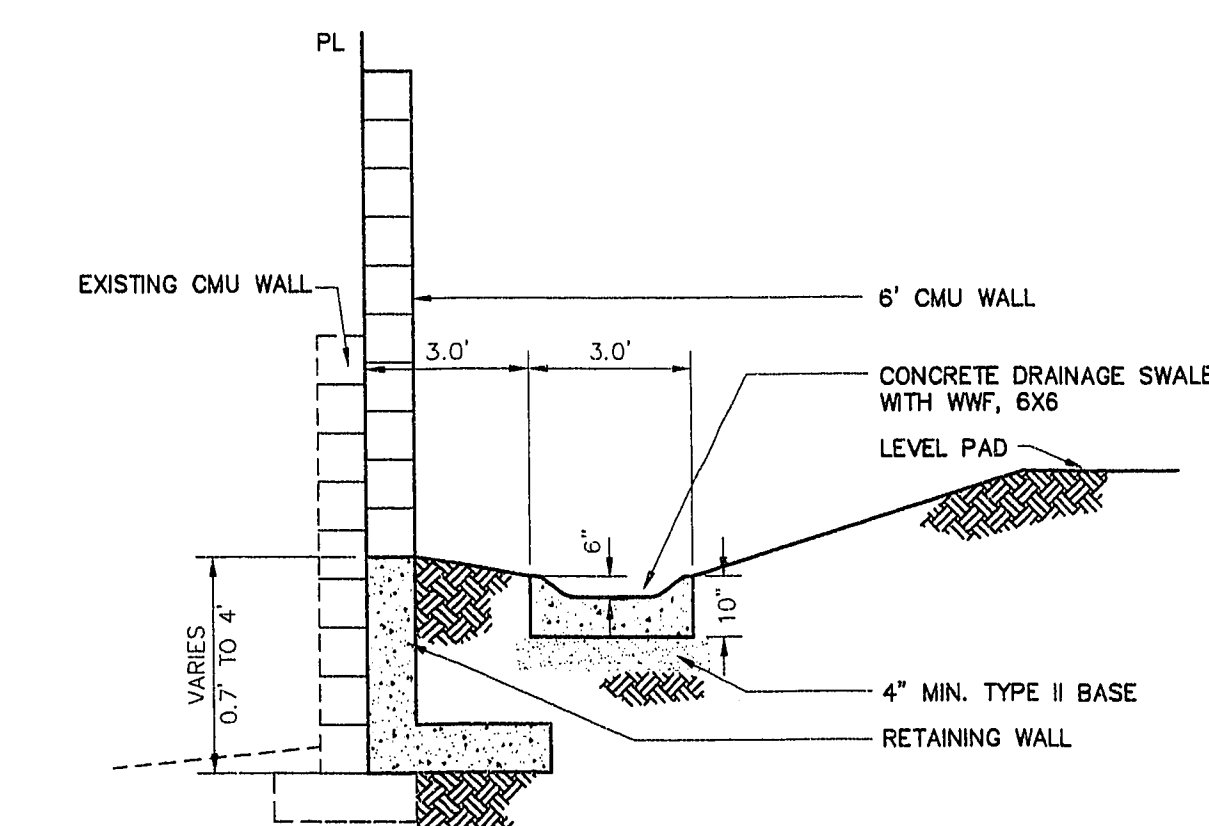
CSWALE 7 RETAINING WALL AND CONCRETE SWALE DETAIL SCALE: NO SCALE
