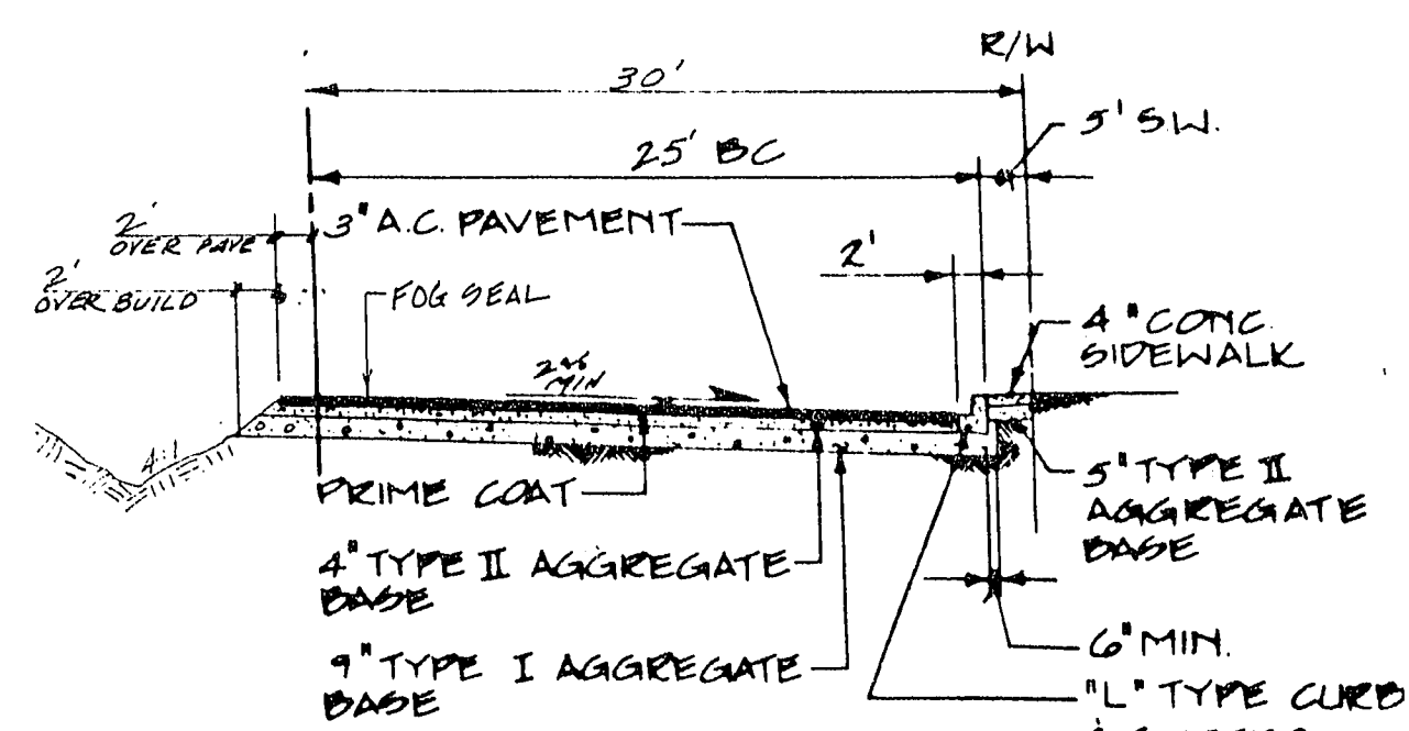
TYPICAL STREET SECTION
