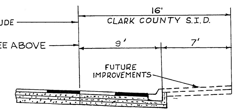
STA. 39+62± TO LAKE MEAD (EAST SIDE)
