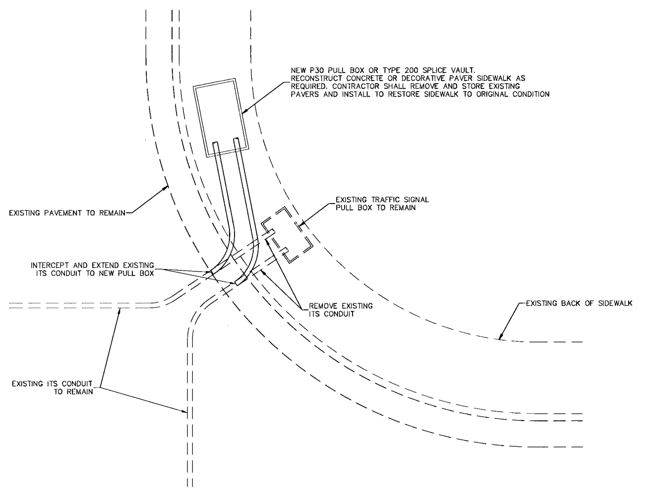
DETAIL B
