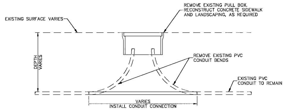
PROFILE
