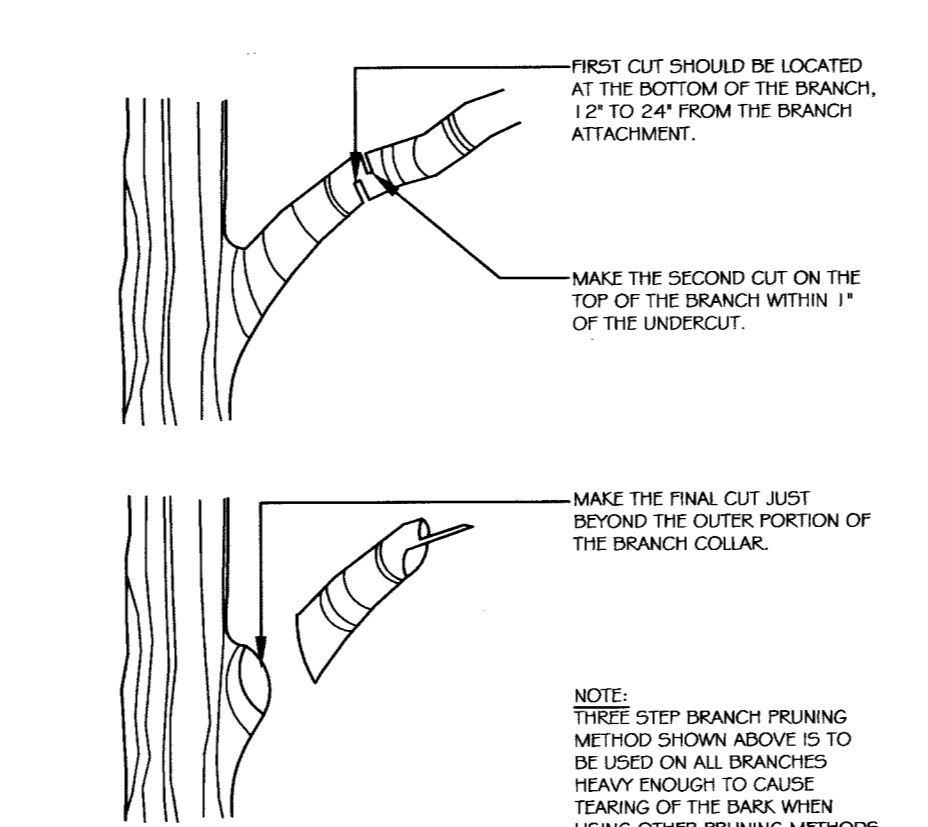
I TREE BRANCH PRUNING DETAIL
