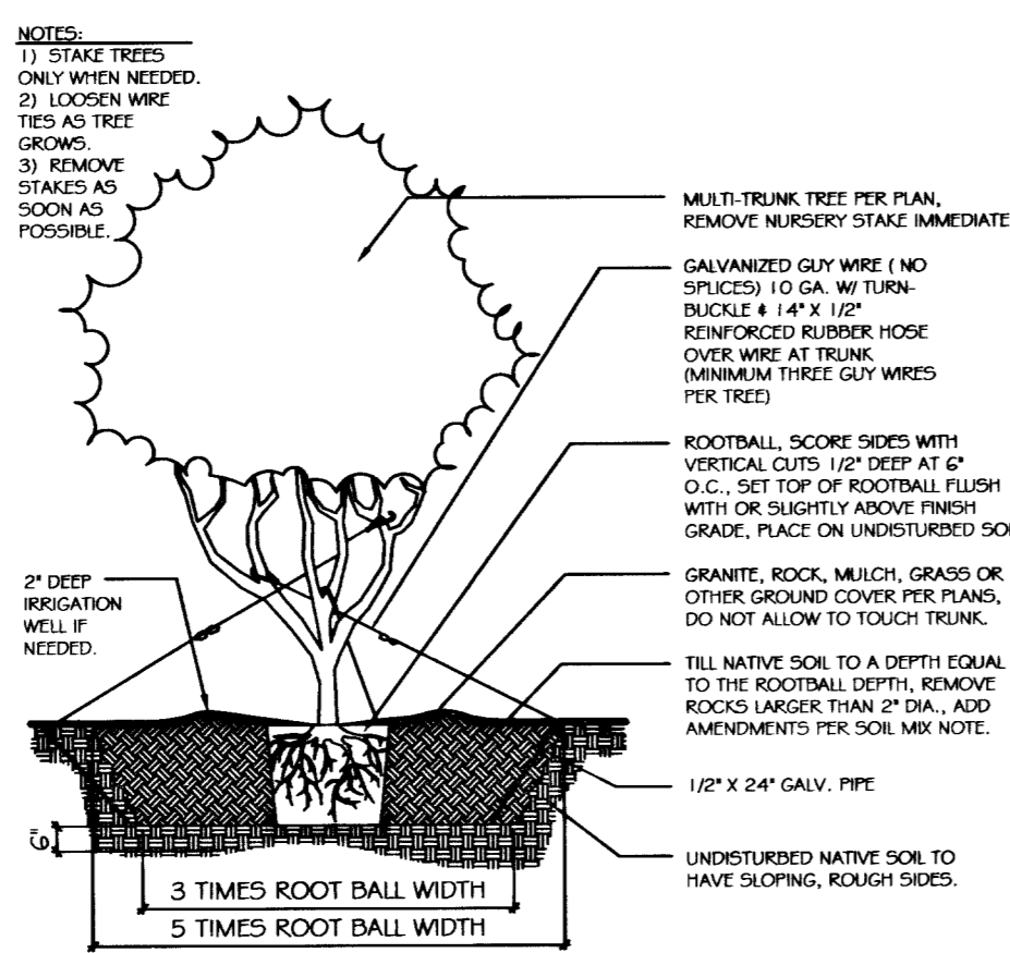
B MULTI-TRUNK PLANTING DETAIL
