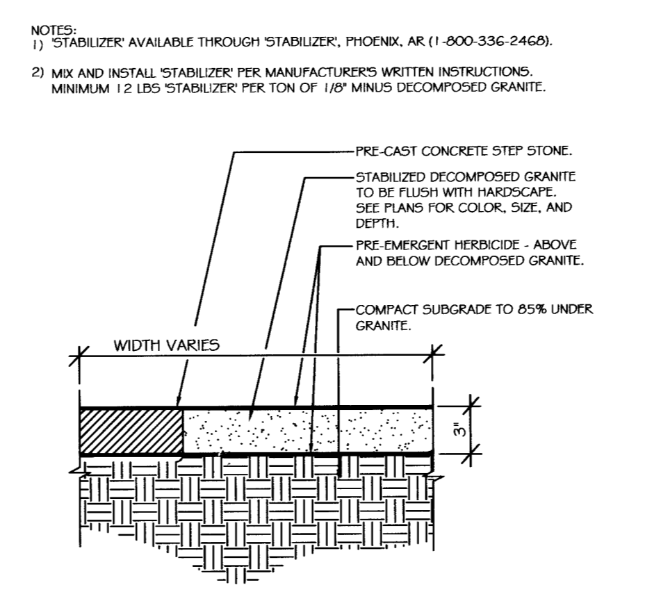
N STABILIZED DECOMPOSED GRANITE
