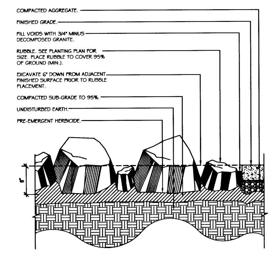
K RUBBLE DETAIL
