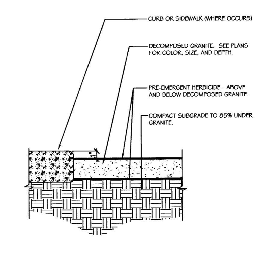
E DECOMPOSED GRANITE DETAIL
