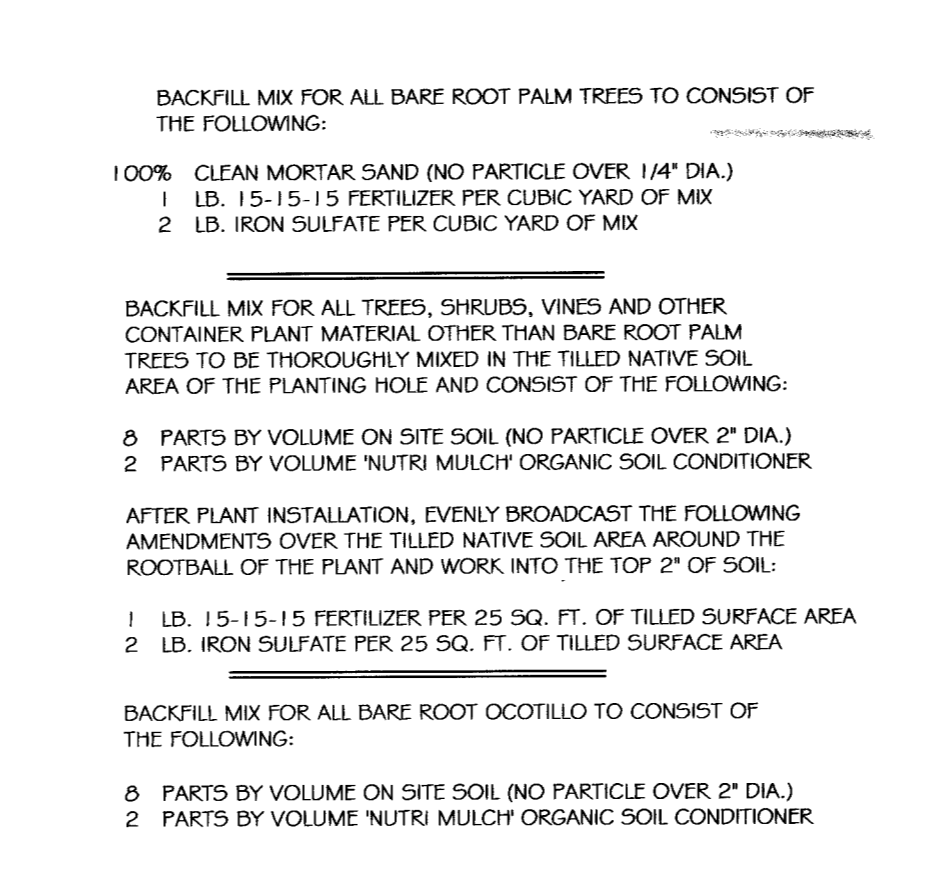
D SOIL MIX NOTE
