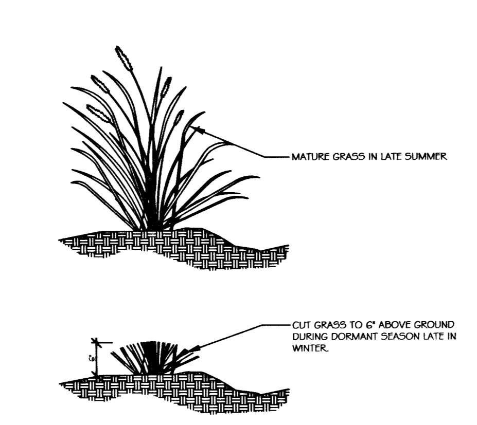
G GRASS PRUNING DETAIL
