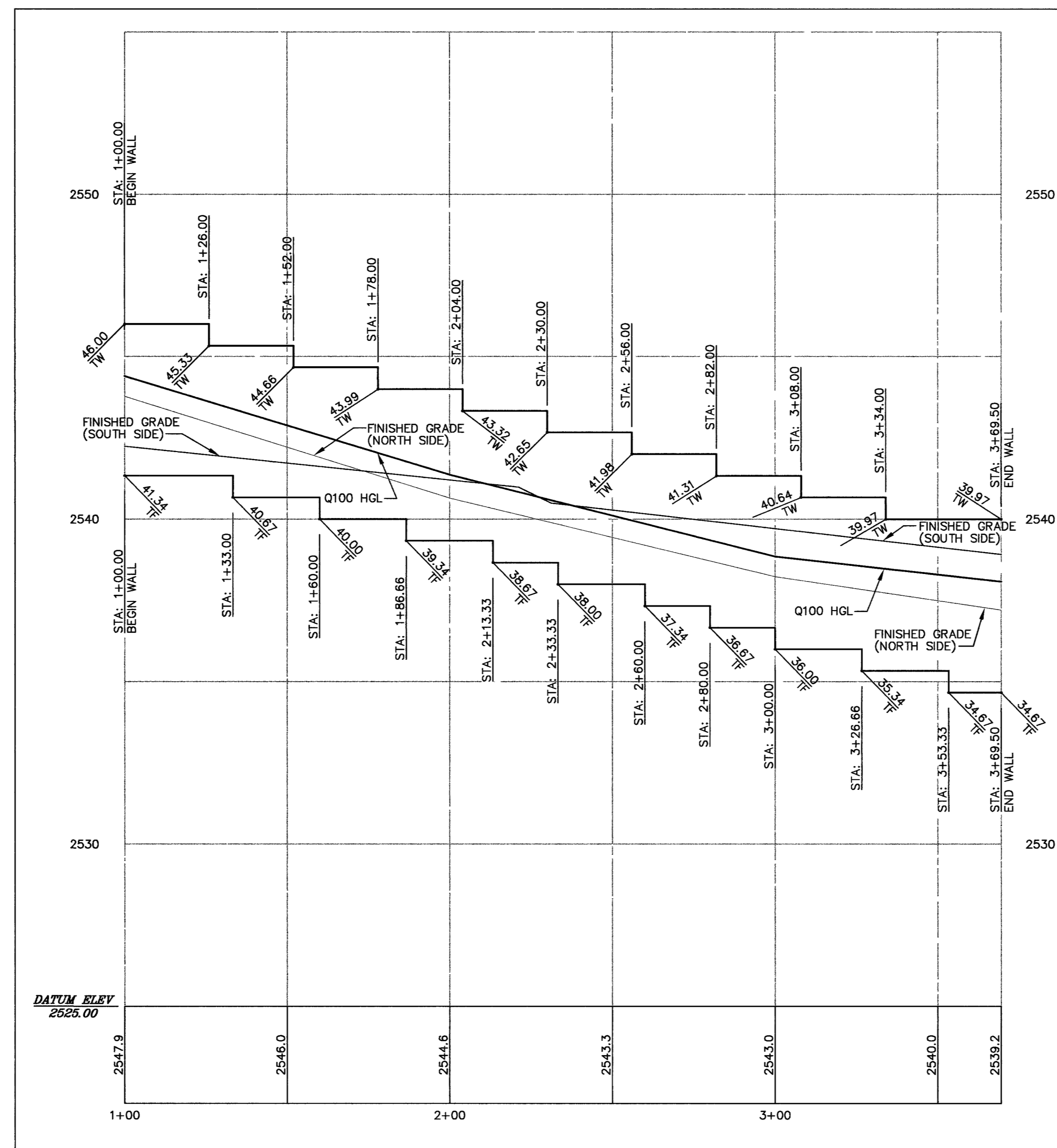
PROFILE VIEW SCALE: H-1"=50' V-1"=5'
