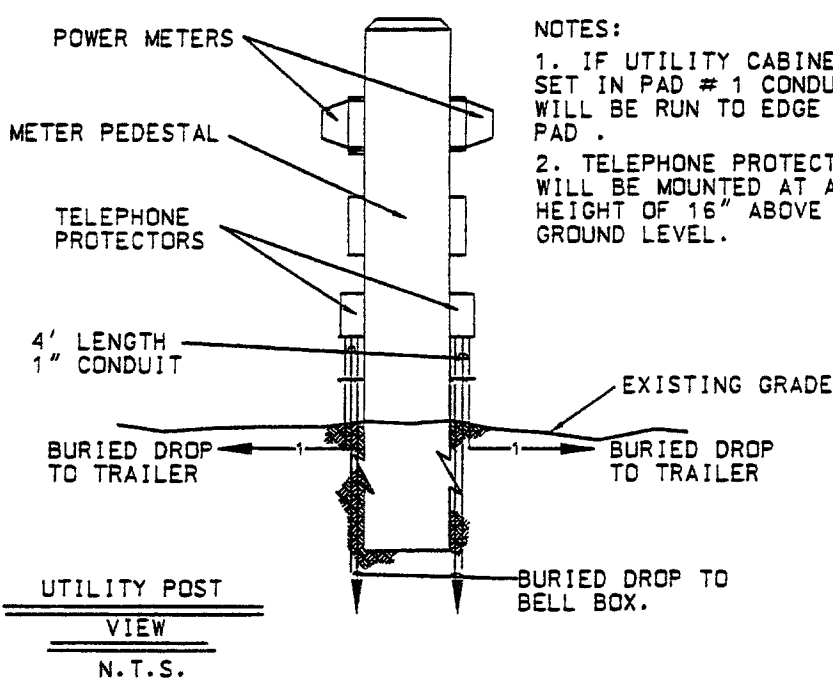
TRAILER PARK DETAIL (TYP.)
