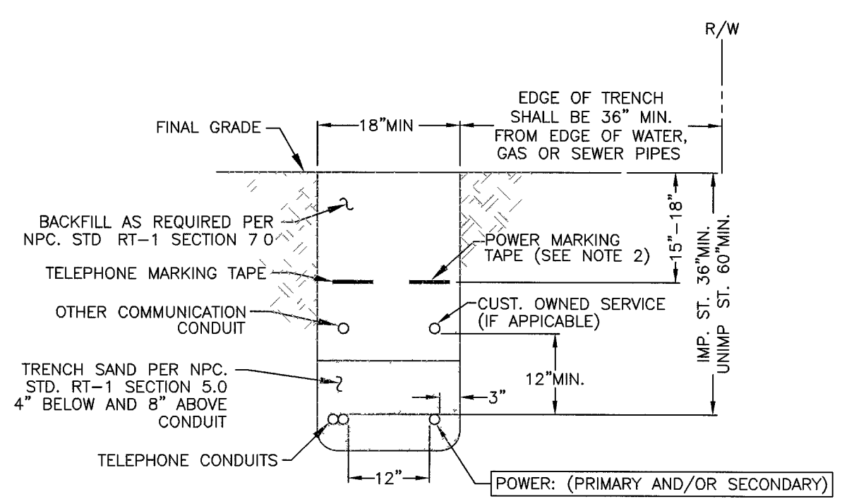
TRENCH DETAIL NPC U.G. STD. RT-12 (REV 4/8/02) (RESIDENTIAL AND COMMERCIAL)
