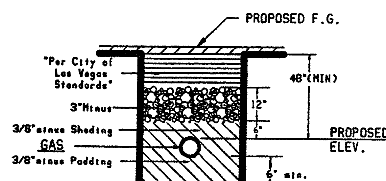
CLV TRENCH DETAIL FOR UNIMPROVED AREAS ONLY
